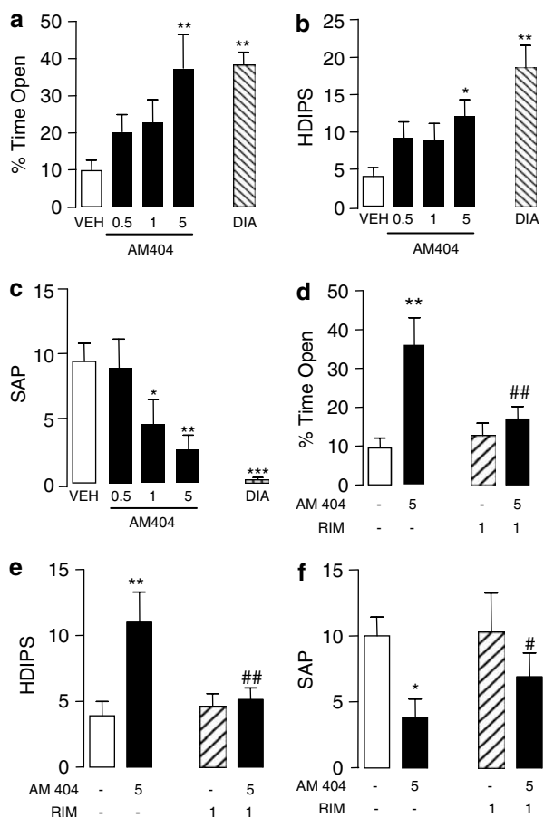
Figure 2 Effects of AM404 ( 0.5\text{--}5 \text{ mg kg}^{-1} , i.p.) or diazepam (DIA, 2.5 \text{ mg kg}^{-1} , i.p.) in the rat elevated plus maze test, and reversal of these effects by rimonabant (RIM). (a and d) AM404 and diazepam were injected 30 and 60 min before testing, respectively. Percent time spent in the open arms (%time open); (b and e) Number of head dips (HDIPS); (c and f) Number of stretched attend postures (SAP). * p < 0.05 , ** p < 0.01 compared to vehicle (VEH); *** p < 0.001 ; # p < 0.05 ; ## p < 0.01 compared to AM404 5 \text{ mg kg}^{-1} ; n = 8\text{--}11 per group.
