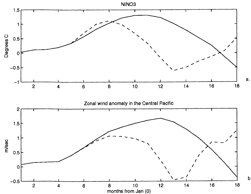
Figure 3. The evolution of a typical event for the modern solar forcing (solid line) and the mid-Holocene solar forcing in June–August and zero forcing during the rest of the year (dashed line). The two experiments have identical initial conditions and the first year and a half (starting in January (0)) are shown in (a) the NINO3 index and (b) the zonal wind field anomaly on the equator in the central Pacific ( 180^{\circ}\text{E} to 140^{\circ}\text{W} ) in \text{m s}^{-1} .
