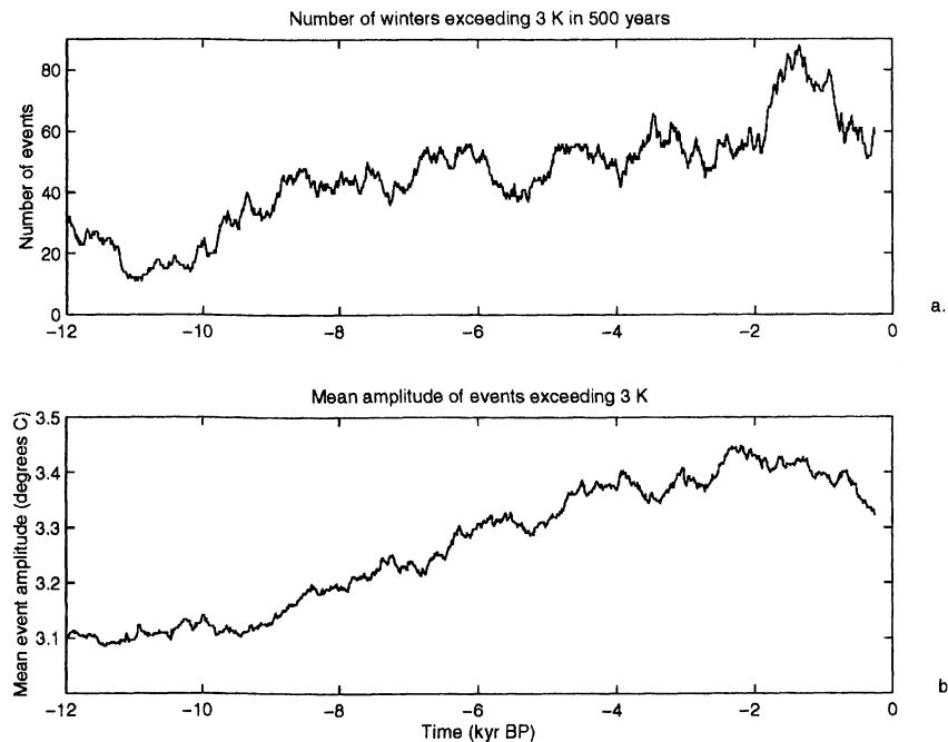
Figure 2. (a) The number of occurrences of events in 500 year overlapping windows (overlapping every 10 years) as a function of kiloyears B.P. An event is defined to occur when the mean December-February NINO3 SST anomaly exceeds 3 K. (b) The mean amplitude in the same overlapping 500 year windows of the events exceeding 3 K (in °C).
