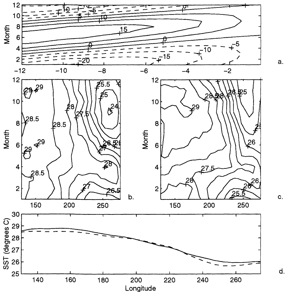
Figure 1. (a) Contour plot of the anomalous surface solar radiation on the equator ( W m^{-2} ) that is used to force the Zebiak-Cane coupled ocean-atmosphere model. The surface solar radiation is computed from the top of atmosphere values [Berger, 1978] assuming a fixed atmospheric transmissivity with a value of 0.7 meant to represent the bulk effect of absorption and reflection of solar radiation by all atmosphere constituents, and the solar zenith angle is also calculated as by Clement et al. [1999]. Values are plotted as a function of kiloyears before present (X axis) and month of the year (Y axis). The contour interval is 5 W m^{-2} . (b) Seasonal cycle of SST on the equator for the present climate as a function of month (Y axis). Note that this consists of both the background mean SST as well as the mean anomaly SST which is non zero due to the skewness of warm events (Zebiak and Cane, 1987). (c) Same as Figure 1b but with the anomalous seasonal cycle for the mid-Holocene (8-6 kyr) added to the present-day background seasonal cycle. (d) Annual mean SST along the equator for the present day (solid) and the mid-Holocene (dashed).
