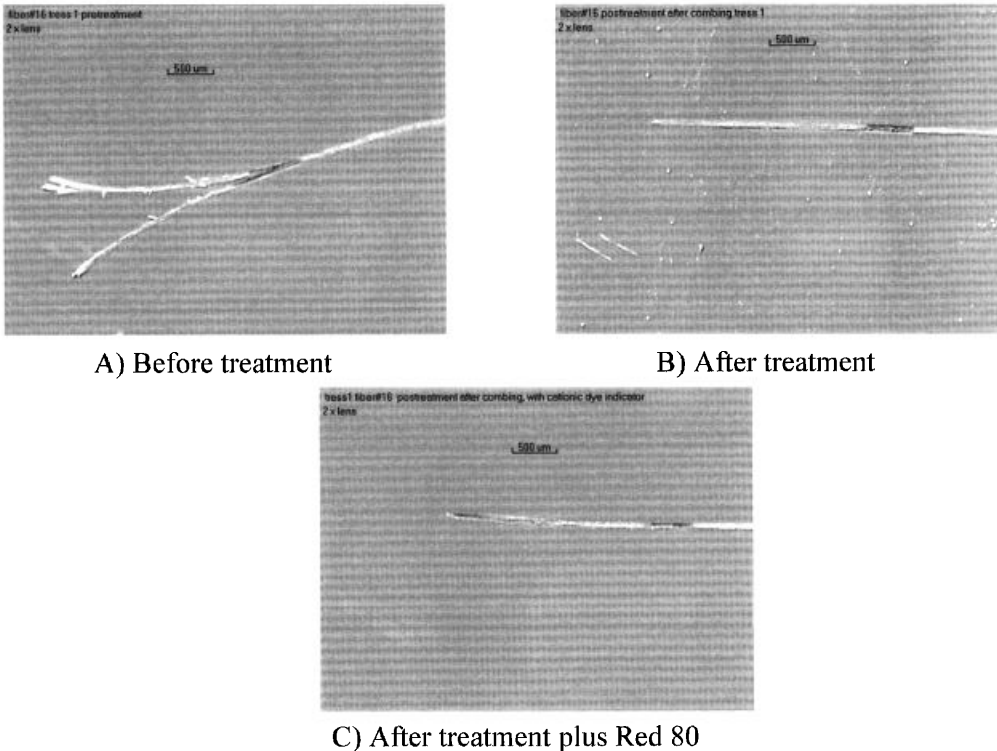
Figure 19. Anionic Direct Red 80 dye test indicates more microgel deposition on tip end.
