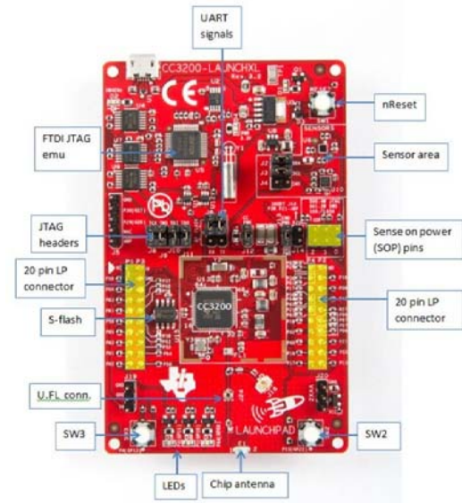
Fig. 1. TI CC3200 Launchpad board
