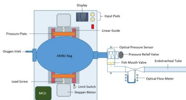
Fig -3: Schematic of Respiration Control Device (RC Device) [Courtesy Gyrodrive Machineries (P) Ltd.]
