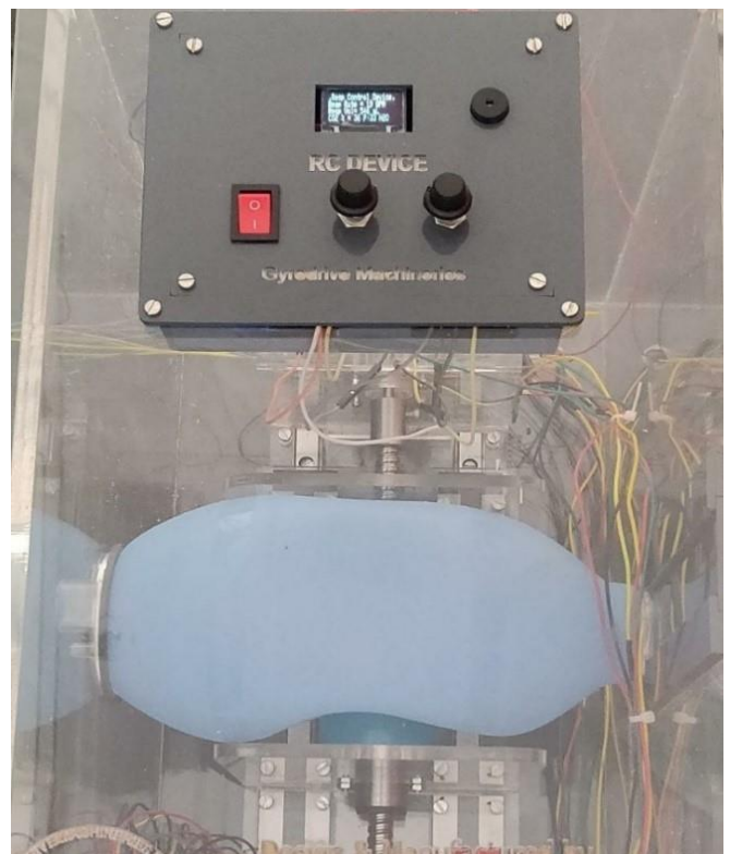
Fig -7: Second Working Prototype of RC Device [Courtesy Gyrodrive Machineries (P) Ltd.]
