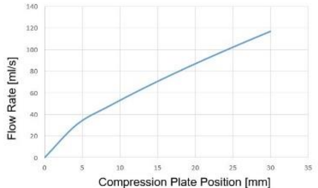
Fig -13: Plot of Air Flow Rate with Compression Plate Position
