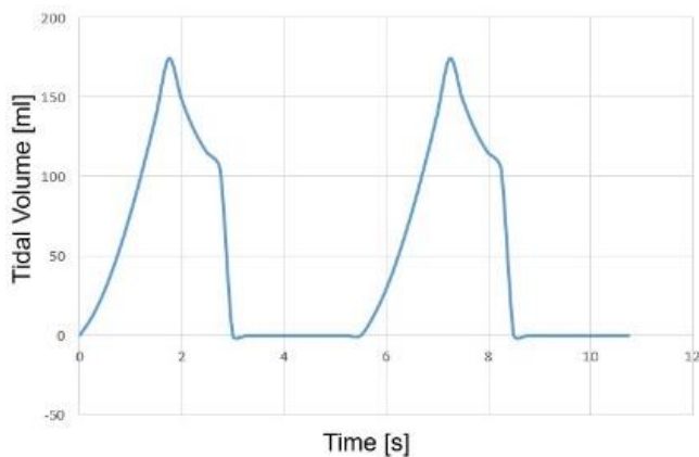
Fig -12: Plot for Tidal Volume with Time generated by Integration Flow Rate
