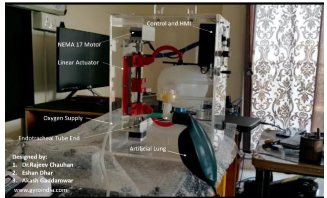
Fig -6: First Working Prototype of RC Device [Courtesy Gyrodrive Machineries (P) Ltd.]
