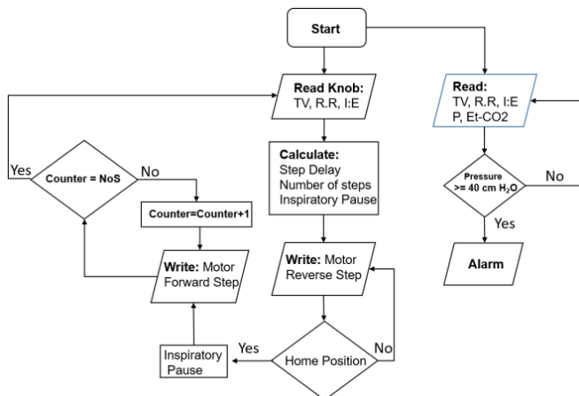
Fig -4: Basic Control Algorithm for RC Device [Courtesy Gyrodrive Machineries (P) Ltd.]
