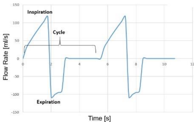
Fig -11: Plot of Air Flow Rate with Time for Two Breathing Cycles [Courtesy Gyrodrive Machinerics (P) Ltd.]
