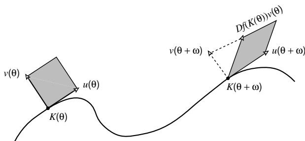
FIGURE 3. Geometric interpretation of the reason for automatic reducibility.
