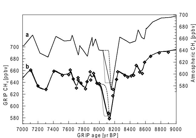
Figure 3. a) Possible Northern Hemisphere CH 4 variations shown as the scenarios S1 (solid black line), S2 (solid grey line) and S3 (dashed black line). b) Modelled CH 4 evolutions for the GRIP ice core assuming the three scenarios with the corresponding line styles. The thickness of the black line marks the range of solutions for S1. All model runs for GRIP lie within the 1\sigma uncertainty (10 ppbv) of the CH 4 measurements (diamonds) from Figure 1.
