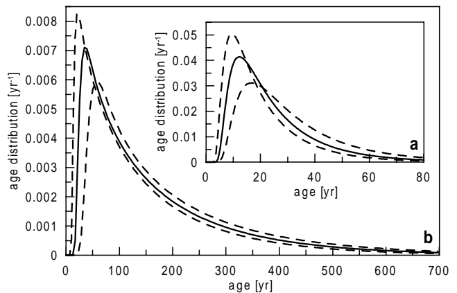
Figure 2. Modelled CH 4 age distribution for a) GRIP and b) Dome C at the depth where the air is completely enclosed in bubbles using the conditions during the 8.2 kyr BP event (Table 1). The solid line represents the best guess and the dashed lines the range of solutions. The age distributions are normalised to have an area of 1. Note the different scales in the two parts of the figure.
