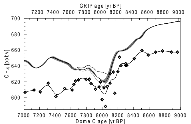
Figure 4. Comparison between the spline through the Dome C CH 4 data (bottom thick line and diamonds) from Figure 1 and the modelled CH 4 variations (three top lines) for the same core calculated from the assumed scenarios with the corresponding line styles (Figure 3). The shaded area marks the range of solutions for S1. The GRIP age scale has been displaced by 25 yr against the Dome C age in order to match the minimum of the spline trough the data and the modelled variation from S1.
