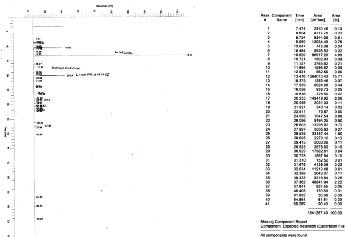
Fig. 2: Chromatogram of the essential oil of variety CIM Surabhi indicating the presence of high linalool content.
