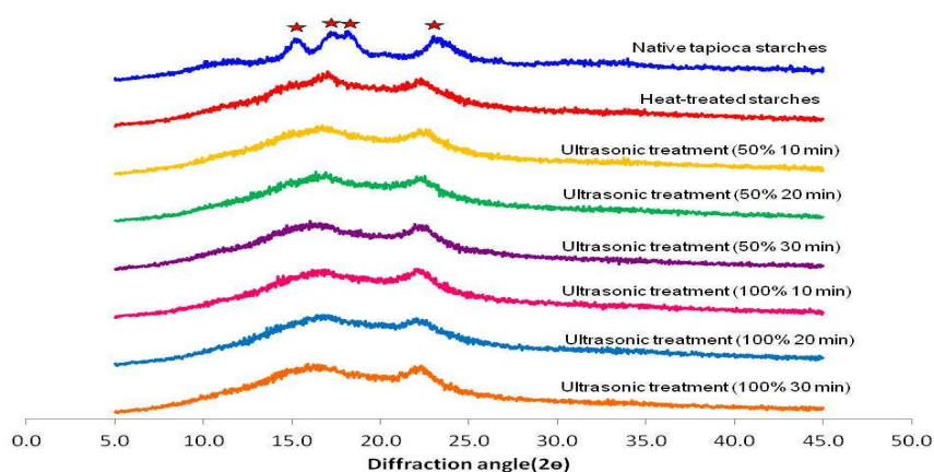
Figure 2. Powder x-ray diffractograms of native and modified tapioca starches.
