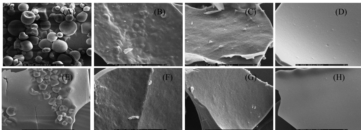
Figure 1. SEM images of the native and modified tapioca starches; (A) native, (B) heat-treated, ultrasonically treated with amplitude of 50% for (C) 10, (D) 20, (E) 30 min and ultrasonically treated with amplitude of 100% for (F) 10, (G) 20, (H) 30 min.
