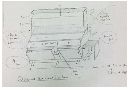
Fig. 3: Concept A – Automated Shoe Cabinet Lift with Foldable Bench.
