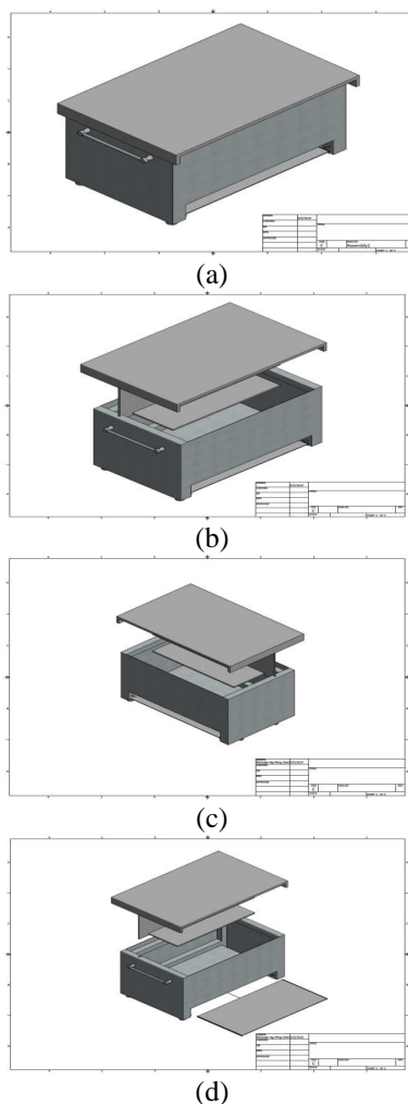
Fig. 5: CAD Drawings of Automated Shoe Storage Bench.
