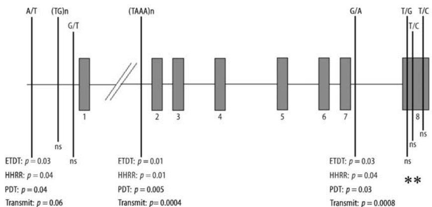
Fig. 1 Global significance values for eight common polymorphisms across SNAP-25 using four different methods for within family association analysis. * Indicate the two SNPs first described by Barr et al. [5]. Adapted from Mill et al. [121]
