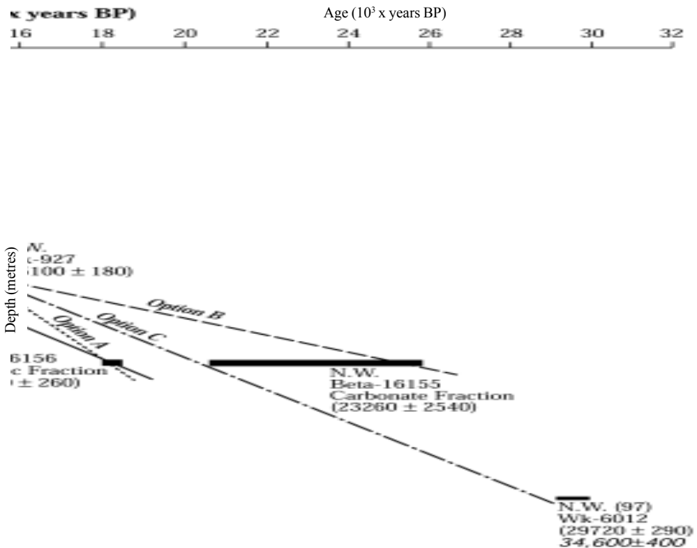
Fig. 3. Possible age-depth lines for sediment accumulation at sites from Tower Hill (modified from D'Costa et al. 1991)
