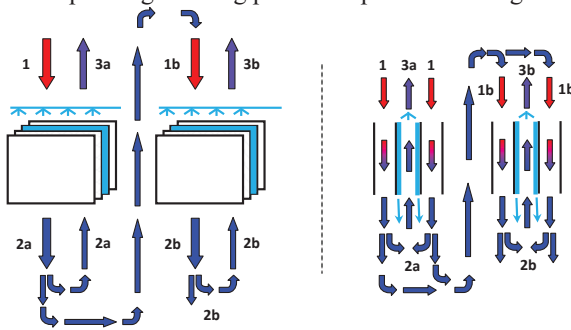
Fig. 7. Working principle scheme of D-IEC equipment; two stages R-IEC
