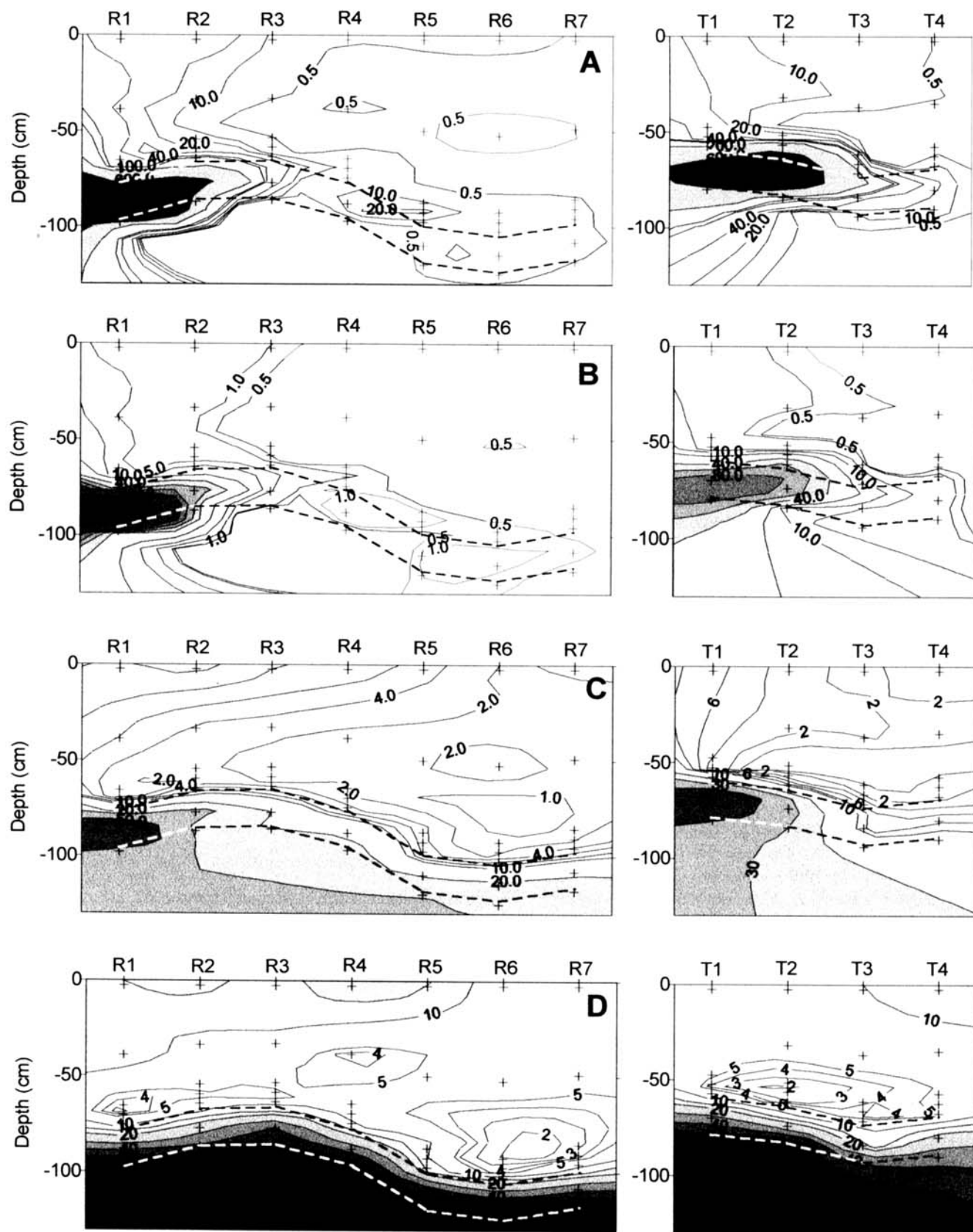
Fig. 3. a. Chl a , b. phaeo a , c. \text{NO}_3^- and d. \text{Si}(\text{OH})_4 spatial patterns along the two “coast to offshore” transects (R 1 to R 7 , 15/11/1995 and T 1 to T 4 , 26/11/1995). Pigment units: \text{mg m}^{-3} ; Nutrient units: \mu\text{M} (not normalized). Dashed lines indicate the PLI extent. Shading is proportional to concentration.
