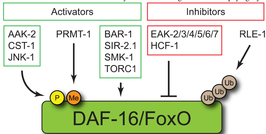
Figure 3. DAF-16/FoxO regulators and cofactors. DAF-16/FoxO is directly regulated by the serine/threonine kinases AAK-2, CST-1, and JNK-1, the arginine methyltransferase PRMT-1, and the E3 ubiquitin ligase RLE-1. The mechanistic basis for DAF-16/FoxO regulation by BAR-1, SIR-2.1, SMK-1, TORC1, the EAK proteins, and HCF-1 has not been established. See text for details.
