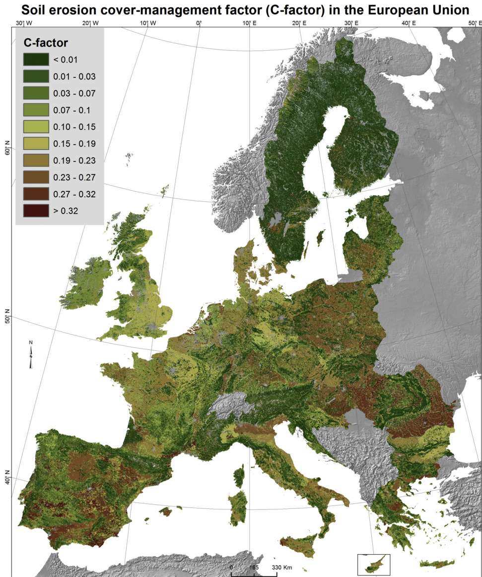
Fig. 3. C-factor map of the European Union.
