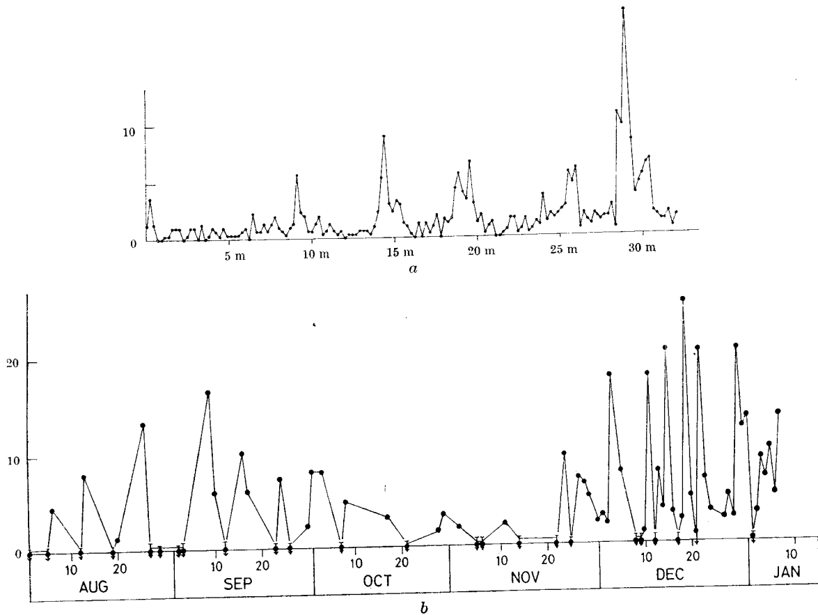
Fig. 2. a , The time variation of the smoothed (over ten pulses) pulse amplitude. b , Daily variation of peak pulse amplitude. (Ordinates are in units of W m^{-2} Hz^{-1} \times 10^{-16} .)
