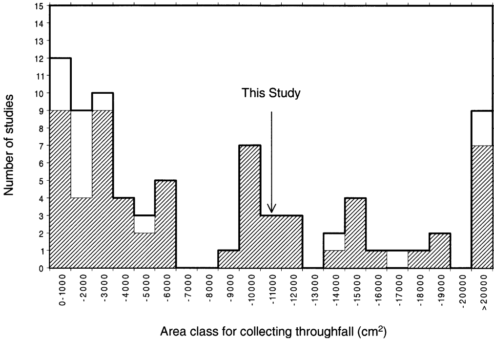
Fig. 8. Frequency distribution of total area for collecting throughfall in hydrological or ecological studies in tropical/subtropical forests all over the world (Number of studies, n = 77 ). Hatched area indicates the number of studies on natural forests or logged forests, while blank block means those on man-made forests. The total area of throughfall collector in this study are shown in the figure with an arrow. This figure are modified from KURAJI and TANAKA (2003).
