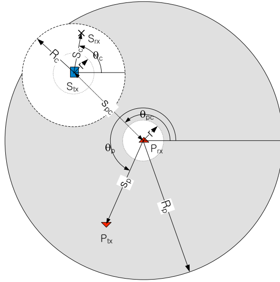
Fig. 1.5. Network configuration.
