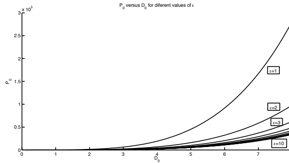
Fig. 1.10. Relationship between the primary transmit power P_0 and the exclusive region radius D_0 .
