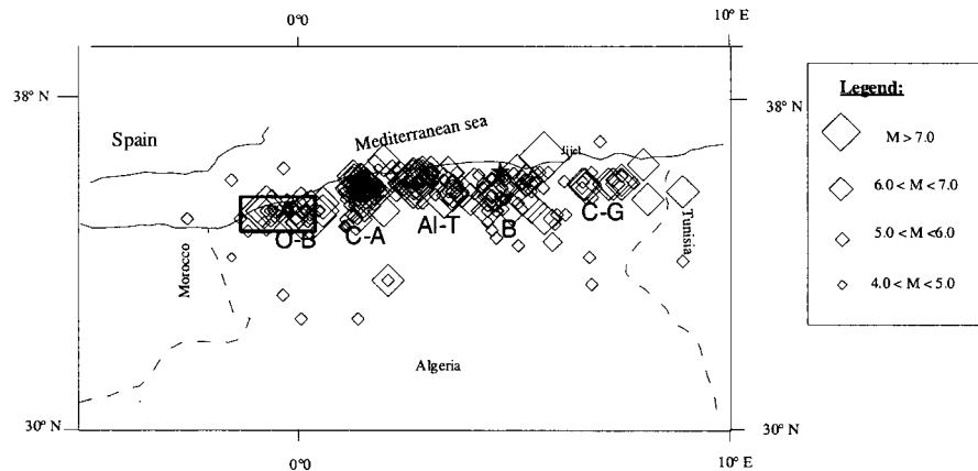
Figure 1. Seismicity map of the Tellean Atlas of Algeria for the period of 1365–1992. Location of epicentres are from historical seismicity catalogues of CRAAG, 1994 and Benouar, 1994. Areas of special concentration of epicentres are indicated by letters: O–B = Oran–Beni–Chougrane, C–A = Chlef–Ain Defla, Al–T = Algiers–Tipaza, B = Babor and C–G = Constantine–Guelma. The rectangle represents the studied area (see Figure 4).
