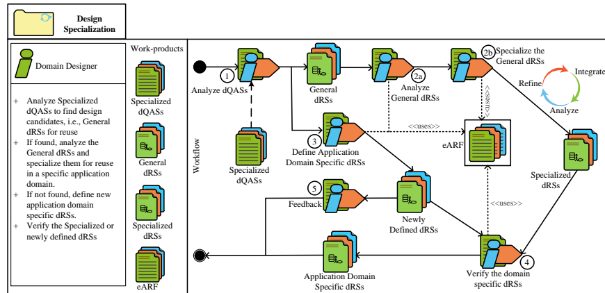
Figure 11: Design Specialization Process Package
