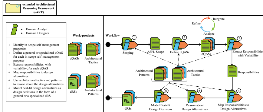
Figure 6: extended Architectural Reasoning Framework
