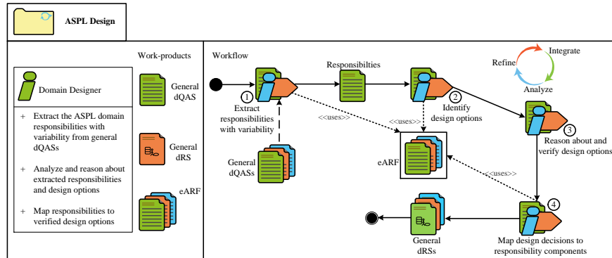
Figure 9: ASPL Design Process Package
