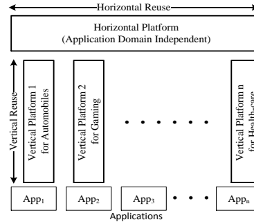
Figure 2: Horizontal and Vertical Reuse
