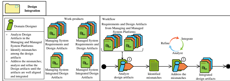
Figure 13: Design Integration Process Package
