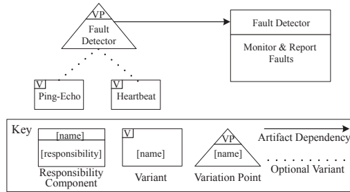
Figure 7: An excerpt from a dRS for Self-Healing
