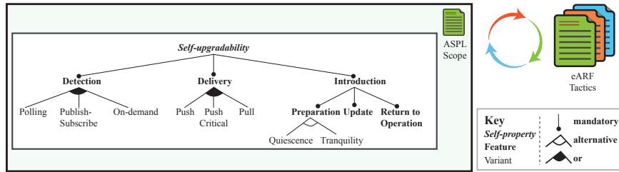
Figure 8: ASPL Scope Definition - Feature Model
