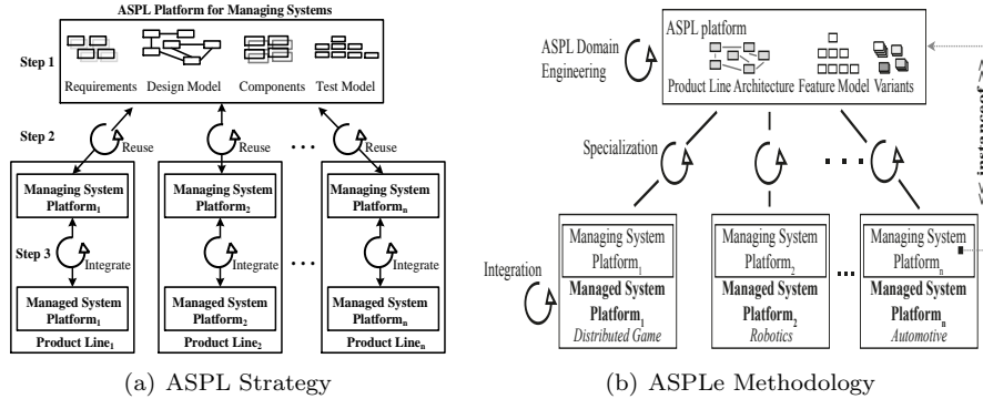
Figure 4: ASPL Strategy and ASPLe Methodology
