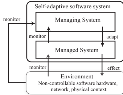
Figure 1: SASS - Conceptual Architecture
