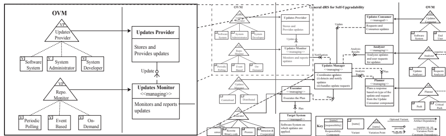
Figure 10: A General dRS for Self-Upgradability
