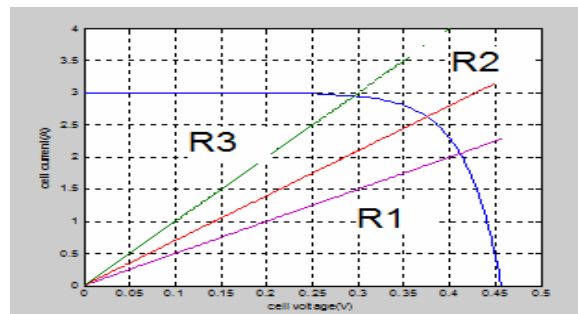
Figure 1. Variation of operating point with loads
