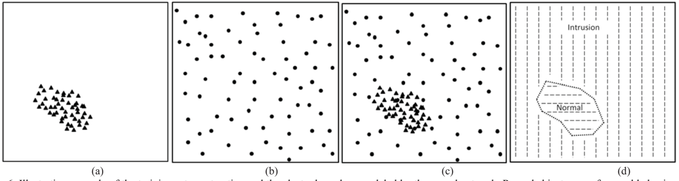
Fig. 6. Illustrative example of the training set construction and the cluster boundary modeled by the neural network. Recorded instances of normal behavior (a) and simulated intrusion instances (b) are combined together into a training set (c). The classification function and the cluster boundary (dotted line) is modeled by the neural network during the supervised learning process (d).
