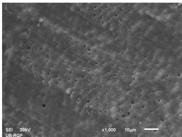
Figure 4. Representative microphotography of the apical third (chlorhexidine, intermittent protocol) (score 3) – SEM \times 1,000
