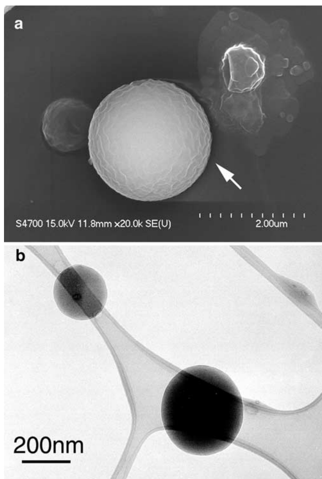
Figure 3. (a) Scanning electron microscope image of a tar ball (arrowed) in young smoke from the Medikwe Game Reserve fire, South Africa, on 20 August 2000; (b) TEM image of tar balls in aged smoke 16 km downwind from the Timbavati fire on 7 September 2000.
