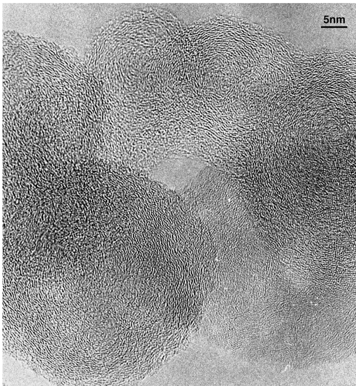
Figure 5. High-resolution TEM image of a soot aggregate in smoke from the Medikwe Game Reserve fire, South Africa, on 20 August 2000. The soot spheres show structures with onion-like curved, disordered graphitic (graphene) layers.
