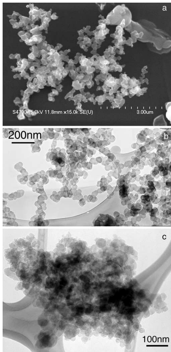
Figure 4. (a) Scanning electron microscope image of soot aggregates in young smoke from the Medikwe Game Reserve fire, South Africa, on 20 August 2000; (b) TEM image of chain-like soot aggregates in flaming smoke from the dambo fire near Kaoma, Zambia, on 5 September 2000; (c) TEM image of a compact soot aggregate in regional haze near Skukusa, South Africa, on 22 August 2000.
