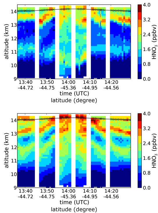
Figure 21. Comparison between a one-dimensional (top) and three-dimensional (bottom) reconstruction of \text{HNO}_3 during the GLORIA hexagonal flight. The segments of the hexagon are separated by white stripes. Measurement time (UTC) and latitude (degree) for the beginning of each segment are given on the x axis.
