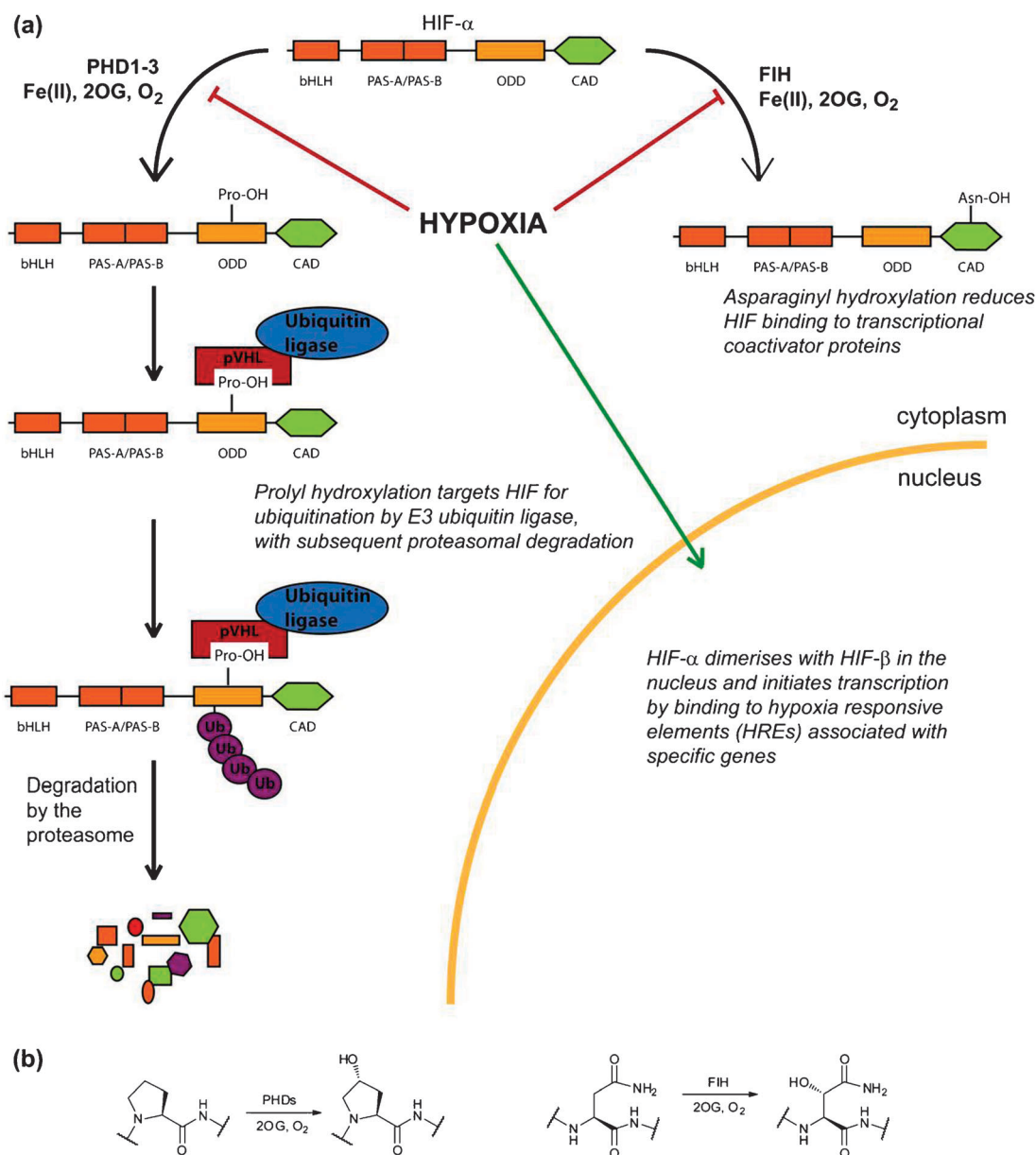
Fig. 12 The role of 2OG oxygenases in the hypoxic response in humans. (a) In humans, three PHD isoforms signal for HIF- \alpha degradation via the ubiquitin proteasome system by catalysing HIF- \alpha prolyl hydroxylation. FIH reduces the transcriptional activity of HIF by catalysing asparaginyl hydroxylation of its C-terminal transcriptional activation domain, a post-translational modification that reduces the interaction of HIF with transcriptional coactivator proteins. The bHLH (basic helix-loop-helix) and PAS domains of HIF- \alpha are involved in DNA binding and dimerisation with HIF- \beta . HIF- \alpha undergoes two prolyl-hydroxylations in its oxygen dependent degradation domain (ODD) and one in its C-terminal transcriptional activation domain (CAD). The von Hippel-Lindau Protein (pVHL) acts as a targeting component for an E3 ubiquitin ligase. (b) Prolyl and asparaginyl hydroxylation reactions catalysed by the PHDs and FIH.
