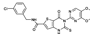
Fig. 14 Development of inhibitors of the HIF prolyl hydroxylases. (a) Variations on the glycinamide motif have been developed as inhibitors of PHD2. Selected compounds are shown; see ref. 238 for more detailed review. (b) Alternative metal chelation motifs have also been developed. Where applicable, selected patent applications associated with these compounds are given.
