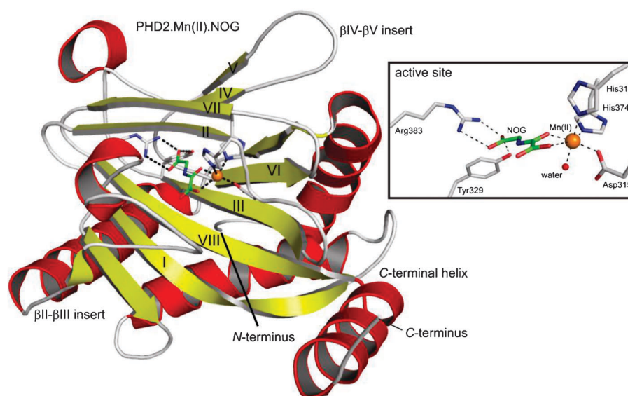
Fig. 1 General structural features of 2OG oxygenases. The view is derived from a crystal structure of the catalytic domain of the hypoxia inducible factor prolyl hydroxylase PHD2 (EGLN1) PDB ID 3HQR. The eight strands of the conserved double-stranded \beta -helix core fold are labelled I to VIII. Mn(II) and N -oxalylglycine (NOG) substitute for Fe(II) and 2OG respectively. The inset is a close-up of the active site showing the metal and 2OG binding residues.
