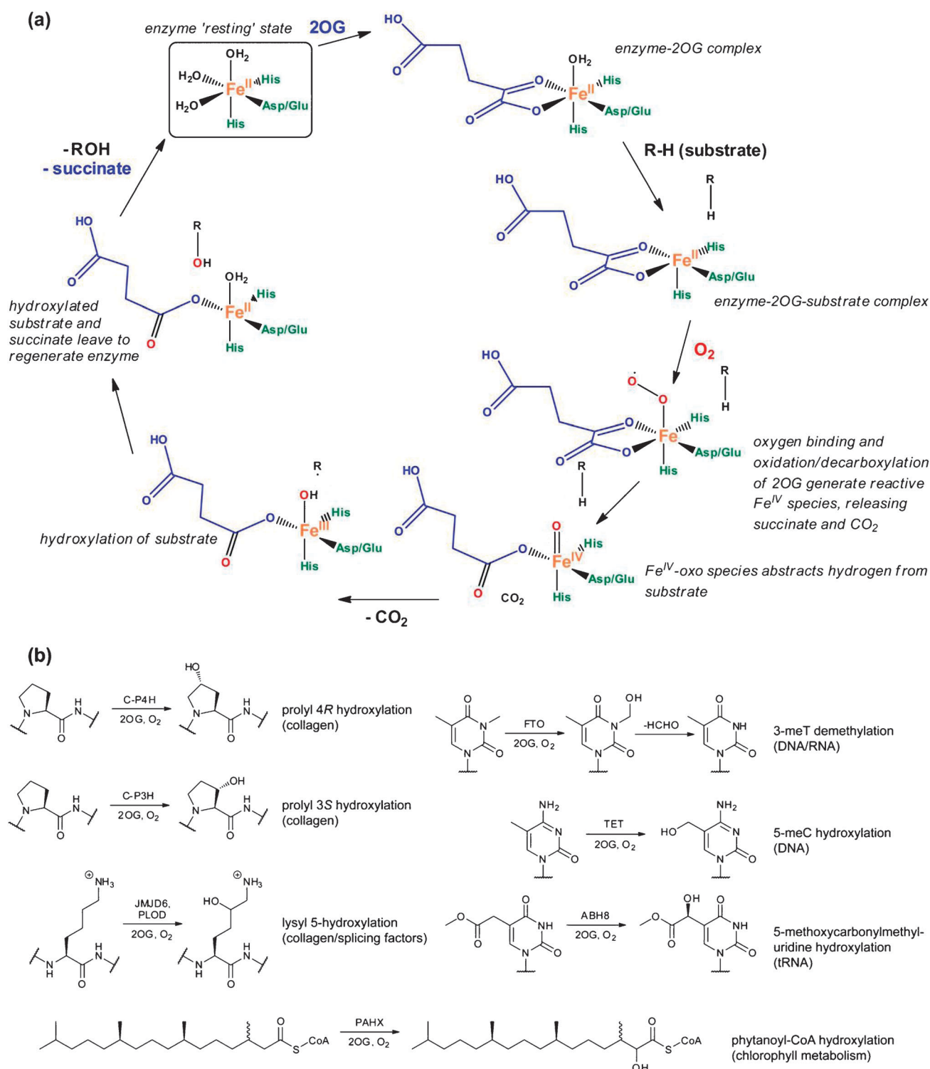
Fig. 2 Outline consensus mechanism for 2OG oxygenases and selected reactions catalysed by 2OG oxygenases. (a) There is evidence for all the intermediates shown, including the ferryl species, except for the O_2 complex and the Fe(III)-OH intermediate shown after reaction of the ferryl species. (b) Selected reactions catalysed by human 2OG oxygenases, showing the range of substrate types accepted by these enzymes. Other human 2OG oxygenase reactions are in Fig. 10, 12 and 15.
