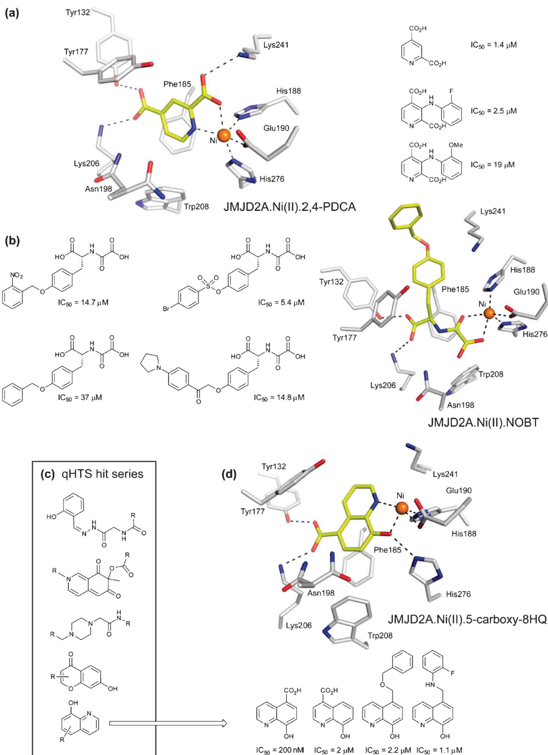
Fig. 16 Inhibitors of the JMJD2 histone demethylases. (a) View from a crystal structure of JMJD2A in complex with 2,4-PDCA (PDB ID 2VD7). The crystal structure indicates that substituents at the 3-position of 2,4-PDCA would be tolerated by the enzyme; 3-arylamino derivatives of 2,4-PDCA were shown to inhibit JMJD2 enzymes potently, but do not inhibit PHD2. (b) View from the crystal structure of JMJD2A in complex with N -oxalyl-D-( O -benzyl)tyrosine. Several other variations on the N -oxalyl-D-( O -benzyl)tyrosine scaffold are also good inhibitors of the JMJD2 demethylases, with sulfonate derivatives among the most potent. These inhibitors bind in the 2OG binding site but also block peptide substrate binding. (c) Selected compound classes identified as hit series from a high-throughput screen against the demethylase JMJD2E. (d) View from a crystal structure of JMJD2A in complex with the inhibitor 5-carboxy-8-hydroxyquinoline, identified through high-throughput screening, together with structures of several other potent inhibitors of the JMJD2 demethylases based on the 8-hydroxyquinoline template.
