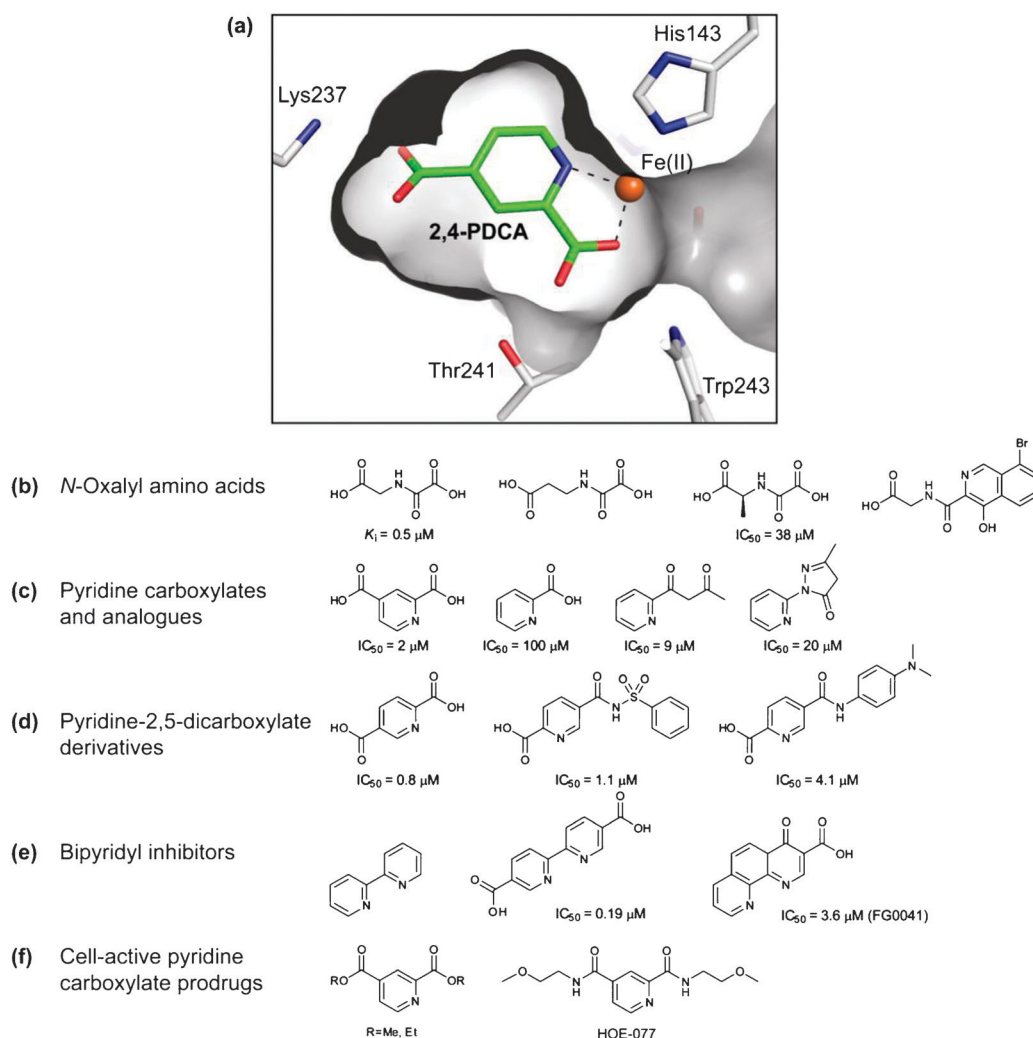
Fig. 7 Development of inhibitors of collagen prolyl-4-hydroxylase as potential antifibrotic agents. (a) View from a crystal structure of a collagen prolyl-4-hydroxylase (C-P4H) from C. reinhardtii in complex with 2,4-PDCA (PDB ID 2JIG), (b) N -oxalyl amino acid C-P4H inhibitors; while N -oxalylglycine and N -oxalyl-L-alanine were potent inhibitors, N -oxalyl- \beta -alanine was significantly less potent. Bicyclic analogues of N -oxalylglycine were also developed as inhibitors. (c) 2,4-Pyridinedicarboxylate and analogues of the 2-carboxylate were potent inhibitors, while pyridine-2-carboxylate (without the 4-carboxylate) was a weak inhibitor. (d) 2,5-PDCA was among the most potent C-P4H inhibitor characterised; a variety of substituents were tolerated at the C-5 carboxylate, suggesting an alternative mode of binding to that shown for 2,4 PDCA in (a) ( i.e. the C-5 carboxylate does not interact with Lys237, as observed for 2,4-PDCA). (e) Bipyridyl inhibitors of C-P4H. (f) Cell-active forms of 2,4-PDCA used in preclinical experiments. Reduction of hepatic fibrosis was achieved with HOE-077, but the mechanism of action may not be solely via inhibition of C-P4H.
