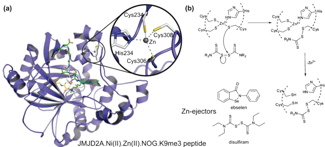
Fig. 17 Inhibition of the histone demethylase JMJD2A by ejection of structural Zn. (a) View from a crystal structure of JMJD2A in complex with H3K9me3 substrate peptide (PDB ID 2OQ6). Zn(II) is chelated by three cysteines and one histidine residue, and serves to hold together two loops of the enzyme. (b) The binding of Zn(II) is disrupted by ‘Zn-ejectors’ such as disulfiram and ebselen; a possible mechanism is shown here.
