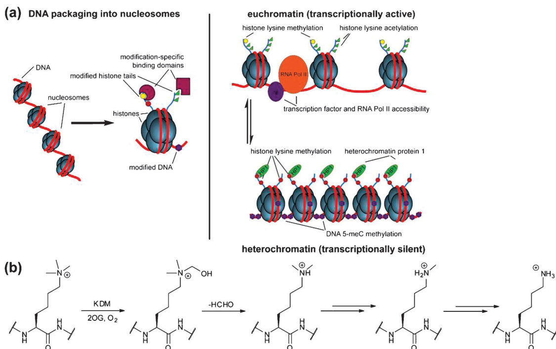
Fig. 15 Role of histone demethylases in chromatin modification. (a) Eukaryotic DNA is packaged into chromatin by formation of nucleosomes, which consist of eight histone proteins around which is wrapped ~146bp of DNA. Post-translational modifications of amino acid residues in the histone tails contribute to regulation of transcription by establishing euchromatin (transcriptionally active/accessible to RNA polymerase II) or heterochromatin (transcriptionally silent) states. 247 Note the figure is a simplification, many proteins are involved in transcriptional regulation. (b) The JmjC subfamily of 2OG oxygenases catalyse N ε -demethylation of all three N ε -methylated forms of histone lysine residues.
