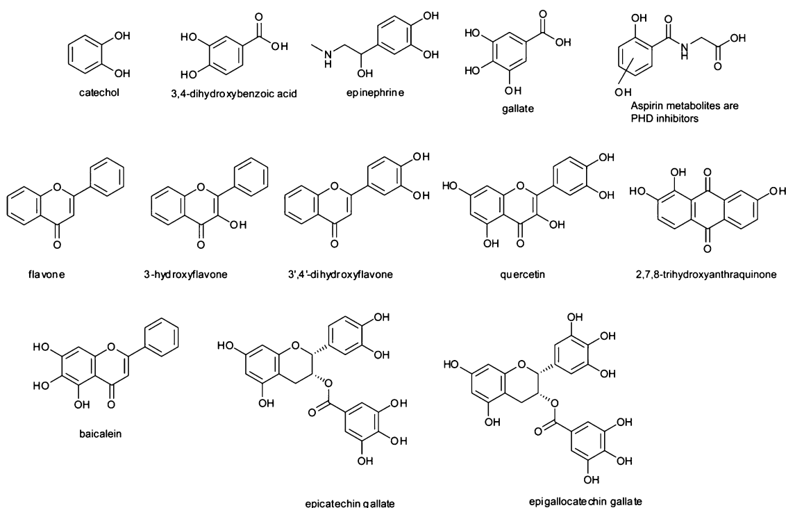
Fig. 6 Flavonoid inhibitors of 2OG oxygenases. Structures of flavonoids and other catechol type compounds observed to inhibit 2OG oxygenases.
