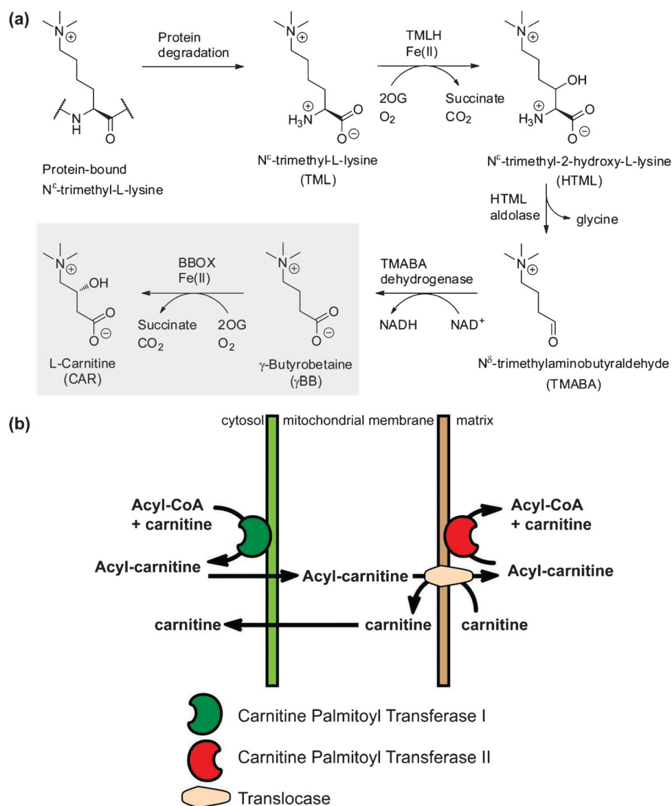
Fig. 10 Role of 2OG oxygenases in carnitine biosynthesis. (a) BBOX and TMLH catalyse steps in carnitine biosynthesis, and (b) function of carnitine/acyl-carnitine in transporting fatty acids across the mitochondrial membrane.
