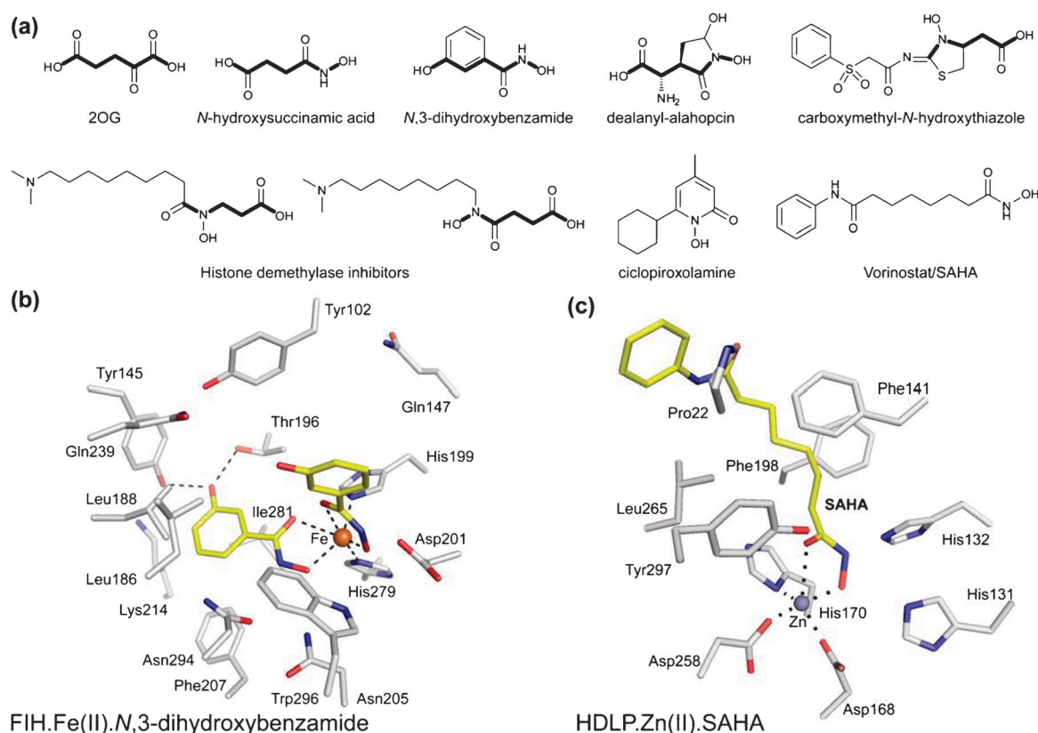
Fig. 4 Hydroxamic acids are inhibitors of 2OG oxygenases. (a) Structures of 2OG and of hydroxamic acids and related compounds reported to inhibit 2OG oxygenases. (b) View from the crystal structure of FIH in complex with 3-hydroxybenzamic acid (PDB ID 2WA4), which occupies the 2OG binding site and chelates the active site metal via the hydroxamic acid carbonyl and hydroxyl oxygens. Note that in this structure, another molecule of the hydroxamic acid was observed to bind, displacing the Fe-chelating residue Asp201, which forms part of the conserved HXD...H motif common to most 2OG oxygenases. (c) View from the crystal structure of Histone Deacetylase-Like Protein (HDLP) in complex with SAHA, the first hydroxamic acid HDAC inhibitor to be approved for clinical use (PDB ID 1C3S). As observed in (b), SAHA binds the active site Zn(II) ion through the carbonyl and hydroxyl oxygens of the hydroxamic acid moiety. SAHA has also been observed to inhibit the JMJD2 histone demethylase subfamily.
