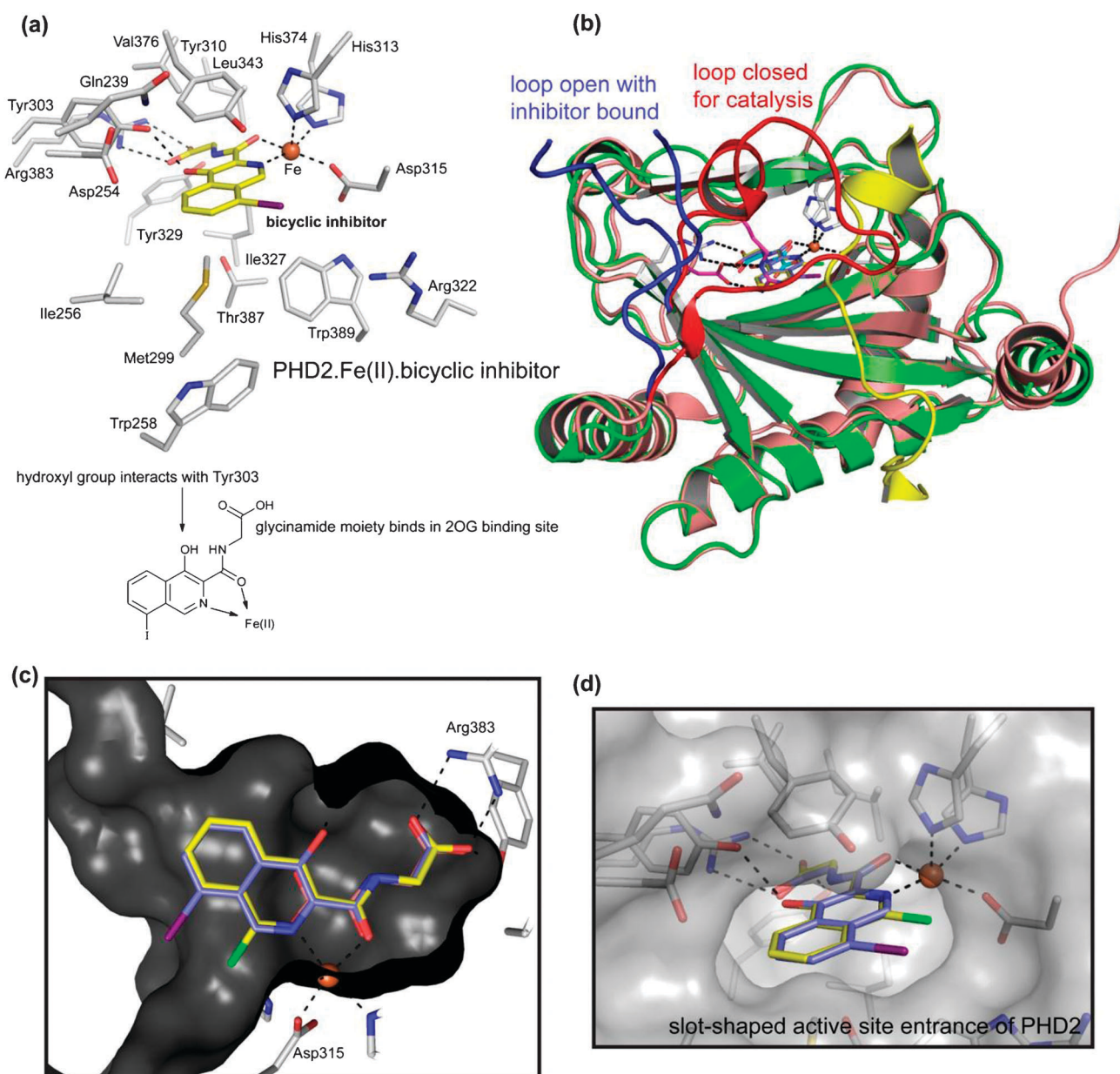
Fig. 13 Structures of the HIF prolyl hydroxylases complexed with inhibitors. (a) View from the crystal structure of PHD2 in complex with the bicyclic glycinamide 3-hydroxy-7-iodo-isoquinoliny-2-( N -glycyl)-carboxamide (PDB ID 2G19). (b) Views from crystal structures of PHD2 in complex with (i) a fragment of the HIF1- \alpha substrate and NOG (substrate in yellow, protein shown in pink), and (ii) with bicyclic inhibitor (with protein shown in green). A mobile loop (shown in red) folds to enclose the substrate peptide for active catalysis to occur. When the inhibitor is bound, the inhibitor prevents the closure of the loop by disrupting an intra-loop salt bridge (the loop in blue in this structure). (c) The glycinamide moiety (of both FG-2216 and the 7-iodo bicyclic inhibitor) binds in the 2OG binding site, forming a salt bridge with Arg383, while the 3-hydroxyl group hydrogen bonds with Tyr303. (d) The entrance to the active site of PHD2 in the inhibitor structures is relatively flat and 'slot-shaped,' and most of the reported potent inhibitors are relatively flat aromatic compounds that can fit into this 'slot.'
