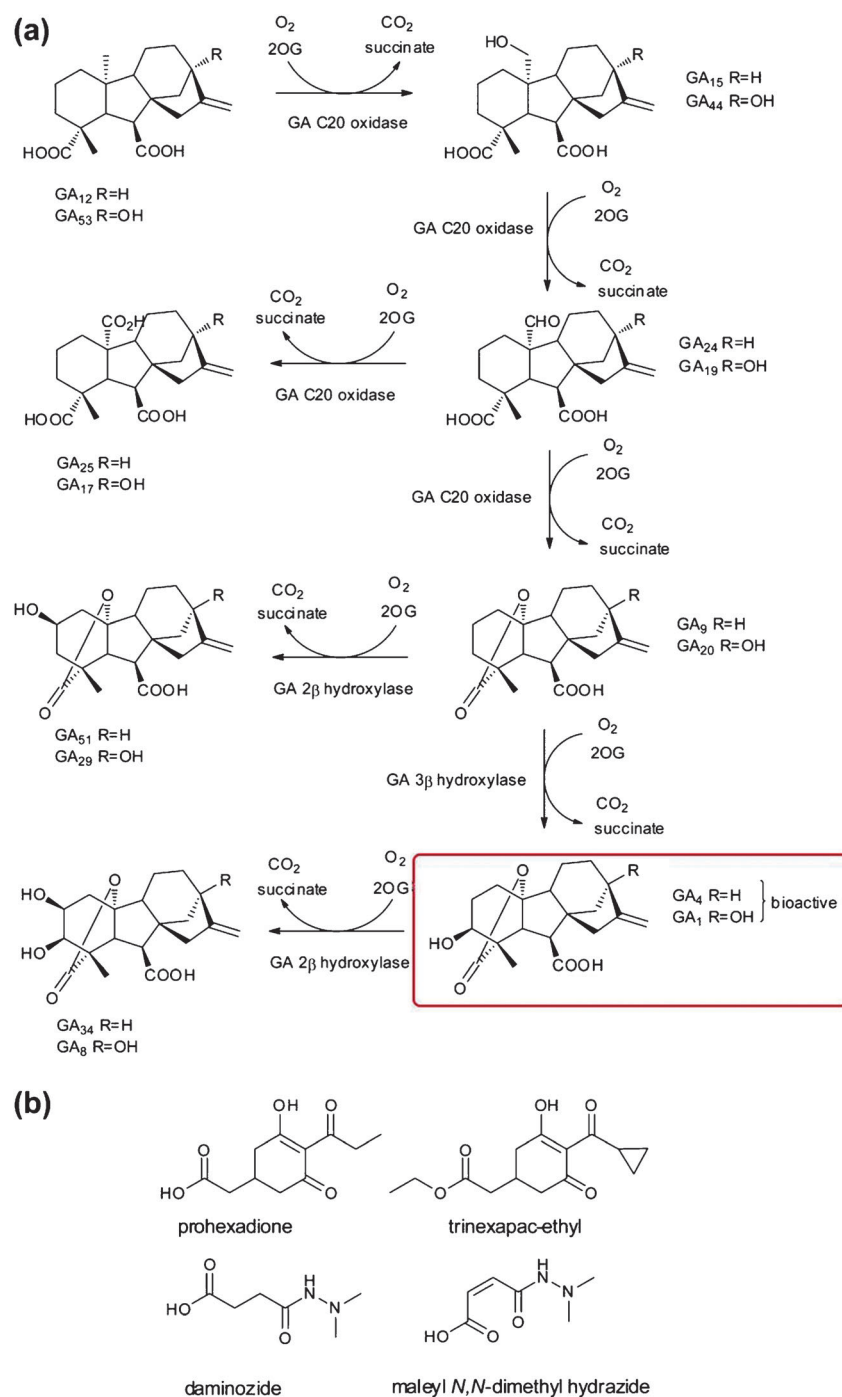
Fig. 8 Role of 2OG oxygenases in the biosynthesis of plant signalling molecules. (a) Steps in gibberellin synthesis. Starting with GA_{12} or its C-13 hydroxylated analogue GA_{53} , sequential oxidations at position C-20 lead to formation of alcohol ( GA_{15}/GA_{44} ) then aldehyde ( GA_{24}/GA_{19} ) intermediates before formation of either a carboxylic acid ( GA_{25}/GA_{17} ) or loss of C-20 and formation of a lactone bridge ( GA_9/GA_{20} ). Subsequent conversion to biologically active gibberellins is by the action of GA 3-oxidase/GA 3 \beta -hydroxylase enzymes. (b) Commercially used plant growth regulators.
