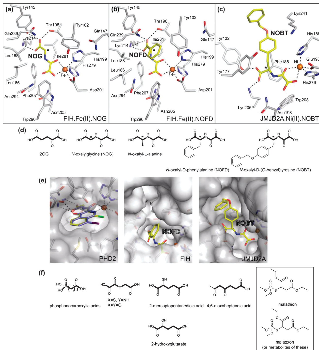
Fig. 3 N -Oxalyl amino acids are 'generic' inhibitors of 2OG oxygenases, binding in a similar mode to the 2OG cosubstrate. Differences in the 2OG and substrate binding pockets can be exploited for selective inhibition. (a) View from a crystal structure of FIH complexed with N -oxalylglycine (PDB ID 1H2K). (b) View from a crystal structure of FIH in complex with N -oxalyl- D -phenylalanine (PDB ID 1YCI), which inhibits FIH but not PHD2. (c) View from a crystal structure of JMJD2A in complex with NOBT ( N -oxalyl- D -( O -benzyl)tyrosine) which inhibits JMJD2A but not PHD2 (PDB ID 2WWJ). (d) Structures of 2OG and N -oxalyl amino acids. (e) Surface views from crystal structures of PHD2 (PDB IDs 2G1M overlaid with 3HQU), FIH (PDB ID 2HBV) and JMJD2A (PDB ID 2WWJ), demonstrating the size and shape of the active site and the scope for variation by designing N -oxalyl amino acids with suitable stereochemistry and substituents at the C- \alpha carbon (indicated with * in (a), (b) and (c)). Note that the size of the 2OG binding pocket/active site opening increases on going from PHD2 to FIH to JMJD2A. The PHD2 structure is an overlay of complexes with N -[(4-hydroxy-8-iodoisoquinolin-3-yl)carbonyl]glycine and N -[(1-chloro-4-hydroxyisoquinolin-3-yl)carbonyl]glycine. (f) Other acyclic analogues of 2OG reported as inhibitors (or precursors of inhibitors).
