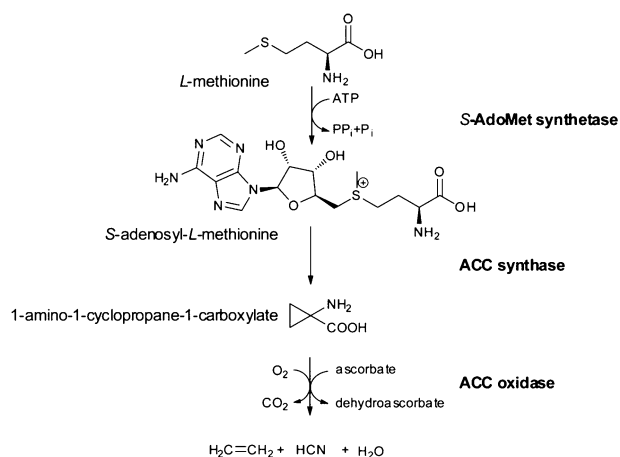
Fig. 9 Steps in the biosynthesis of ethylene. The final step is the ascorbate-dependent conversion of ACC to ethylene which also leads to formation of water and hydrogen cyanide. ACC oxidase activity is stimulated by bicarbonate/CO 2 .
