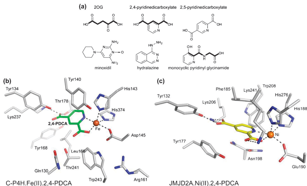
Fig. 5 Pyridine carboxylate inhibitors are simple cyclic analogues of 2OG. (a) Structures of 2OG, 2,4-pyridinedicarboxylate and 2,5-pyridinedicarboxylate, and of the related cyclic inhibitors minoxidil (which inhibits PLOD1), hydralazine (which inhibits C-P4H and the HIF PHDs) and a monocyclic pyridinyl glycinamide (an inhibitor of C-P4H and the HIF PHDs). (b) View from crystal structure of collagen prolyl-4-hydroxylase (C-P4H) from C. reinhardtii in complex with 2,4-PDCA (PDB ID 2JIG). Although 2,5-PDCA is reported to be a more potent inhibitor of C-P4H, 42 based on this crystal structure it may bind differently to the manner observed for 2,4-PDCA. (c) View from the crystal structure of the histone demethylase JMJD2A in complex with 2,4-PDCA (PDB ID 2VD7). 2,4-PDCA is positioned to form a salt bridge via its C-4-carboxylate with Lys206 (as does 2OG) and chelates the active site metal through the pyridinyl nitrogen and 2-carboxylate, but binds in a different plane to 2OG/NOG (compare PDB ID 2OQ6).
