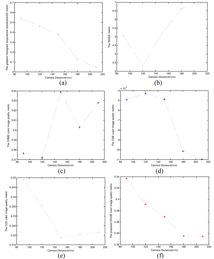
Fig. 8. Quality values of ColorChecker chart images (Fig.7). (a) R. (b) WGSA. (c) CRME. (d) CQE. (e) CIQI. (f) UCIQE.
