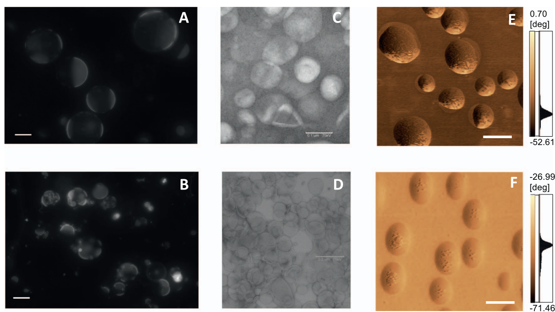
Fig. 6. Characterization of liposomes and proteoliposomes by different techniques. Fluorescence microscopy ( 60\times magnification, scales bar of 20 \mu\text{m} , labeled with 2% rhodamine) of (A) giant liposomes consisting of DOPC, CHOL and SM (8:1:1, molar ratio) and (B) 8:1:1 DOPC:CHOL:SM-giant liposomes harboring TNAP. Electron microscopy using negative staining of: (C) Liposomes consisting of DPPC (D) DPPC-proteoliposomes harboring TNAP, both with 50\times magnification. 3D topographic AFM images of (E) liposomes consisting of DPPC and DPPS (9:1, molar ratio) (xy area is 1\ \mu\text{m} \times 11\ \mu\text{m} and z axis from 0 to 84.50 nm) and scale bar of 250 nm and (F) 9:1 DPPC:DPPS-proteoliposomes harboring TNAP (xy area is 2.50\ \mu\text{m} \times 2.50\ \mu\text{m} and z axis from 0 to 40.81 nm) and scale bar of 250 nm.
