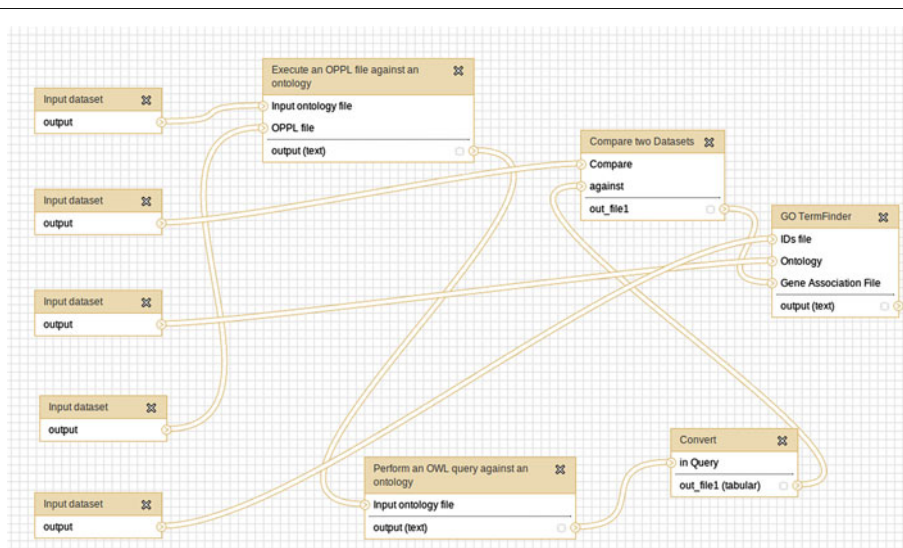
Figure 11 Selective extraction of modules from GO for term enrichment (as shown in Galaxy). In this workflow a reduced GAF is obtained by querying GO ( i.e. , extracting a module) and comparing the retrieved GO terms with the GO terms from the GAF. The resulting reduced GAF is used to perform an enrichment analysis with GO::TermFinder.
