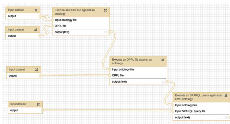
Figure 13 OWL TBox to ABox transformation for assisting SPARQL queries (as shown in Galaxy). In this workflow two OPPL scripts are used: the first one adds an instance to every class with the same URI and the second one adds an RDF triple for every existential restriction.
