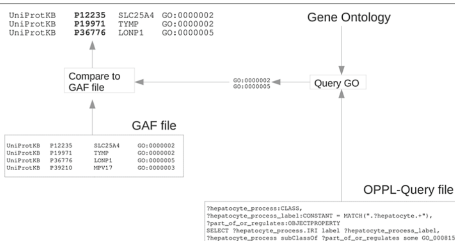
Figure 9 Complex querying of GO (details). Detailed depiction of the workflow shown in Figure 8.
