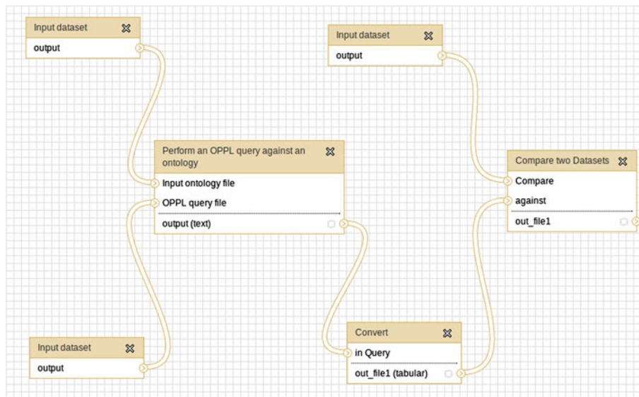
Figure 8 Complex querying of GO (as shown in Galaxy). OPPL-query workflow for querying GO against GAFs. The result is a list of proteins of interest.
