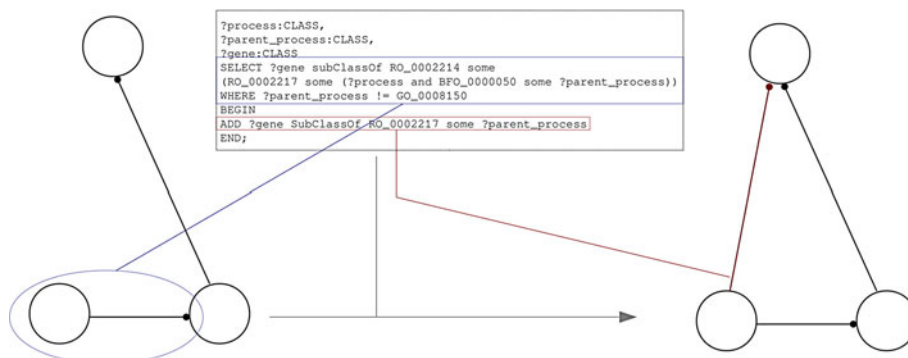
Figure 10 Expansion of gene product annotations through GO structure. This workflow starts from an OWL ontology that includes GAF information, produced by OORT. The script detects the structure ?gene subClassOf RO_0002214 some (RO_0002217 some (?process and BFO_0000050 some ?parent_process)) (Simplified depiction) and adds a new restriction to every matching class.
