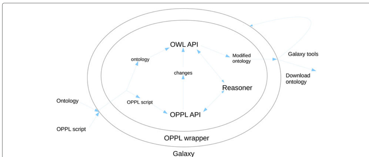
Figure 3 OPPL-Galaxy architecture. The inner circle represents the OPPL wrapper and the outer one Galaxy. Galaxy manages the data and parameters that will be passed to the OPPL wrapper. In order to pass, for instance, an ontology to the OPPL wrapper, the ontology must be first uploaded to Galaxy (or passed to it from the output of another Galaxy tool). Also, Galaxy manages the output of the OPPL wrapper: it can be redirected to other Galaxy tools or downloaded and saved as a standalone file. The OPPL wrapper coordinates the OPPL API (to parse the OPPL script and execute it), the OWL API (to read/write ontologies from stdin to stdout and perform changes), and the chosen reasoner (to perform inferences).
