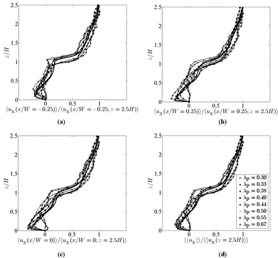
FIG. 6. Vertical mean velocity profiles in the broader street canyon normalized over the mean velocity at the height z/H = 2.5 . Showing profiles at 3 different horizontal positions: (a) x/W = -0.25 , (b) x/W = +0.25 , and (c) x/W = 0 ; along with (d) average vertical mean velocity profiles, averaged over the three horizontal positions shown in (a)–(c) and depicted at the half-width.
