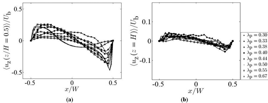
FIG. 12. (a) Horizontal profiles of the vertical velocity at the mid-height level of the modelled street-canyon, for all tested geometric packing densities. (b) Horizontal profiles of the vertical velocity at the rooftop of the modelled street-canyon, for all tested geometric packing densities.
