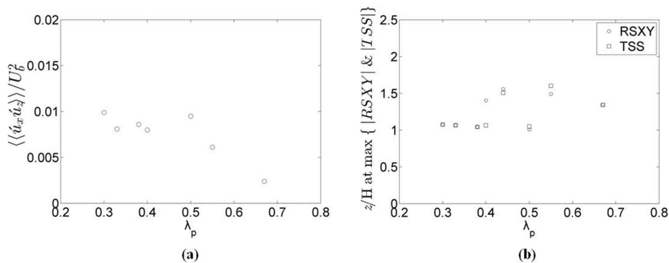
FIG. 9. (a) Averaged Reynolds stress RS_{xy} at the rooftop level ( z/H = 1 ) over the entire horizontal span, for the different geometries/packing densities. (b) Normalized height at which maximum stress occurs for each packing density geometry, using as indicator the Reynolds stress maximum (denoted as RS_{XY} ) and the total shear stress (denoted as TSS ).
