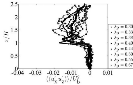
FIG. 8. Vertical Reynolds stress profiles, averaged over the horizontal positions at x/W = -0.25, 0, and +0.25 .
