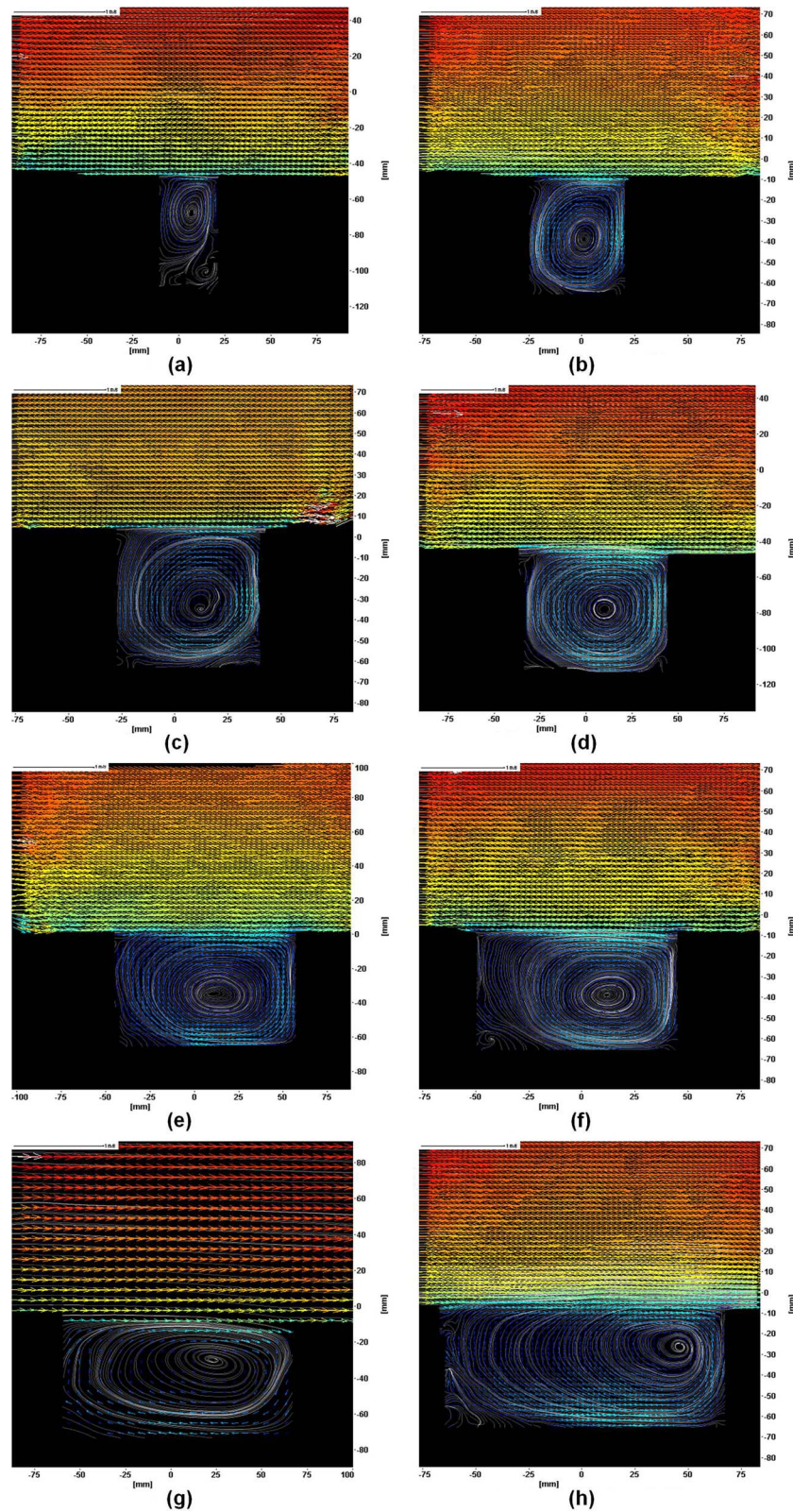
FIG. 4. The flow velocity fields and streamlines obtained using PIV measurements in the range of test cases conducted. (a) Case 1: \lambda_p = 0.67 ; (b) Case 2: \lambda_p = 0.55 ; (c) Case 3: \lambda_p = 0.50 ; (d) Case 4: \lambda_p = 0.44 ; (e) Case 5: \lambda_p = 0.40 ; (f) Case 6: \lambda_p = 0.38 ; (g) Case 7: \lambda_p = 0.33 ; (h) Case 8: \lambda_p = 0.30 .
