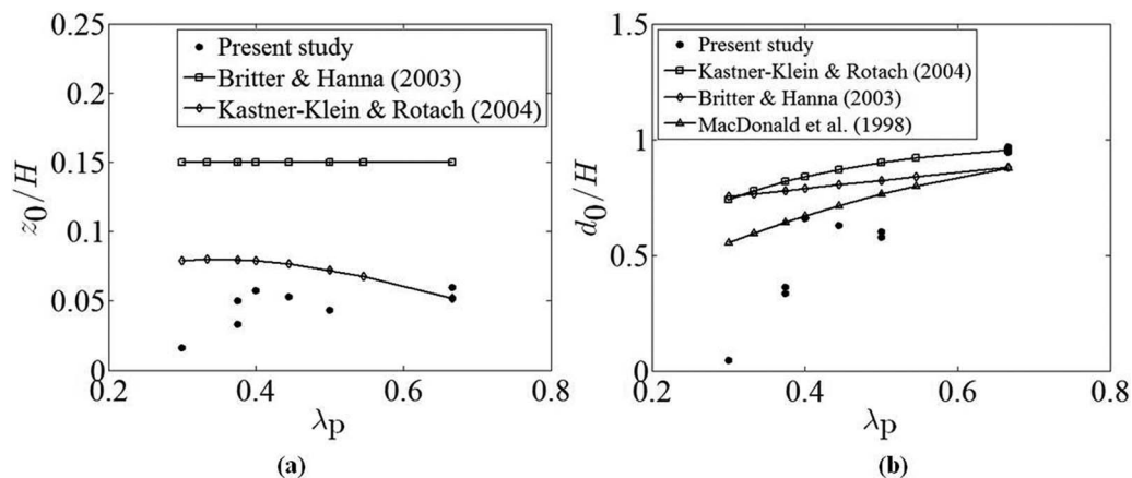
FIG. 11. (a) The deduced variation of the surface roughness length z_0 with the geometric packing density. (b) Variation of the zero-plane displacement thickness/height d_0 with the geometric packing density, for the idealized, homogeneous 2D rectangular-canyon-like roughness elements and contextual comparison with: the heterogeneous canyon case in a modelled real urban area under controlled laboratory conditions by Kastner-Klein et al. ; 23 the case of real field data (including natural wind variability) using morphometric methods by Britter and Hanna; 7 the homogeneous cubical building arrays by MacDonald 51 for the zero-plane displacement height d_0 .
