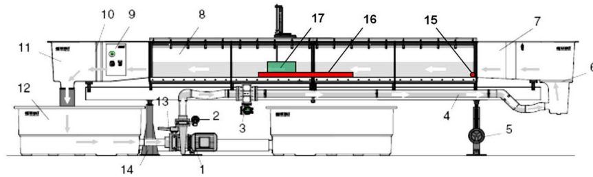
FIG. 1. Water flow channel apparatus: (1) centrifugal pump; (2) shut-off valve hand wheel for flow rate regulation; (3) flow rate meter; (4) pressure line; (5) incline adjustment facility; (6) flow rectifier; (7) intake flow preparation section; (8) modular centre element; (9) switch box; (10) overflow sensor; (11) outflow element; (12) tank; (13) shut-off valve; (14) fixed bearing; (15) trip wire; (16) urban canopy model; and (17) measurement area.
