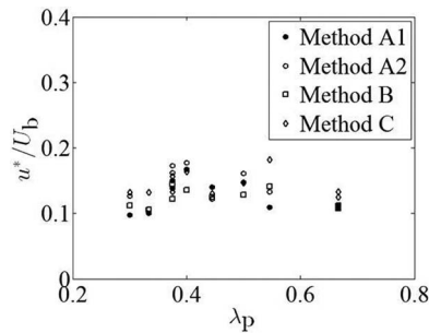
FIG. 10. Variation of the friction velocity deduced from the PIV measurements with the packing density of urban geometry. Method A1: from U = f(\ln(y)) gradient with d_0 imposed from Kastner-Klein and Rotach. 23 Method A2: from U = f(\ln(y)) intercept “2” with z_0 imposed from Kastner-Klein and Rotach. 23 Method B: from \max\{|RS_{xz}^{1/2}|\} = \max\{|\langle u'_x u'_z \rangle|^{1/2}\} . Method C: from maximum total shear stress as \max\{|TSS_{\max}|^{1/2}\} .
