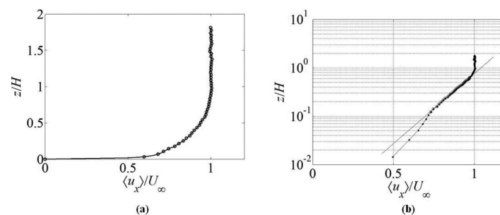
FIG. 3. Measured boundary layer profile upstream of the urban canopy/geometry model in: (a) linear and (b) semi-logarithmic axes.
