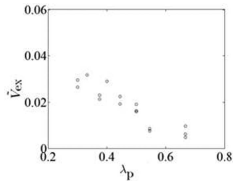
FIG. 13. Variation of the non-dimensional exchange velocity ( V_{ex} ) (normalized with respect to U_b ) with the geometric packing density.
