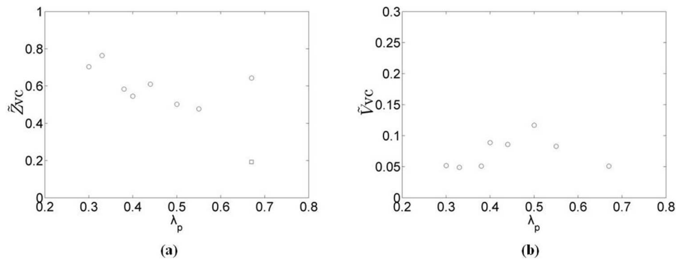
FIG. 5. (a) The dimensionless (with respect to H ) vertical position ( Z_{vc} ) of the internal canyon recirculation cell core. (b) The dimensionless (with respect to U_b and W ) net bulk flux ( V_{vc} ), evaluated from Eq. (8).
