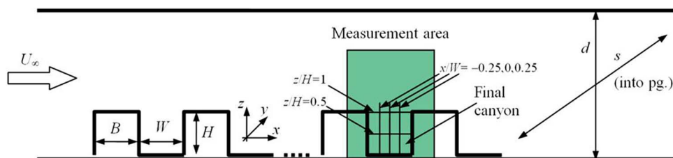
FIG. 2. Urban canopy-geometry model.
