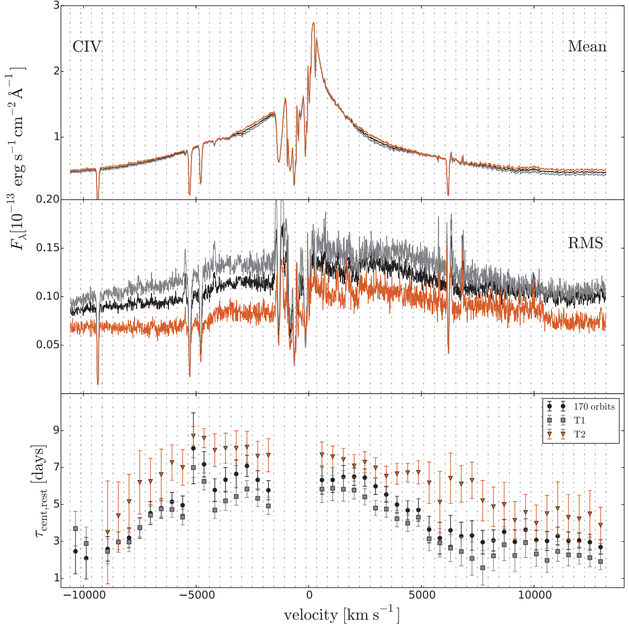
Figure 5. Velocity-binned results for the CIV \lambda 1549 emission line. The top and middle panels show the mean and RMS spectra, respectively. The bottom panel shows the centroid of the cross-correlation function for each individual velocity bin, corrected to the rest frame of NGC 5548. Velocity bins with no lag measurement contain too little total flux to reliably characterize the variations. In each case, the black line represents the entire dataset, and the T1 (first 85 visits) and T2 (last 85 visits) subsets are shown in gray and orange, respectively. Note that the shortest lags are found for the highest-velocity gas.
