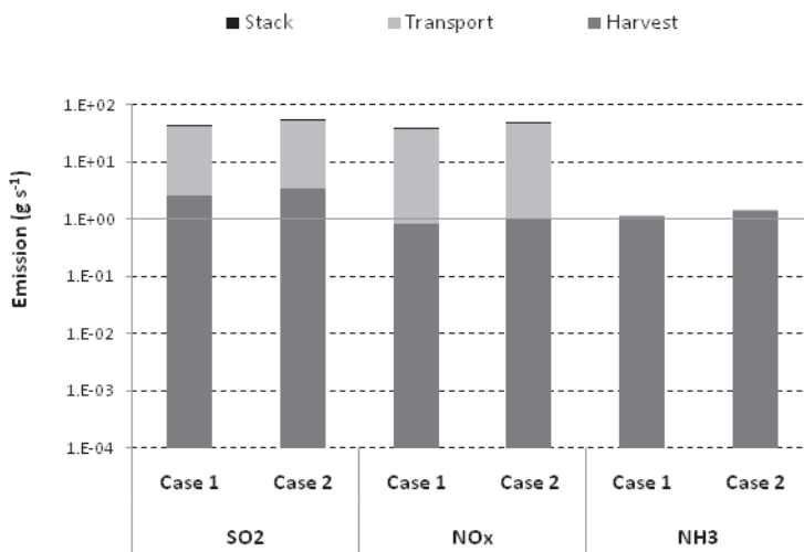
Figure 2: Emission inventory generated for the constituent activities on a life cycle of a CHP system.
