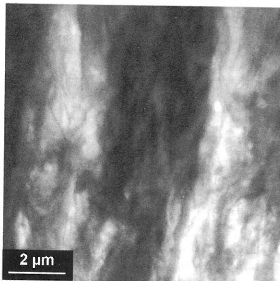
Figure 6 - TEM images of nickel layers deposited from the sulfamate bath with 4g/L (30 oz/gal) of 1,3,6 naphthalene trisulfonic acid at two current densities. Right image: i = 0.5 \text{ A/dm}^2 (4.6 A/ft 2 ). Left image: i = 20 \text{ A/dm}^2 (186 A/ft 2 ).
