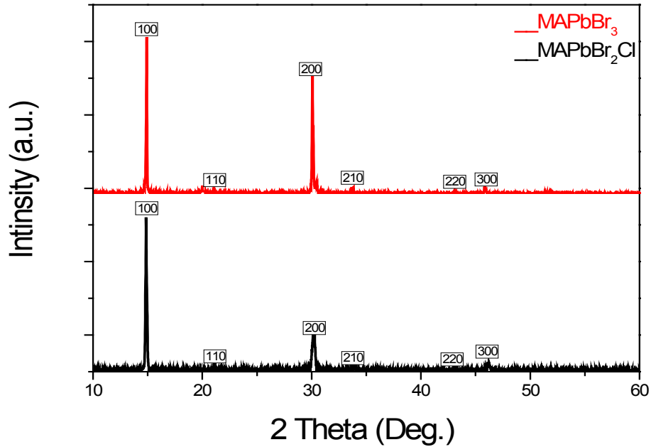
Figure 1. XRD pattern for the MAPbBr 3 and MAPbBr 2 Cl perovskites
