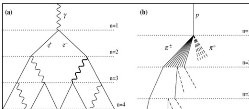
Figure 1. Schematic views of (a) Electromagnetic cascade and (b) Hadronic shower[7].
