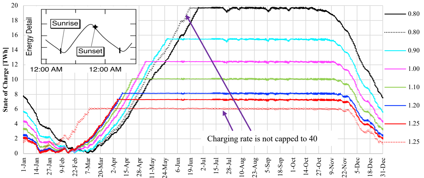
Fig. 1. Calculated state of charge for stored energy using 2019 generation and load data adjusted to reflect zero-carbon grid scenarios with variable solar. Each curve reflects a different annual solar-generation-to-load ratio (see legend). The charging rate was capped at 40 GW for all except for the 2 dotted lines.
