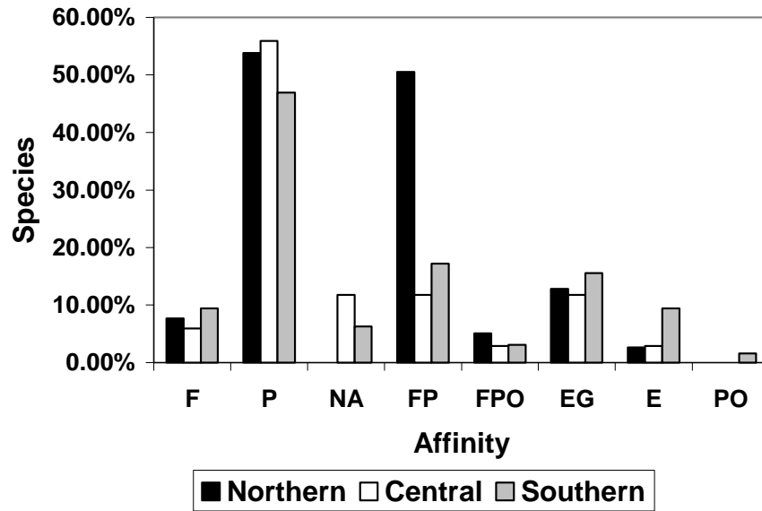
Figure 6: The affinity and faunal composition of the three geomorphological parts in Sinai. E: Endemic to Sinai; EG: Endemic to Egypt; F: Afrotropical; FOP: Afrotropico-Palaeartico-Orienta; FP: Afrotropico-Palaeartico; NA: confined to North Africa only; P: Palaeartico; PO: Palaeartico-Oriental
