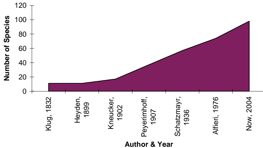
Fig. 1: Summary of carabid diversity in Sinai recorded from 1832 to 2004
