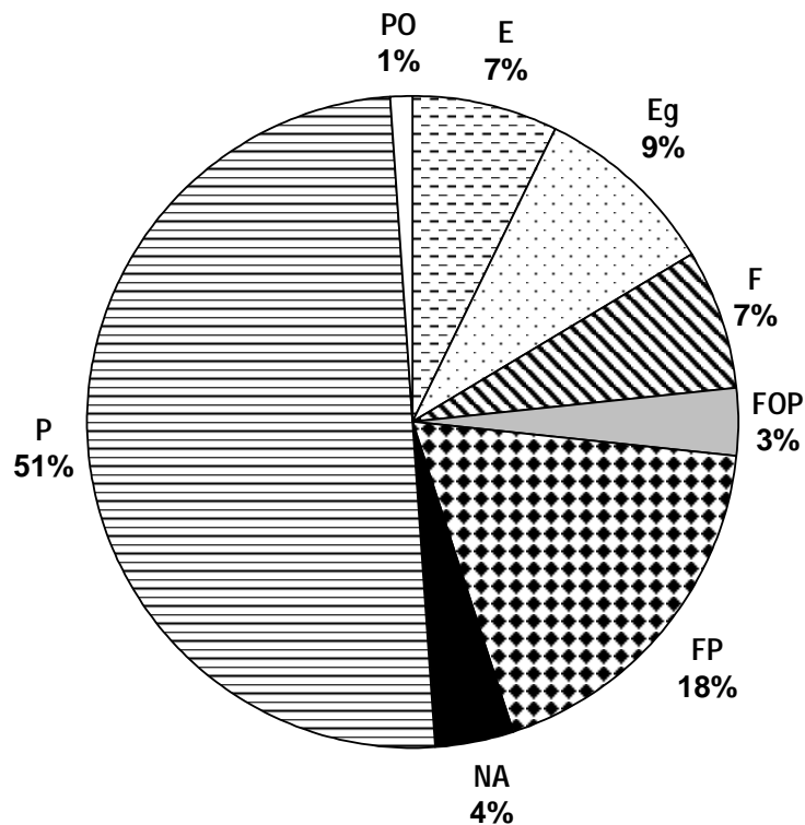
Figure 5: The faunal composition of carabid fauna and its zoogeographical affinities in Sinai Peninsula. E Endemic to Sinai; EG: Endemic to Egypt; F: Afrotropical; FOP: Afrotropico- Palaeartic-Oriental; FP: Afrotropico-Palaeartic; NA: confined to North Africa only; P: Palaeartic; PO: Palaeartic-Oriental.
