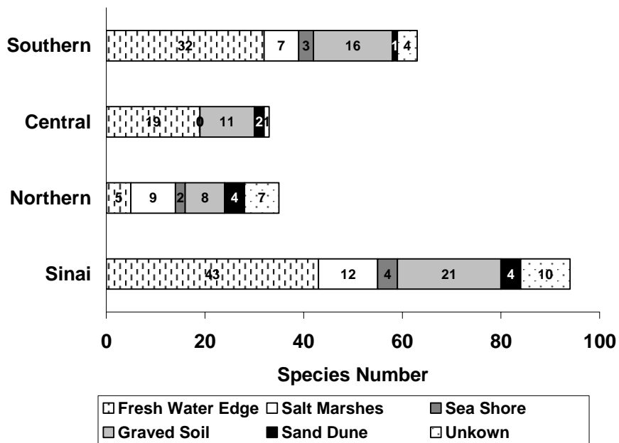
Figure 8: Distribution of carabid species among different habitats in Sinai and its different geomorphological parts.
