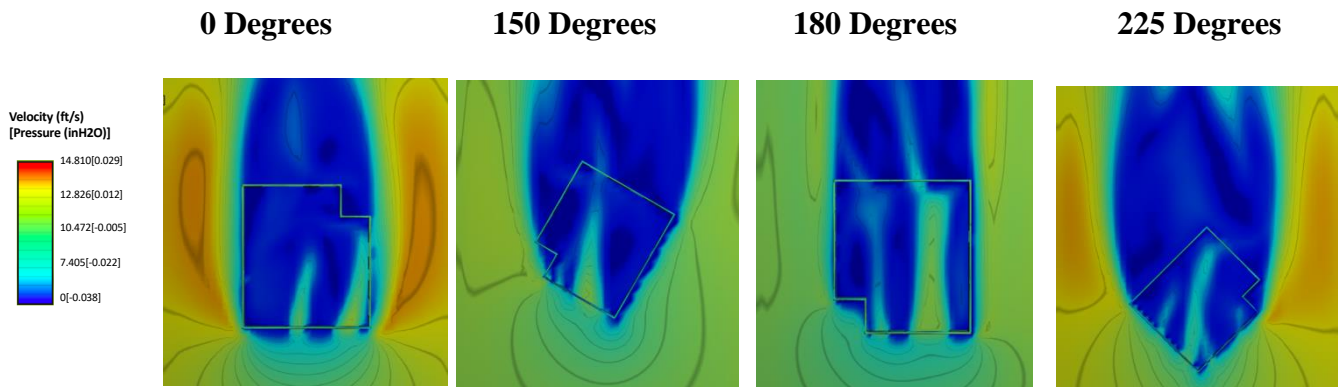
Figure 4. Pressure difference relationship with the wind direction against the building with open windows and doors, (unit conversion: 1 ft/s= 0.305m/s, 1 H2O=248.8 pascal)
