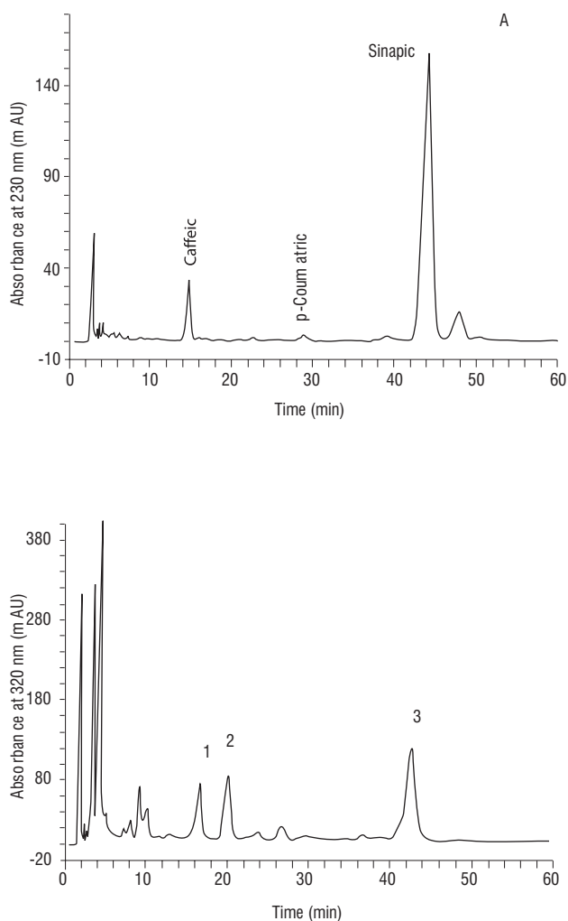
FIGURE 2. HPLC chromatogram of phenolic acids in white cabbage and sauerkraut extract;
