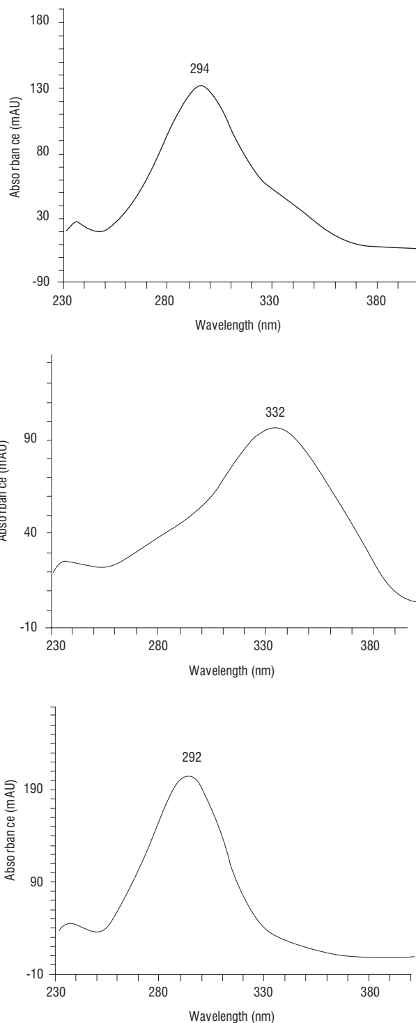
FIGURE 3. UV spectra of phenolic compounds separated from the white cabbage extract after acid hydrolysis using HPLC method; 1-3 – numbers like in FIGURE 2.
