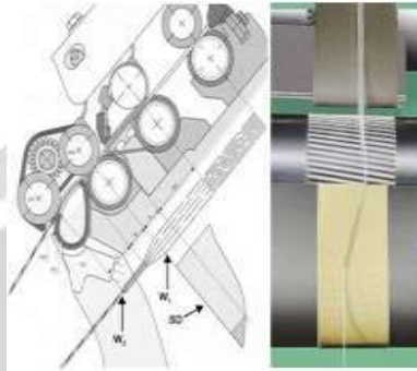
Fig 1:- The Elite Compacting System [9]
