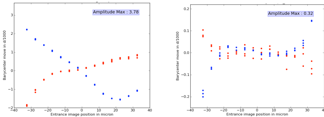
Figure 4. Near Field scrambling measurements with Figure 3 set-up. Left: for a FVP circular fiber 100\ \mu\text{m} . Right: for the octagonal piece fusion spliced between two pieces of circular fiber 100\ \mu\text{m} . The points represent the barycenter displacements of the output near field during a scan of a 35\ \mu\text{m} – diameter spot at N=2.3 on the core of the tested fiber assembly, in units of 1000^{\text{th}} of fiber diameter. Red and Blue points are for the X and Y axis.
