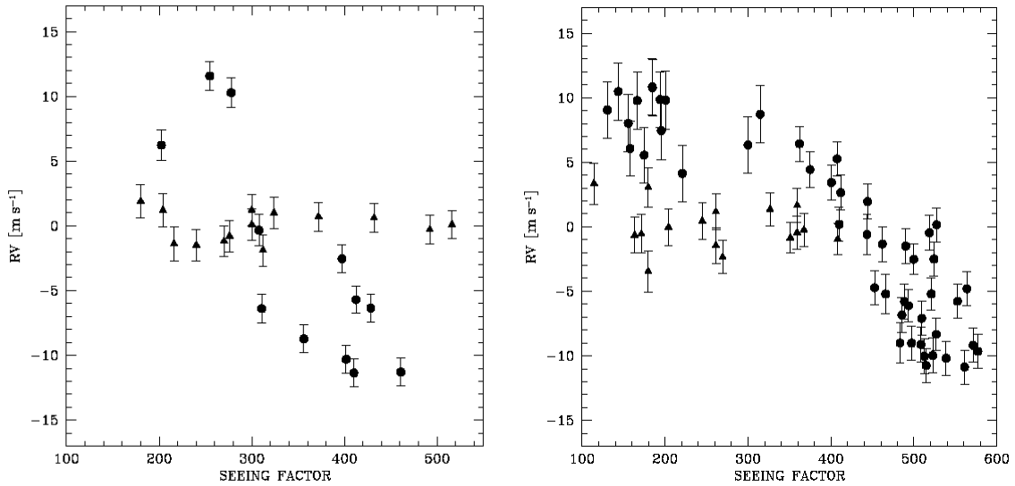
Figure 8. Radial velocity changes as function of the seeing factor showing a clear correlation when the previous configuration is used (circles). Triangles: use of the new configuration. Left: HD185144. Right: HD109358.
