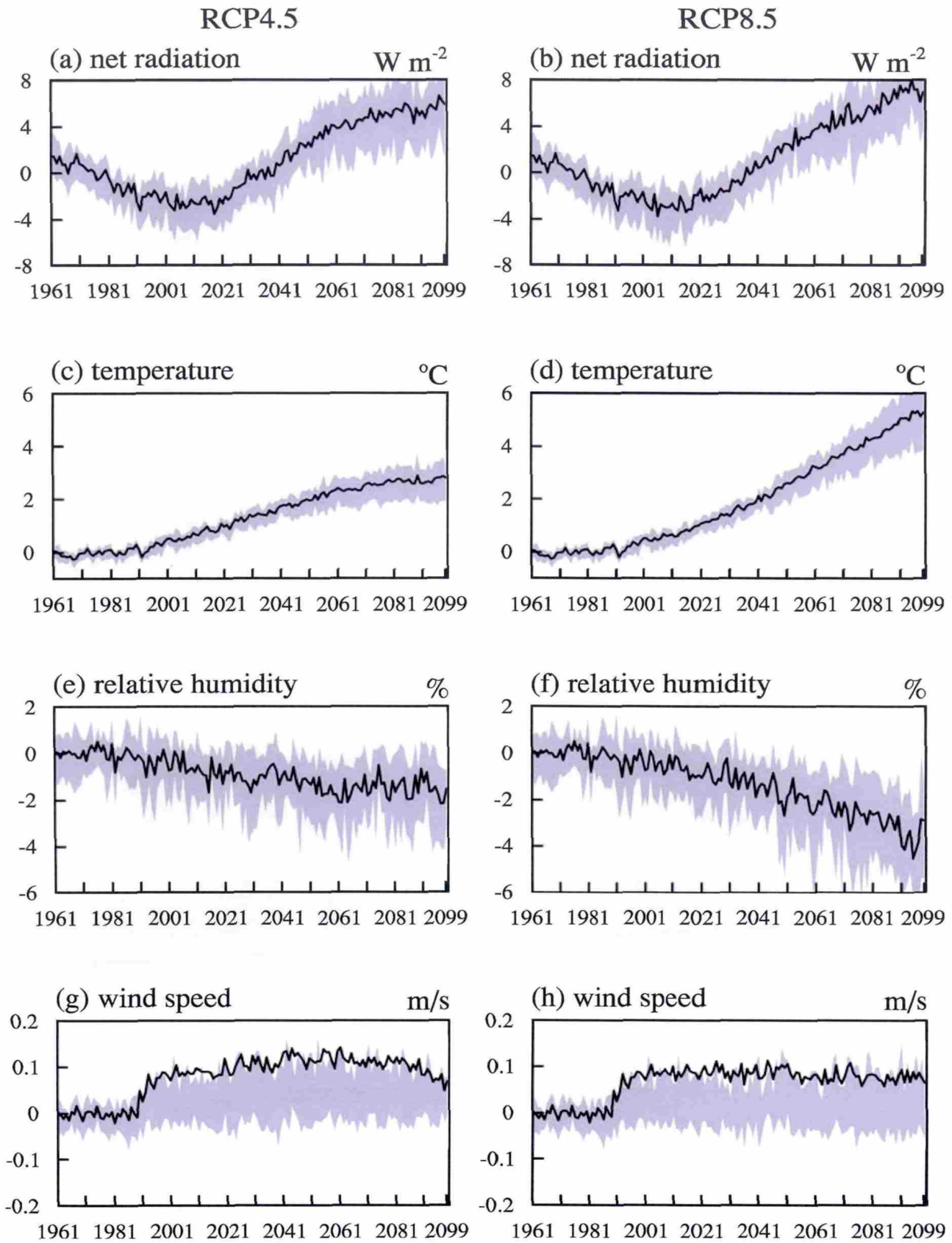
Fig. 6. Anomalies of (a, b) annual mean surface net radiation (units: W m^{-2} ), (c, d) temperature (units: ^{\circ}C ), (e, f) relative humidity (units: %), and (g, h) wind speed (units: m s^{-1} ) under RCP4.5 and RCP8.5 averaged over Southwest China during 1961–2099 relative to the 1961–90 average. The black line and blue shading denote the ensemble mean and interquartile range across all GCMs, respectively.
