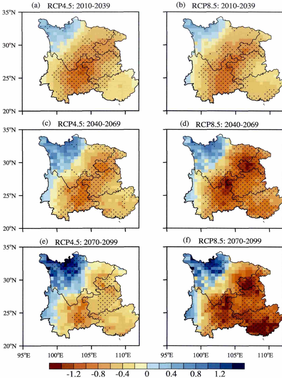
Fig. 9. The same as Fig. 8 but for SPEI at the time scale of 48 months.
