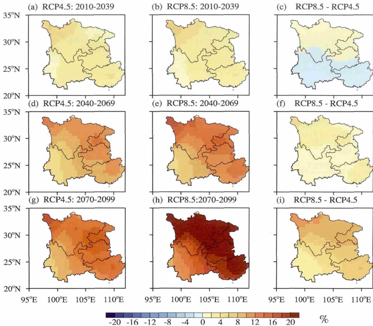
Fig. 5. The same as Fig. 3 but for potential evapotranspiration. The stippling shown in Fig. 3 to indicating how robust these changes are is omitted here due to almost all GCMs agreeing on the sign of the mean change (positive).
