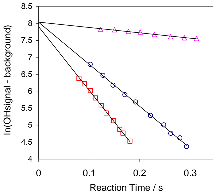
Fig. 2. Pseudo-first-order decays of \ln(\text{OH signal} - \text{background}) versus reaction time. The upper decay ( \blacktriangle ) was obtained using zero-air in the laboratory, and the solid line is a linear-least squares fit to these data, the gradient of which gives a physical loss rate of 1.88 \pm 0.09 \text{ s}^{-1} . The two lower decays ( \circ and \square ) are examples from field measurements, the solid lines are fits to these data which give OH reactivities of 12.46 \pm 0.15 \text{ s}^{-1} and 18.59 \pm 0.21 \text{ s}^{-1} , respectively, after correction for the physical loss. The errors quoted are the 1 sigma random errors from the linear least-squares fitting routine.
