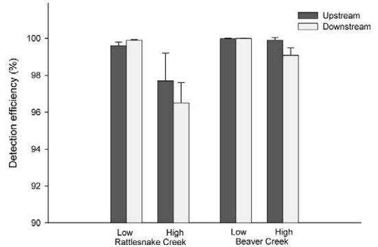
FIGURE 6.—Efficiency of detection of PIT-tagged fish moving upstream or downstream (mean + SE) past PIT tag interrogation systems consisting of three arrays and six antennas in Rattlesnake and Beaver creeks under two flow conditions: low ( \leq 0.14 \text{ m}^3/\text{s} in Rattlesnake Creek and \leq 0.57 \text{ m}^3/\text{s} in Beaver Creek) and high ( > 0.14 \text{ m}^3/\text{s} and > 0.57 \text{ m}^3/\text{s} ).
