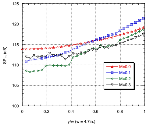
Plane 1, corrected, extrapolated, 1500 Hz ( \Delta f = 4 Hz, Linm0-0 May 27, Linm0-1 May 29, Linm0-2 June 25, Linm0-3 June 25)
