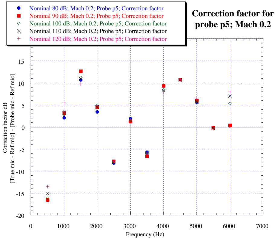
Figure Correction for probe p5; Mach 0.2; [True mic - Ref mic] - [Probe mic - Ref mic] Nominal velocity +/- 5%; \Delta f = 4 Hz.
