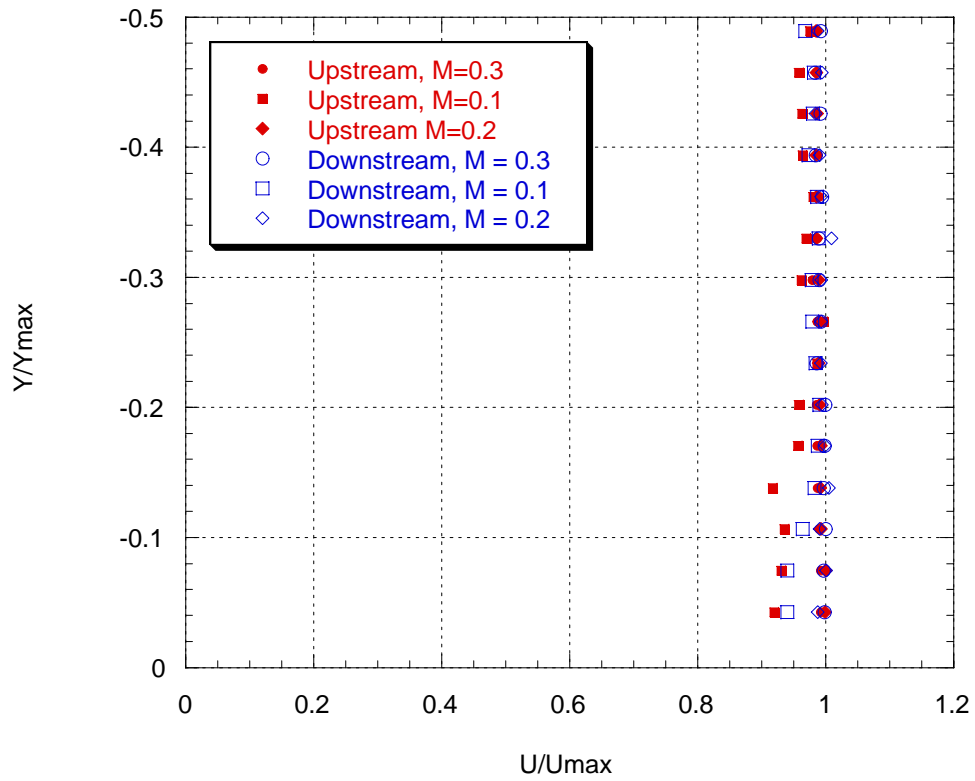
Velocity profiles for M = 0.1 , M = 0.2 , M = 0.3 Hardwall, Major Axis
