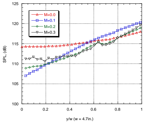
Plane 2, corrected, extrapolated, 1500 Hz ( \Delta f = 4 Hz, Linm0-0 May 27, Linm0-1 May 29, Linm0-2 June 25, Linm0-3 June 25)
