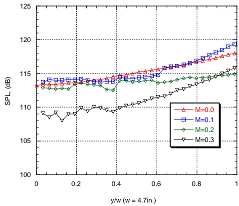
Plane 1, corrected, extrapolated, 2500 Hz ( \Delta f = 4 Hz, Linm0-0 May27 Linm0-1 May29, Linm0-2 June 25, Linm0-3 June 25)
