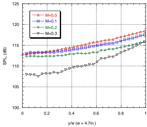
Plane 2, corrected, extrapolated, 2500 Hz ( \Delta f = 4 Hz, Linm0-0 May27 Linm0-1 May29, Linm0-2 June 25, Linm0-3 June 25)
