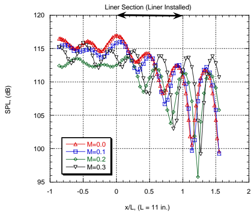
Axial, 1500 Hz, \Delta f = 4 Hz (linm0-0 May 27, linm0-1 May 29, linm0-2 Jun 25, linm0-3 June 25)
