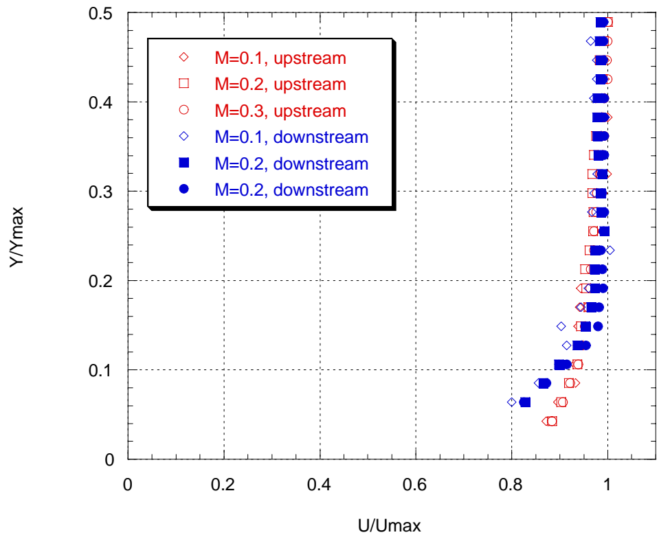
Major axis, Liners installed 2 short walls, Upstream and Downstream planes velocity profiles (up1a, up2a, up3a, dn1, dn2, dn3, velocity profiles, 6/23)
