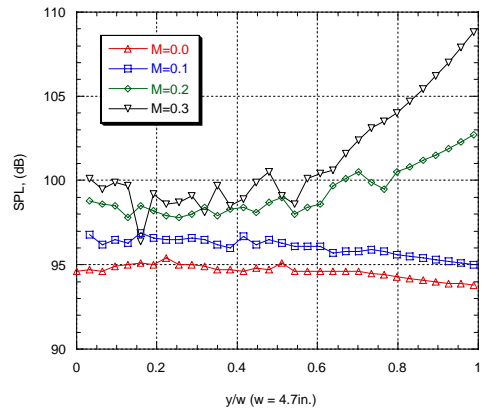
Plane 3, corrected, extrapolated, 1000 Hz ( \Delta f = 4 Hz, Linm0-0 May 27 Linm0-1 May 29, Linm0-2 June 25, Linm0-3 June 25)
