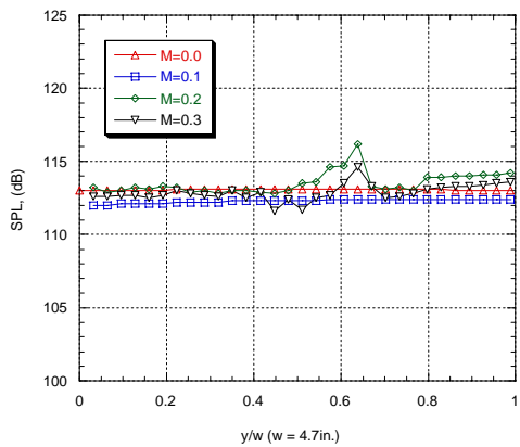
Plane 2, corrected, extrapolated, 1000 Hz ( \Delta f = 4 Hz, Linm0-0 May 27 Linm0-1 May 29, Linm0-2 June 25, Linm0-3 June 25)
