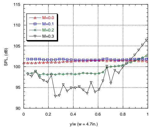
Plane 4, corrected, extrapolated, 2500 Hz ( \Delta f = 4 Hz, Linm0-0 May27 Linm0-1 May29, Linm0-2 June 25, Linm0-3 June 25)
