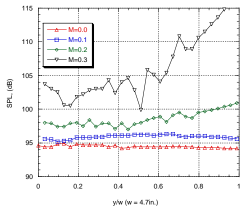
Plane 4, corrected, extrapolated, 1000 Hz ( \Delta f = 4 Hz, Linm0-0 May 27 Linm0-1 May 29, Linm0-2 June 25, Linm0-3 June 25)
