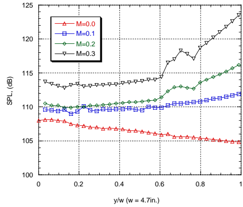
Plane 3, corrected, extrapolated, 1500 Hz ( \Delta f = 4 Hz, Linm0-0 May 27, Linm0-1 May 29, Linm0-2 June 25, Linm0-3 June 25)
