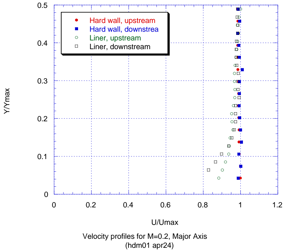
Figure 17. Velocity profiles for hard wall and lined wall cases for Mach number = 0.2.
