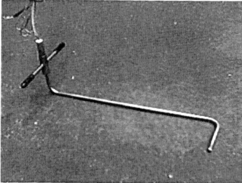
Figure 7. Pressure probe used for flow measurements.
