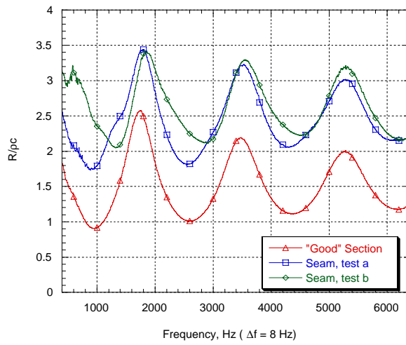
Normal Impedance tests of ceramic liner used in flow duct measurements (test CL 9/1/98, CT 9/2/98)
