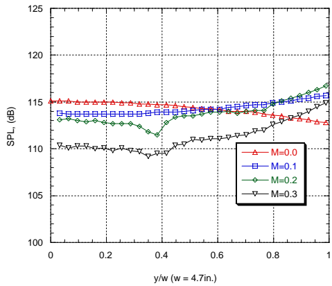
Plane 1, corrected, extrapolated, 2000 Hz ( \Delta f = 4 Hz, Linm0-0 May 27 Linm0-1 May 29, Linm0-2 June 25, Linm0-3 June 25)
