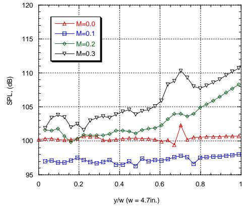
Plane 3, corrected, extrapolated, 2000 Hz ( \Delta f = 4 Hz, Linm0-0 May 27 Linm0-1 May 29, Linm0-2 June 25, Linm0-3 June 25)
