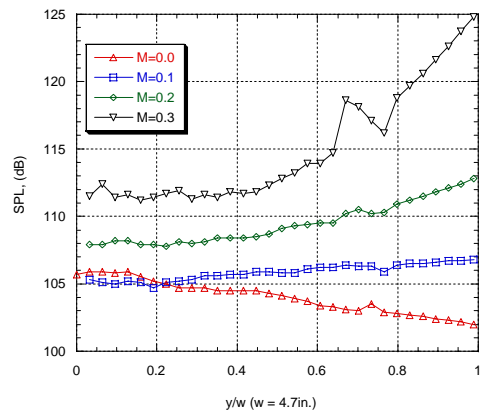
Plane 4, corrected, extrapolated, 1500 Hz ( \Delta f = 4 Hz, Linm0-0 May 27, Linm0-1 May 29, Linm0-2 June 25, Linm0-3 June 25)
