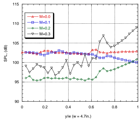
Plane 4, corrected, extrapolated, 2000 Hz ( \Delta f = 4 Hz, Linm0-0 May 27 Linm0-1 May 29, Linm0-2 June 25, Linm0-3 June 25)
