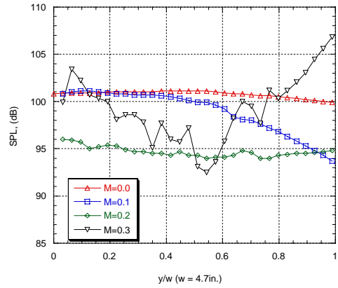
Plane 3, corrected, extrapolated, 2500 Hz ( \Delta f = 4 Hz, Linm0-0 May27 Linm0-1 May29, Linm0-2 June 25, Linm0-3 June 25)
