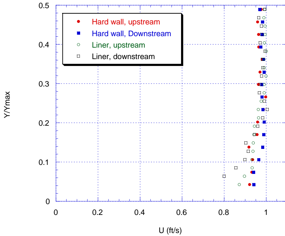
Figure 16. Velocity profiles for hard wall and lined wall cases for Mach number = 0.1.
