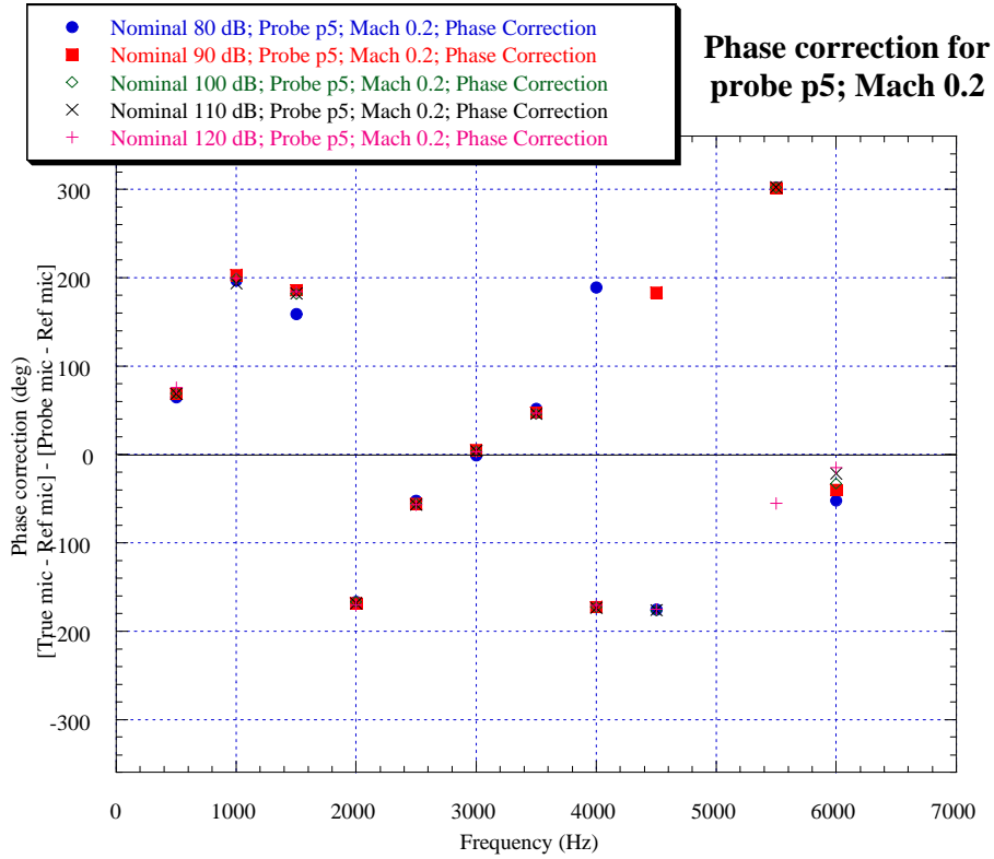
Figure Phase correction for probe p5; Mach 0.2; [True mic - Ref mic] - [Probe mic - Ref mic] Nominal velocity +/- 5%; \Delta f = 4 Hz.
