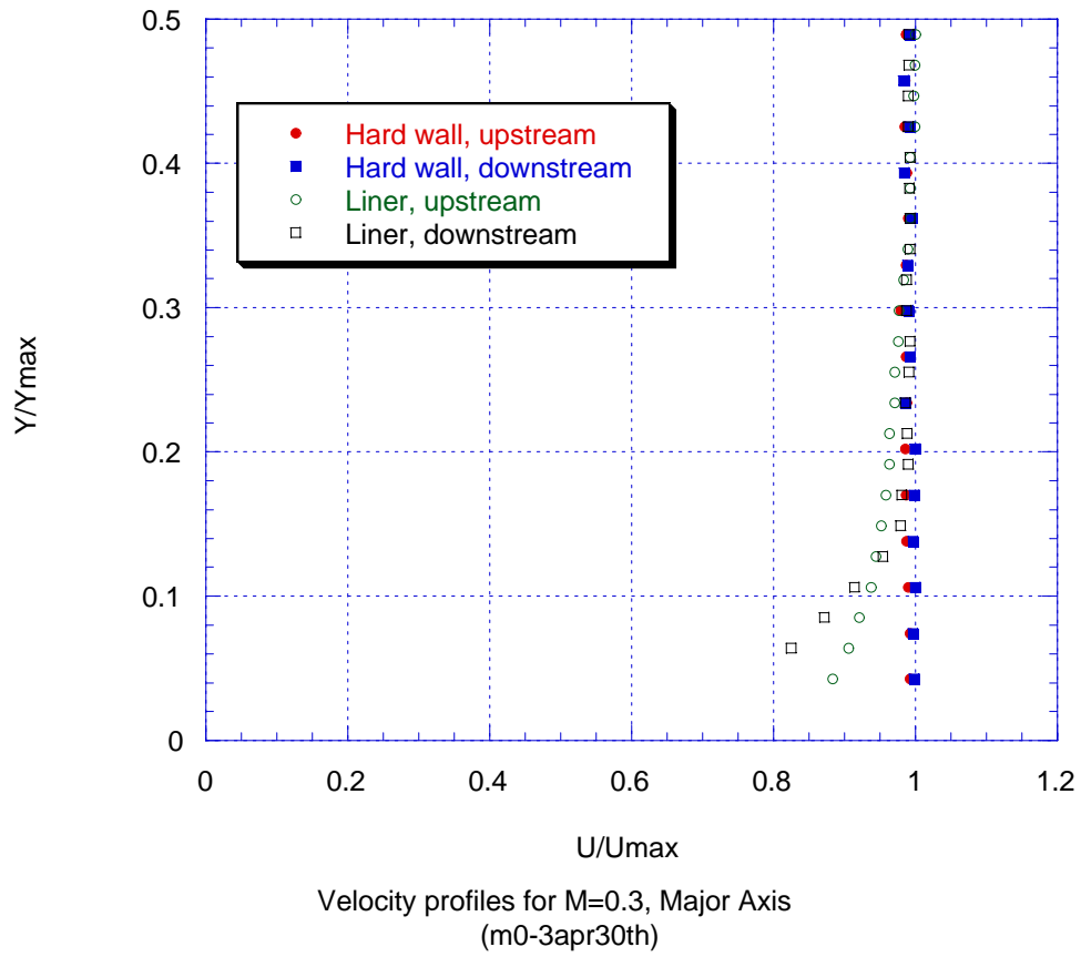
Figure 18. Velocity profiles for hard wall and lined wall cases for Mach number = 0.3.
