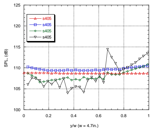
Plane 4, corrected, extrapolated, 500 Hz ( \Delta f = 4 Hz, Linm0-0 May 27 Linm0-1 May 29, Linm0-2 June 25, Linm0-3 June 25)
