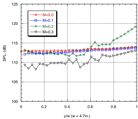
Plane 2, corrected, extrapolated, 500 Hz ( \Delta f = 4 Hz, Linm0-0 May 27 Linm0-1 May 29, Linm0-2 June 25, Linm0-3 June 25)
