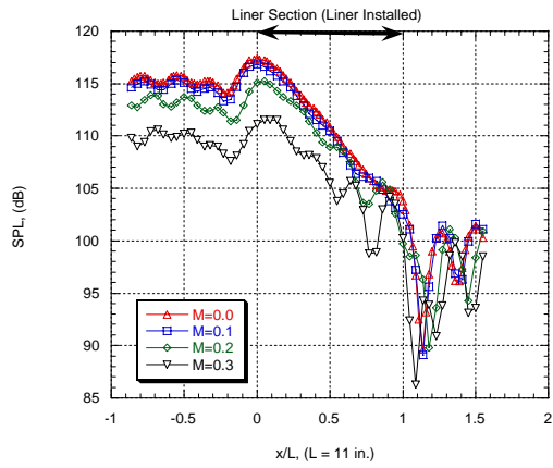
Axial, 2500 Hz, \Delta f = 4 Hz (linm0-0 May 27, linm0-1 May 29, linm0-2 jun25, linm0-3 June 25)
