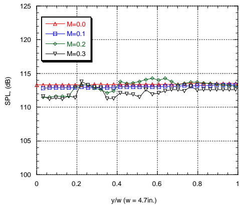
Plane 1, corrected, extrapolated, 1000 Hz ( \Delta f = 4 Hz, Linm0-0 May 27 Linm0-1 May 29, Linm0-2 June 25, Linm0-3 June 25)
