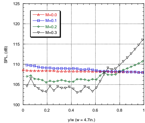
Plane 3, corrected, extrapolated, 500 Hz ( \Delta f = 4 Hz, Linm0-0 May 27 Linm0-1 May 29, Linm0-2 June 25, Linm0-3 June 25)
