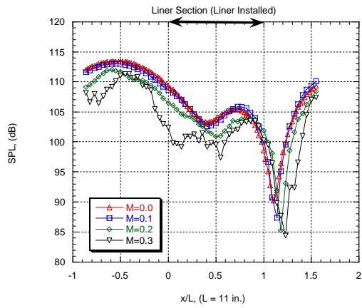
Axial, 500 Hz, \Delta f = 4 Hz (linm0-0 May 27, linm0-1 May 29, linm0-2 Jun 25, linm0-3 June 25)
