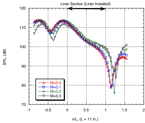
Axial, 1000 Hz, \Delta f = 4 Hz (linm0-0 May 27, linm0-1 May 29, linm0-2 Jun 25, linm0-3 June 25)
