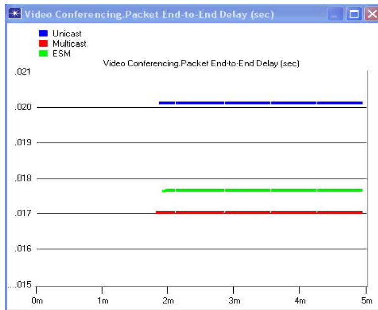
Figure 5. Average end-to-end packet delays for multiple unicast, IP multicast and ESM simulations.
