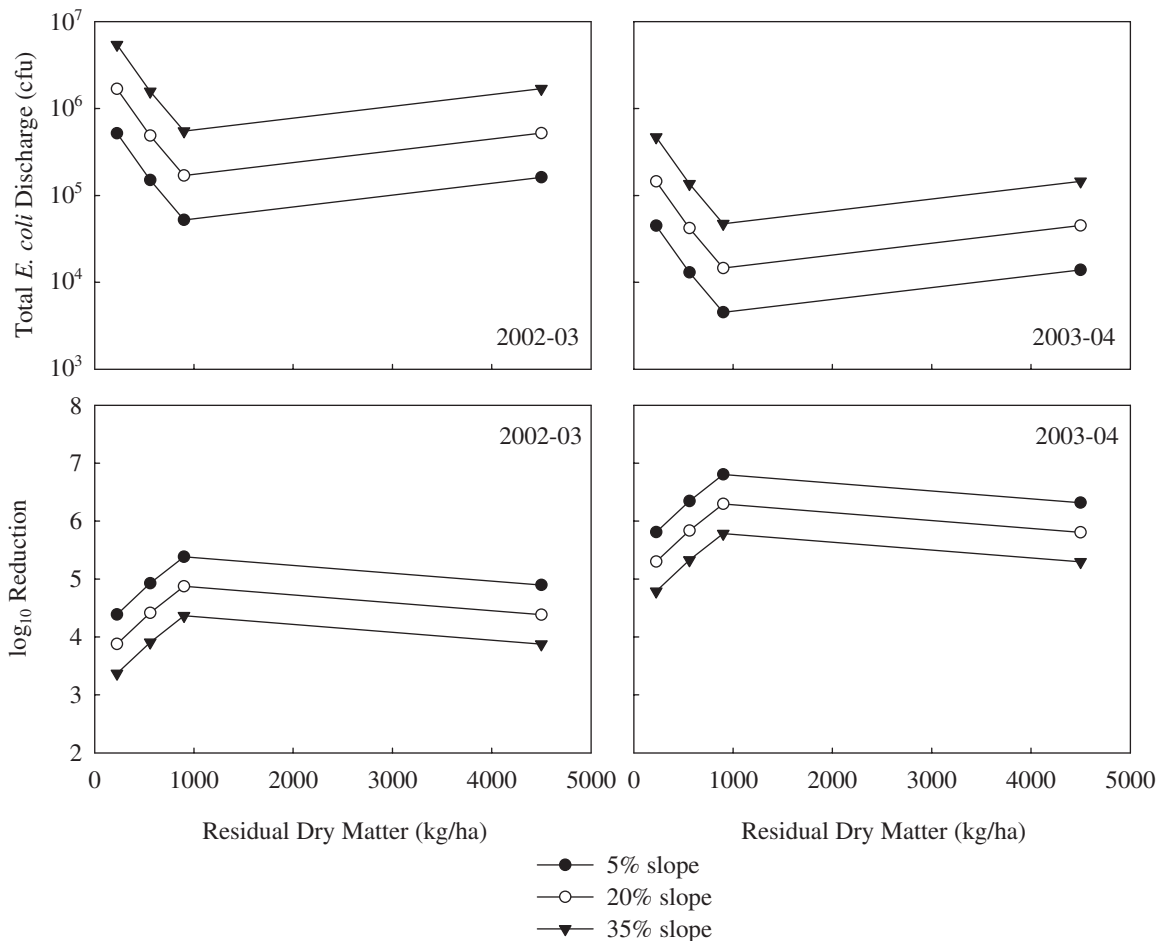
Fig. 8. Relationship of total E. coli discharge (cfu) and \log_{10} reduction in discharge due to residual dry vegetation matter and land slope for storm series observed during portions of the 2002–2003 and 2003–2004 rainfall season contained in the study period.
