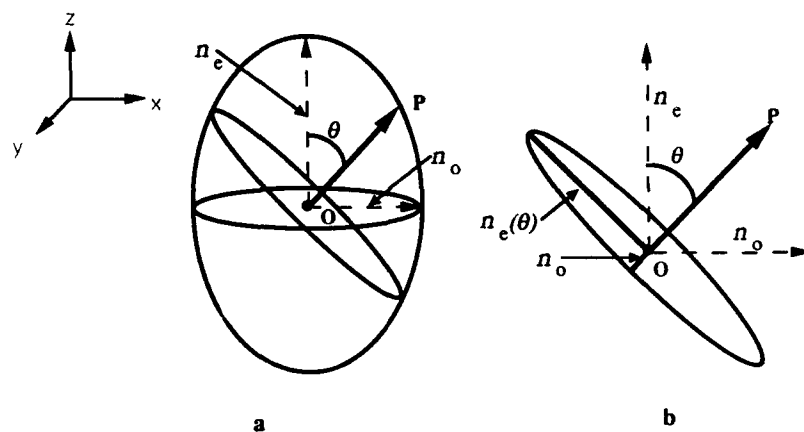
Figure 12. (a) Index ellipsoid defined by n_e and n_o with a ray of light propagating in an arbitrary direction OP ; (b) an ellipse that is formed by the intersection of the plane normal to OP and the index ellipsoid. The principal axes of this ellipse are the angularly dependent index n_e(\theta) and the angularly independent index n_o .
