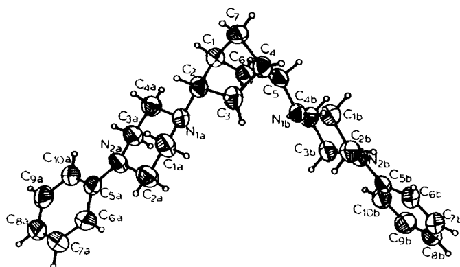
Figure 1. X-ray crystal structure of endo,endo-2,5-bis(4-phenylpiperazinylnorbormane.
