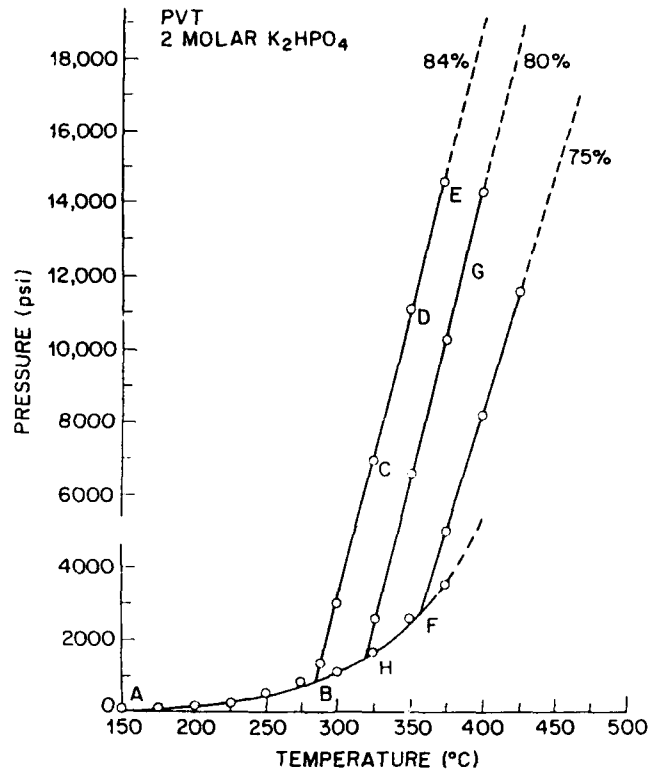
Figure 10: P-% fill-T behavior of K_2HPO_4
