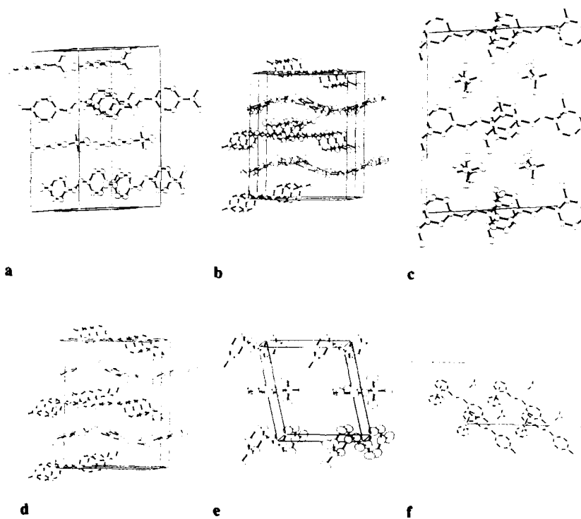
Figure 1. Packing diagrams for a (4)-(CH_3)_2NC_6H_4-CH=CH-(4)-C_5H_4N(CH_3)^+p-CH_3C_6H_4SO_3^- , b (4)-CH_3OC_6H_4-CH=CH-(4)-C_5H_4N(CH_3)^+Cl^- \cdot 4H_2O , c (4)-CH_3OC_6H_4-CH=CH-(4)-C_5H_4N(CH_3)^+Cl^- \cdot 4H_2O , d (4)-BrC_6H_4-CH=CH-(2)-C_5H_4N(CH_3)^+CF_3SO_3^- , e (3,4)-(OH)_2C_6H_3-CH=CH-(4)-C_5H_4N(CH_3)^+p-CH_3C_6H_4SO_3^- , and f (C_5H_5)Fe(C_5H_4)-CH=CH-(4)-C_5H_4N(CH_3)^+NO_3^-
