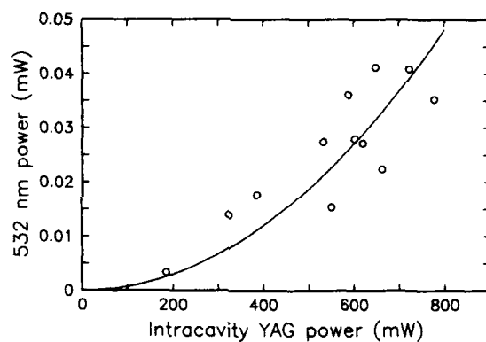
Figure 4. Peak SHG output vs peak intracavity power.
