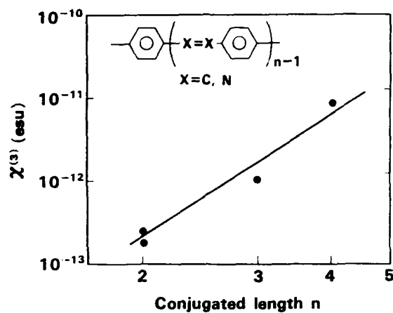
Figure 3. \pi -electron conjugation length dependence of \chi^{(3)} for azobenzene and stilbene dyes.
