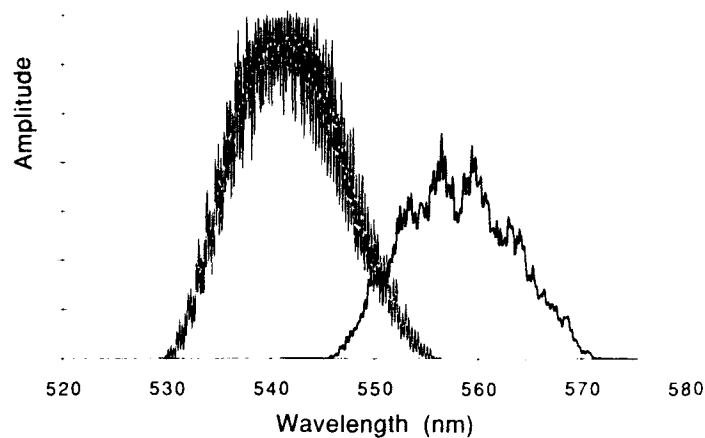
Figure 2. Spectral output of free running coumarin 153 in ethanol (left) and in aged silica gel (right.)
