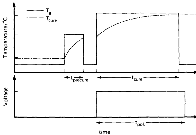
Figure 7. Schematic of thermal processing and poling procedure for a thermoset NLO polymer.
