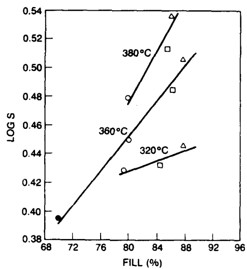
Figure 5: Quartz solubility dependence on % fill
