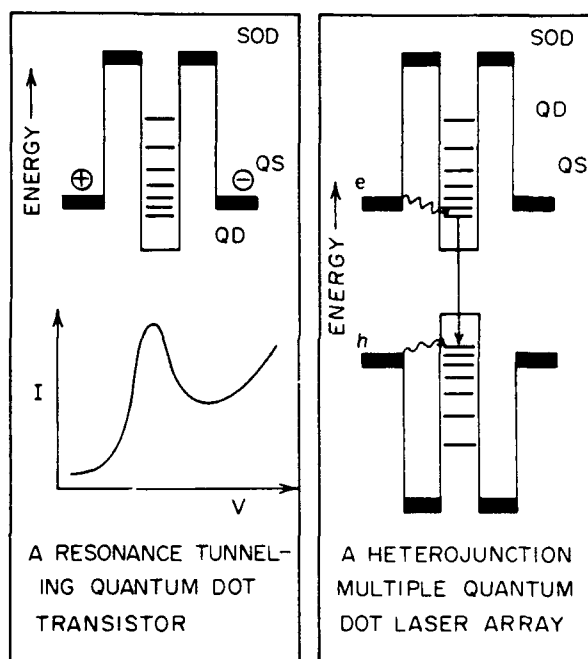
Figure 5. Qualitative electronic state (miniband) band diagrams envisaged for 8Ag_{(2-p)}X_pY -SOD as a new material for a chemistry approach to a resonance tunneling quantum dot transistor and a heterojunction multiple quantum dot laser array.
