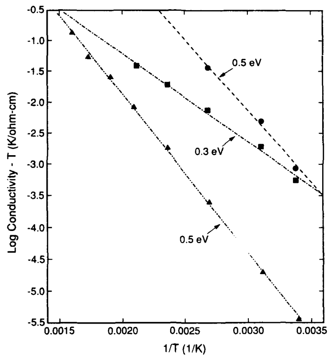
Figure 2. Conductivity data on KTP and KTA, along z, as a function of temperature for determination of the activation energies of conduction. Key: ● KTP Philips flux; ■ KTP Airtron high temperature hydrothermal; ▲ KTA DuPont flux.
