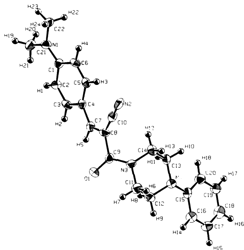
Figure 2. X-ray crystal structure of 4-dimethylamino- \beta -cyanocinnamic phenylpiperazinamide.
