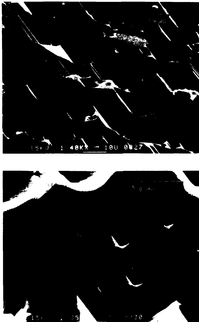
Figure 7. SEM photomicrographs of a quadrilateral face of a Py-D3C crystal in an early stage of growth. Arrows indicate a growth step.
