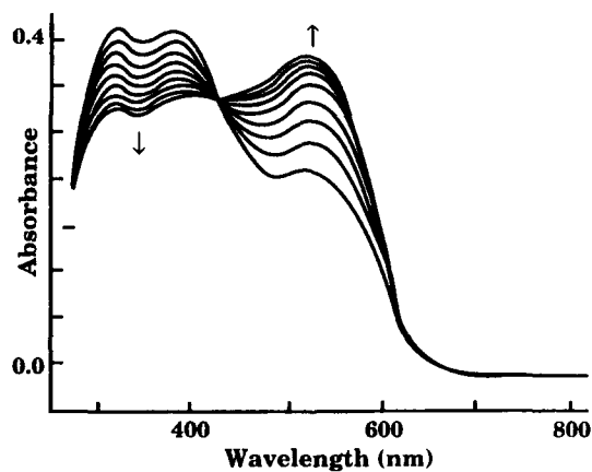
Figure 5. UV-Visible spectra of poly(TMSCOT) in carbon tetrachloride ( 10^{-6} M) obtained between eight periods of photolysis (10 sec each).
