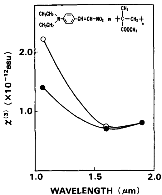
Figure 6. \chi^{(3)} wavelength dependence of a DEANST doped PMMA. ●; measured value, ○; compensated for 3\omega wave absorption
