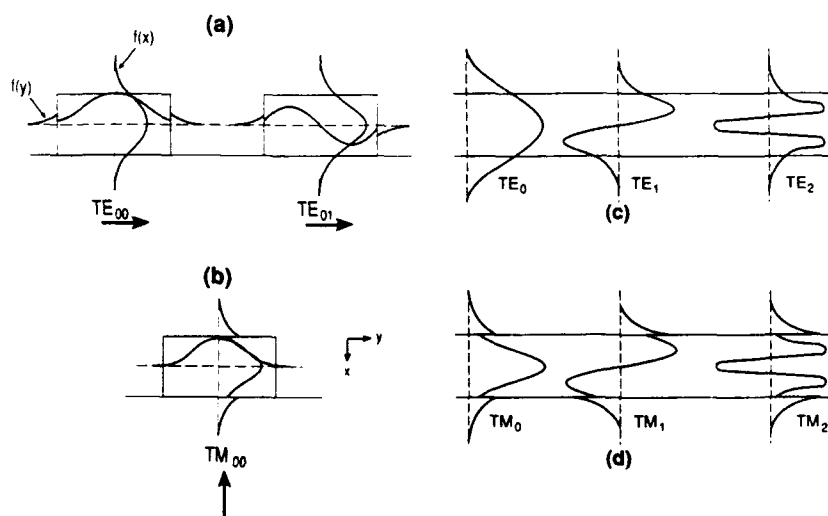
Figure 2. Typical field distributions for waveguides. For the channel case, the transverse distribution f(x,y) is approximated by f(x)f(y) . The arrows indicate the dominant field component. (a) TE_{mn} channel modes, (b) TM_{mn} channel modes, (c) TE_m slab field distributions and, (d) TM_m slab waveguide fields.
