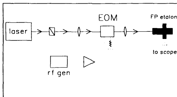
Figure 5. Experimental setup for electro-optic phase modulation.
