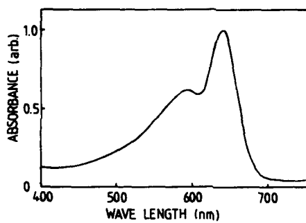
Figure 6. Absorption curve of a vacuum evaporated PDA blue film.
