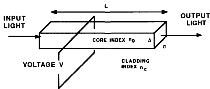
Figure 1. Parameters for a Polymer Channel Waveguide
