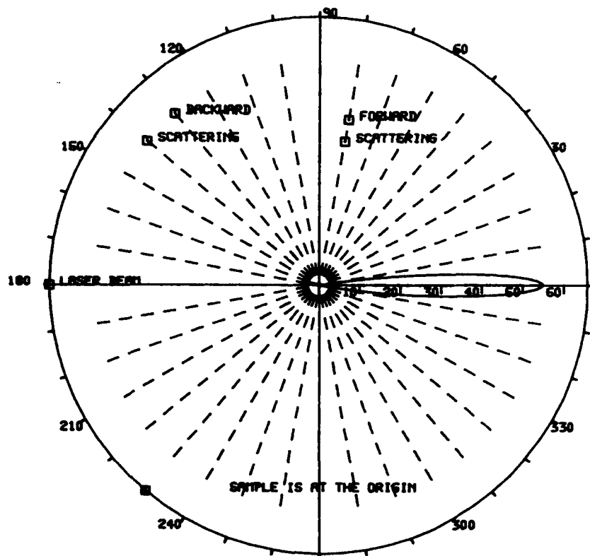
Figure 3. Angular dependence of SHG response (relative to \alpha - \text{SiO}_2 ) of a BADP/PAA (70 wt %) composite; this sample contains well aligned needle crystals.
