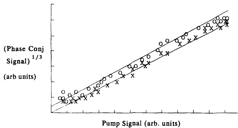
Figure 4. Degenerate four wave mixing in Carbon disulphide (x) and bis [1,2-diphenyl-1,2-ethenedithiolato(2-)-S,S'] Nickel (o).
