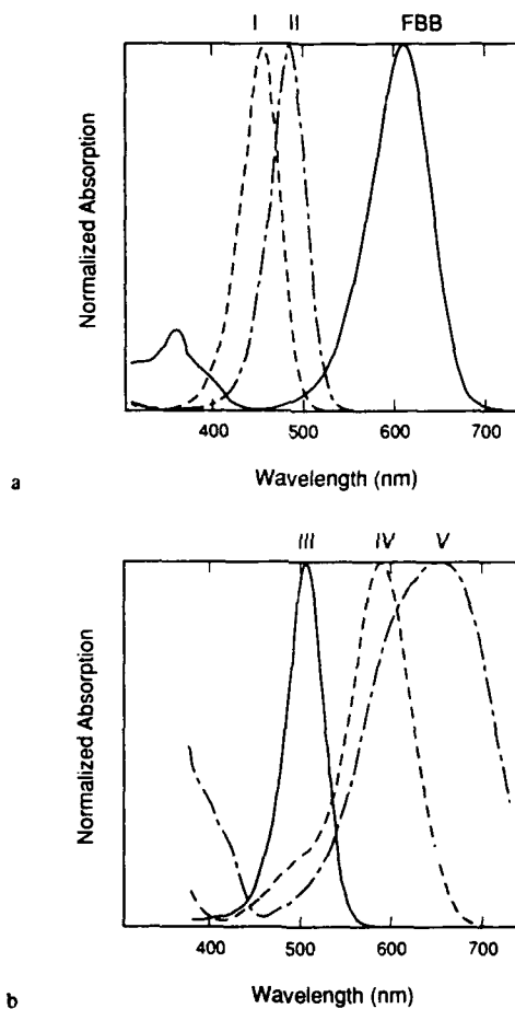
Figure 5. Normalized spectra of Foron Brilliant Blue S-R and analogs. (a) Sulfones (b) Ketones and derivatives
