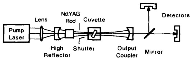
Figure 3. Experimental setup for intracavity SHG using an organic NLO crystal placed in the cuvette.
