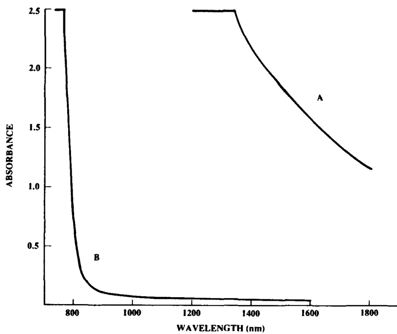
Figure 7. UV-Visible-Near IR spectra of films of poly(COT) (A) and poly( n -butylCOT) (B).
