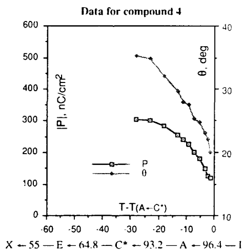
Figure 3. Phase sequence, polarization and tilt angle data as a function of temperature for compounds 3 and 4.
