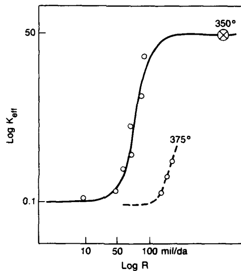
Figure 6: Dependence of the effective partition coefficient for (OH)^- impurity in quartz on growth rate
