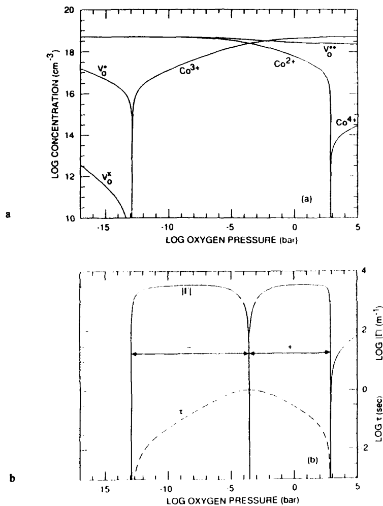
Figure 2. (a) Point defect concentrations as a function of oxygen partial pressure for \text{BaTi}_{0.9}\text{Co} processed at 800^\circ\text{C} . (b) Calculated gain and response time for the model shown in (a).
