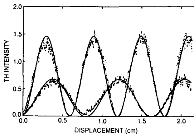
Figure 2. Wedge THG interference fringes for solution of DPB in toluene (larger signal) and for neat toluene using 1907 nm fundamental light. The wedge cell angle was 0.26^\circ . (Reproduced with permission from ref 27. Copyright 1989 Royal Society of Chemistry)
