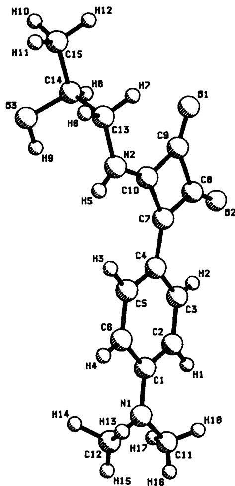
Figure 3. Molecular structure of (-)-4-(4'-dimethylamino-phenyl)-3-(2'-hydroxypropylamino)cyclobutene-1,2-dione (DAD), as determined by X-ray crystallography. C, carbon ; N, nitrogen ; O, oxygen ; and H, hydrogen.
