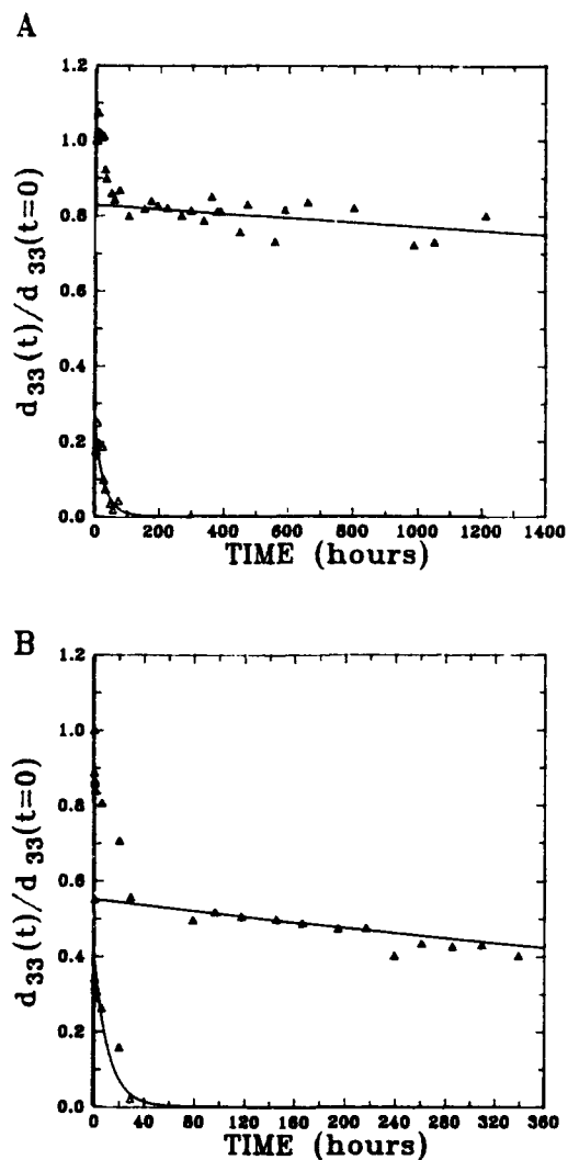
Figure 1. (A) Time dependence of the second harmonic coefficient of a PPO-NPP film (1.4 NPP moieties per polymer repeat unit) contact-poiled at 1.2 MV/cm. Decay data taken at 25°C. The data points are shown as filled triangles. The two curves describing the biexponential fit to equation 1 are shown separately, with the open triangles representing data points dominating the short-term decay. (B) Time dependence of the second harmonic coefficient of a corona-poiled PPO-NPP film (1.4 NPP moieties per repeat unit). Decay data taken at 25°C. The data points are shown as filled triangles. The two curves describing the biexponential fit to equation 1 are shown separately, with the open triangles representing data points dominating the short-term decay.
