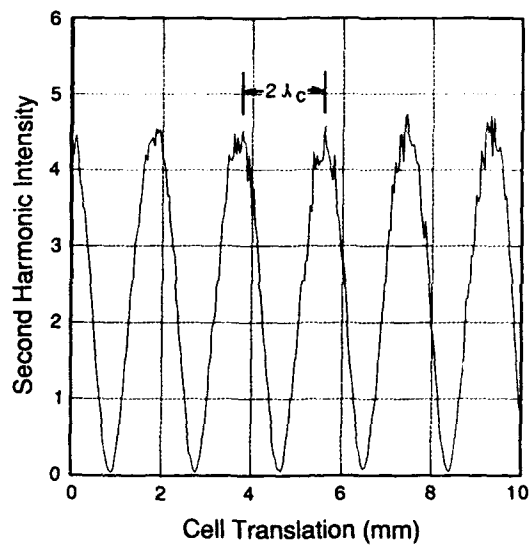
Figure 10. Experimental EFISH trace for nitrobenzene.
