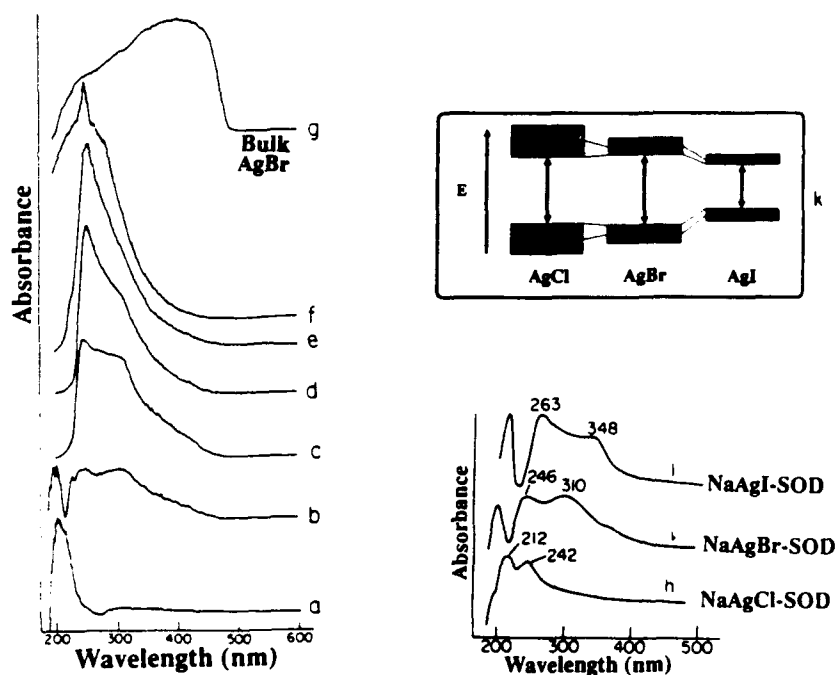
Figure 2. UV-visible reflectance spectra of (8-2n)\text{Na}_2\text{nAg}_2\text{Br-SOD} with varying silver concentrations. \text{Ag}^+/\text{uc} : (a) 0; (b) 0.05; (c) 0.28; (d) 2.0; (e) 3.1; (f) 8.0; (g) bulk AgBr; (h) (8-2n)\text{Na}_2\text{nAg}_2\text{Cl-SOD} , 0.1 \text{Ag}^+/\text{uc} ; (i) (8-2n)\text{Na}_2\text{nAg}_2\text{Br-sodalite} , 0.1 \text{Ag}^+/\text{uc} ; (j) (8-2n)\text{Na}_2\text{nAg}_2\text{I-SOD} , 0.1 \text{Ag}^+/\text{uc} . Note that band-gap absorptions for 8\text{Na}_2\text{X-SOD} expanded insulators peak at 192 (Cl), 208 (Br), and 214 nm (I) (Figure 2h,i,j) and parallel the order for the bulk fcc NaX materials, 138 (Cl), 165 (Br), and 211 nm (I), respectively. (k) Schematic band diagram for expanded AgX semiconductors (Reprinted from ref. 3. Copyright 1990 American Chemical Society.)
