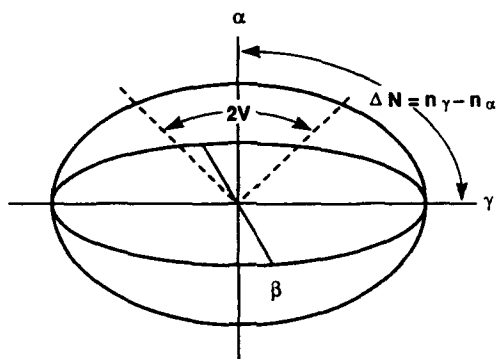
Figure 1. The biaxial indicatrix, whose principal axes correspond to the refractive indices n_\alpha \leq n_\beta \leq n_\gamma . The optic axes are indicated by dashed lines and the optic angle is denoted 2V . N is the principal birefringence.
