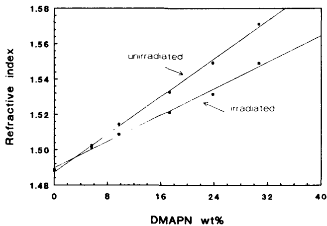
Figure 2. Refractive indexes ( \pm 0.005 , 633 nm) of DMAPN/PMMA films before (●) and after (■) irradiation vs. wt% DMAPN incorporated.
