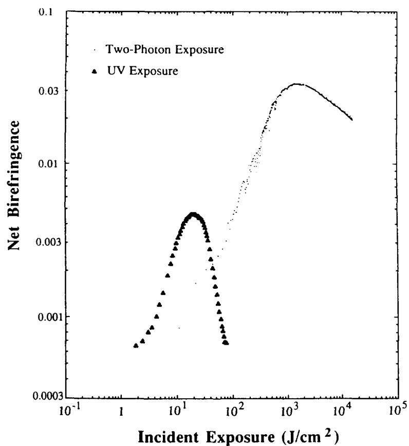
Figure 3. Birefringence ( \Delta n ) versus incident exposure in ( \text{J}/\text{cm}^2 ) for polarized UV( \blacktriangle ) and polarized pulsed laser ( \bullet ) exposure. The continuous 325 nm power density was 0.2 \text{ W}/\text{cm}^2 , while the 575 nm pulsed laser intensity (8 ns pulses at 10 Hz) was 1.6 \text{ GW}/\text{cm}^2 . (Reproduced with permission from Ref. 8. Copyright 1990 Elsevier Science Publishers.)
