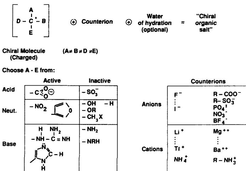
Figure 4. General scheme for the synthesis of chiral organic salts.
