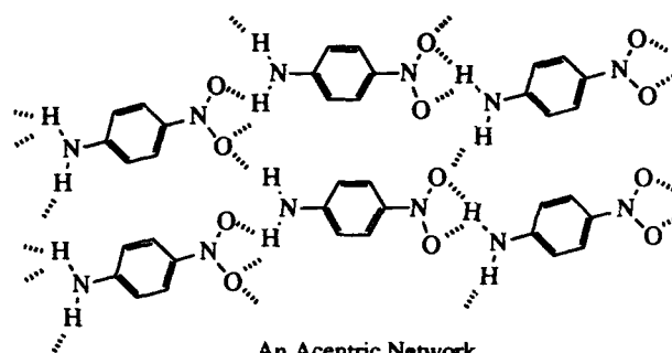
An Acentric Network
