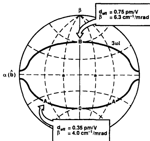
Figure 9. Phasematching loci for type I tripling of 1.664 \mu\text{m} in L-arginine acetate.
