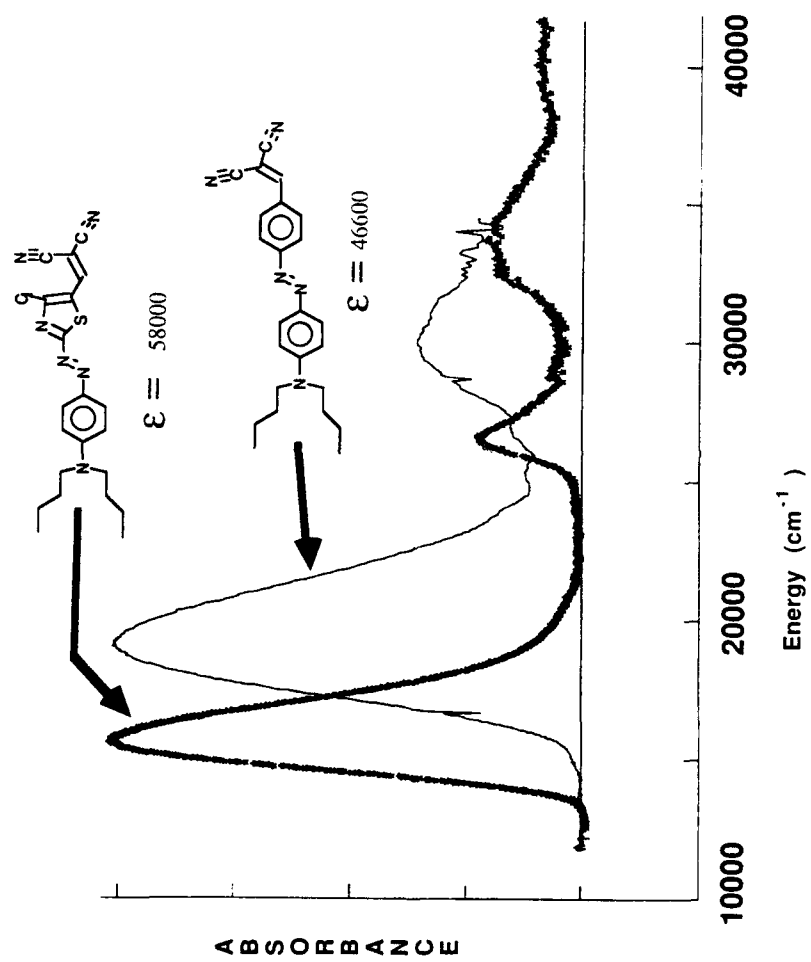
Figure 4. Electronic spectra of analogous benzene and thiazole azo dyes.
