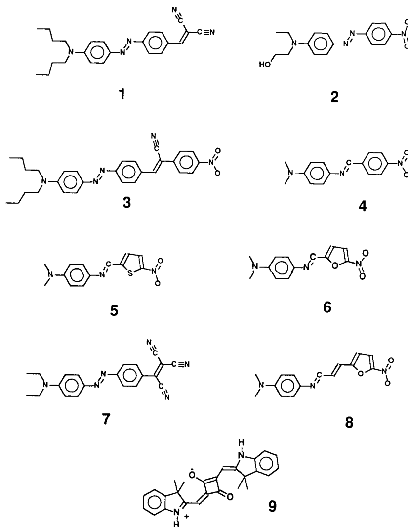
Figure 6. Structures of molecules reported in Table 3.
