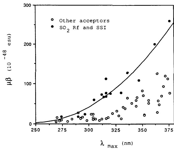
Figure 3. Transparency and nonlinearity trade-offs: \mu\beta vs \lambda_{\max} .
