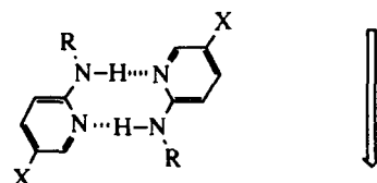
Base Pairs Have Constrained Orientations
