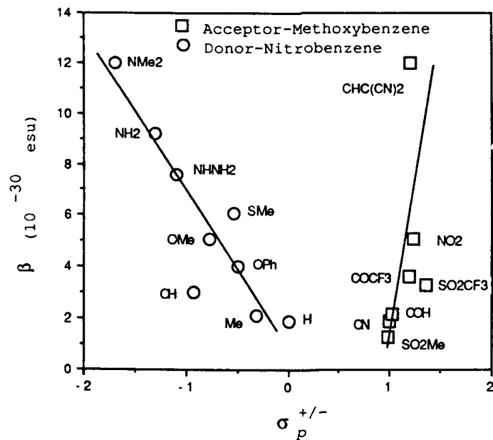
Figure 2. Correlation of \beta and Hammett's Constants.
