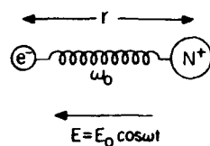
Figure 1. Representation of the Lorentz oscillator.
