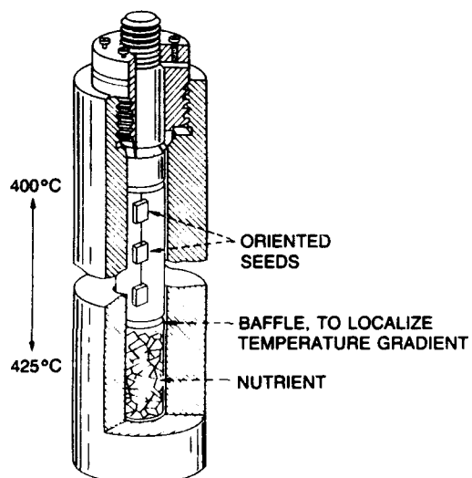
Figure 3: Schematic of hydrothermal synthesis of quartz.
