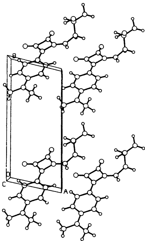
Figure 4. Crystal structure of (-)-4-(4'-dimethylamino-phenyl)-3-(2'-hydroxypropylamino)cyclobutene-1,2-dione (DAD).
