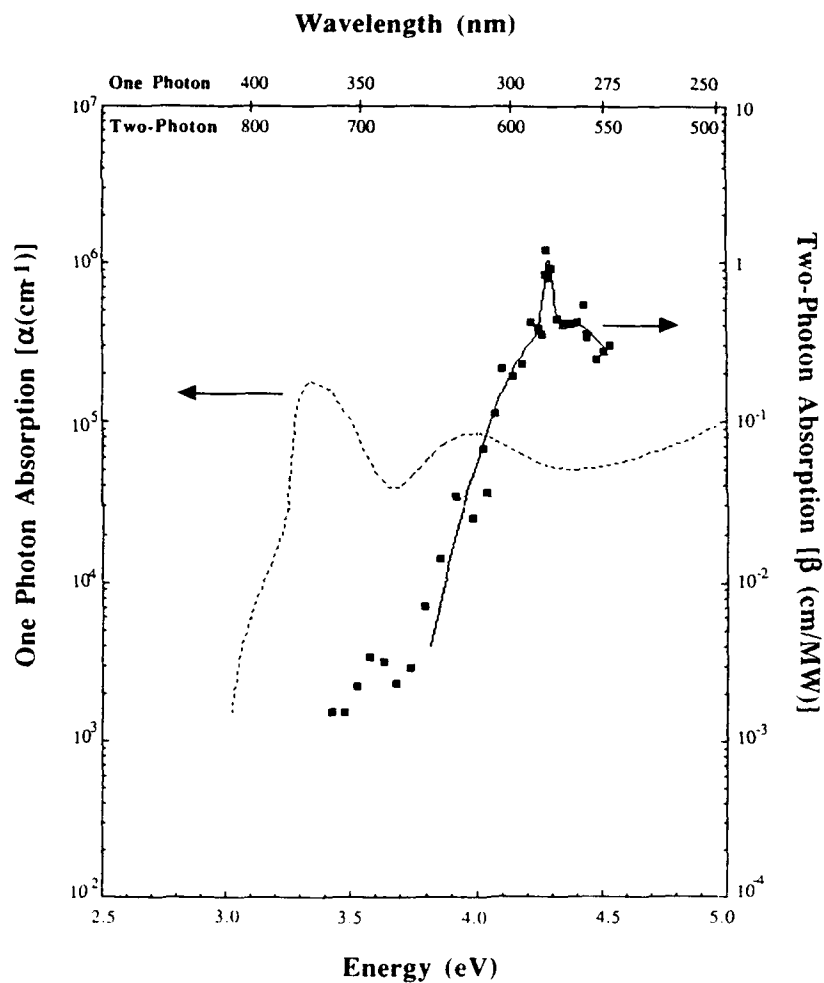
Figure 4. Spectrum of the two-photon absorption coefficient \beta in cm/MW for PIDN6S, calculated from birefringence growth curves as a function of two-photon energy ( \blacksquare ) compared with single-photon absorption spectrum (---). Solid line is a least-squares fit to \beta using the sum of two Gaussians, one broad ( \sim 412 meV), the other narrow ( \sim 33 meV). (Reproduced with permission from Ref. 8. Copyright 1990 Elsevier Science Publishers.)
