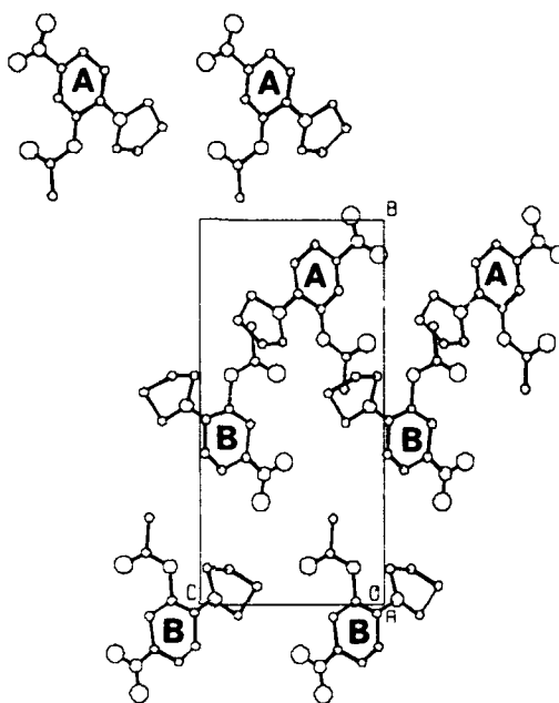
Figure 2. Packing arrangement of the stable \alpha -form of PAN, viewed down the a axis. The two sets of molecules A and B are crystallographically independent, but are related to each other by a pseudo center of inversion. Thus the crystal is non-polar and SHG inactive.
