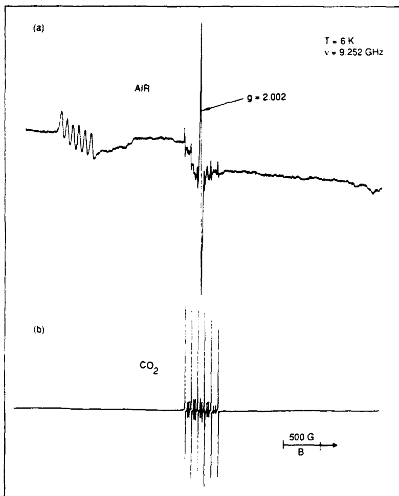
Figure 4. X-band EPR spectra of BaTiO 3 :Mn powders. (a) Sample processed in air. (b) Sample processed in CO 2 .
