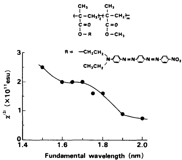
Figure 2. \chi^{(3)} wavelength dependence for bisazo dye attached copolymer.
