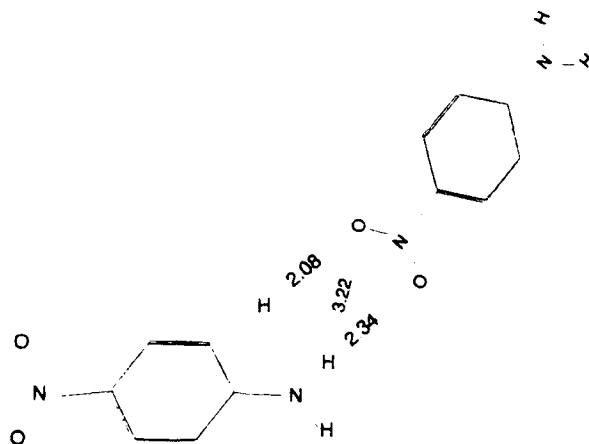
Figure 1C. Structures for p-nitroaniline dimers. Structure obtained by fixing the H-bonds at experimental distances and optimizing the rest. This is not a minimum (due to the constraint).
