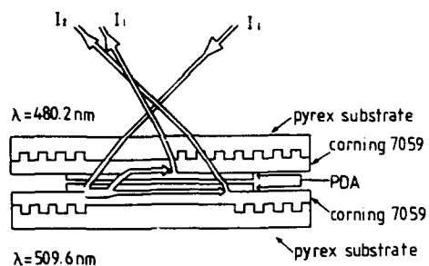
Figure 12. Schematic structure of the nonlinear directional coupler.
