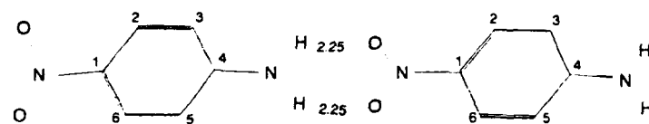
Figure 1A. Structures for p-nitroaniline dimers. Optimal dimer.
