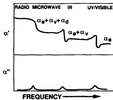
Figure 4. Plot of polarizability of a material as a function of the frequency of the applied field. Top: Real polarizability. Bottom: Imaginary polarizability.
