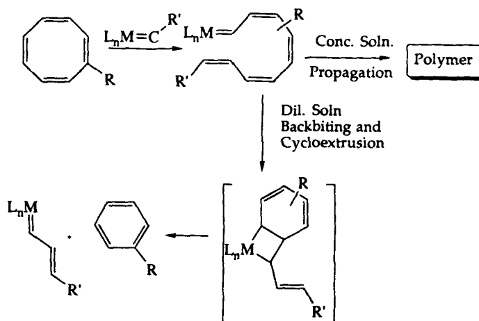
Figure 1. Polymerization of cyclooctatetraenes.
