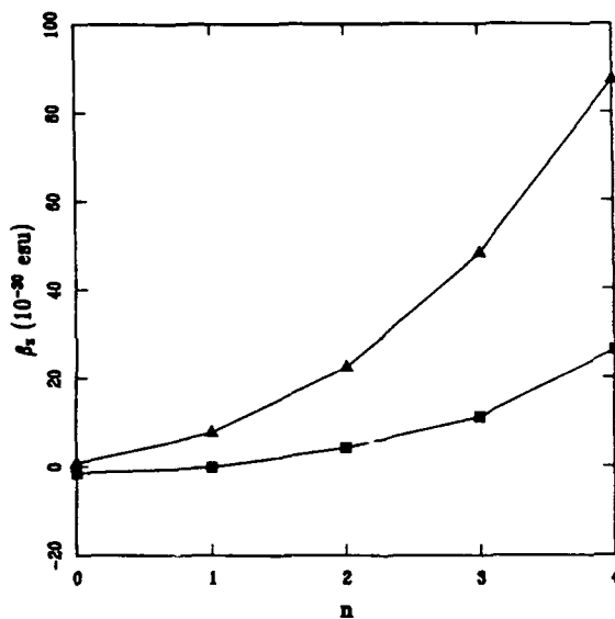
Figure 2. Calculated values (FF) of \beta_2 for H_2N-(CH=CH)_n-NO_2 (▲), and H_2N-(CH=CH)_n-SO_2-CH_3 (■).
