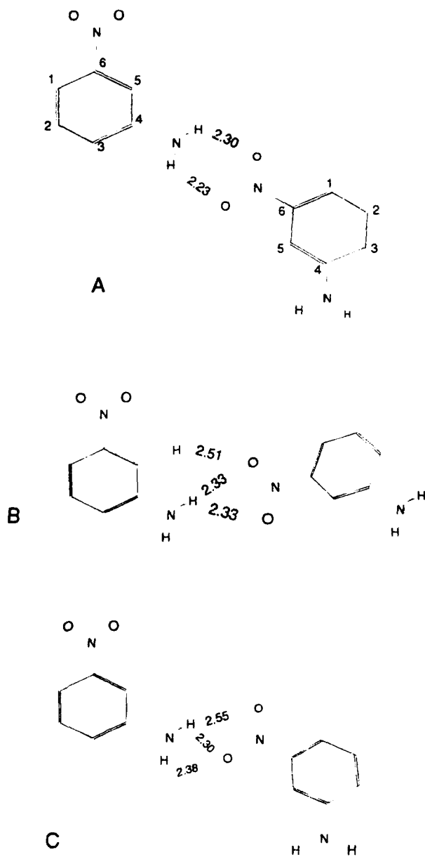
Figure 2. Structures for m-nitroaniline dimers, IIIA-C (structures are labeled as in figure 1).
