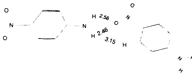
Figure 1C. Structures for p-nitroaniline dimers. Structure obtained by fixing the H-bonds at experimental distances and optimizing the rest. This is not a minimum (due to the constraint).
