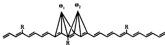
Figure 4. The model compound used in MM2/MM2II computations.
