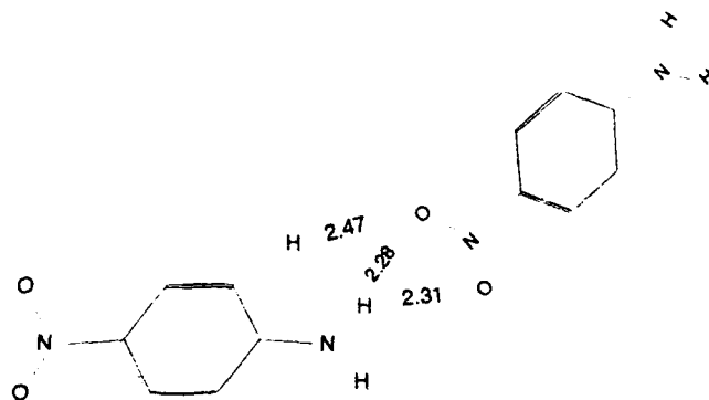
Figure 1B. Structures for p-nitroaniline dimers. Relaxed dimer with at least one H-bond that is the local minimum closest to the crystal structure.
