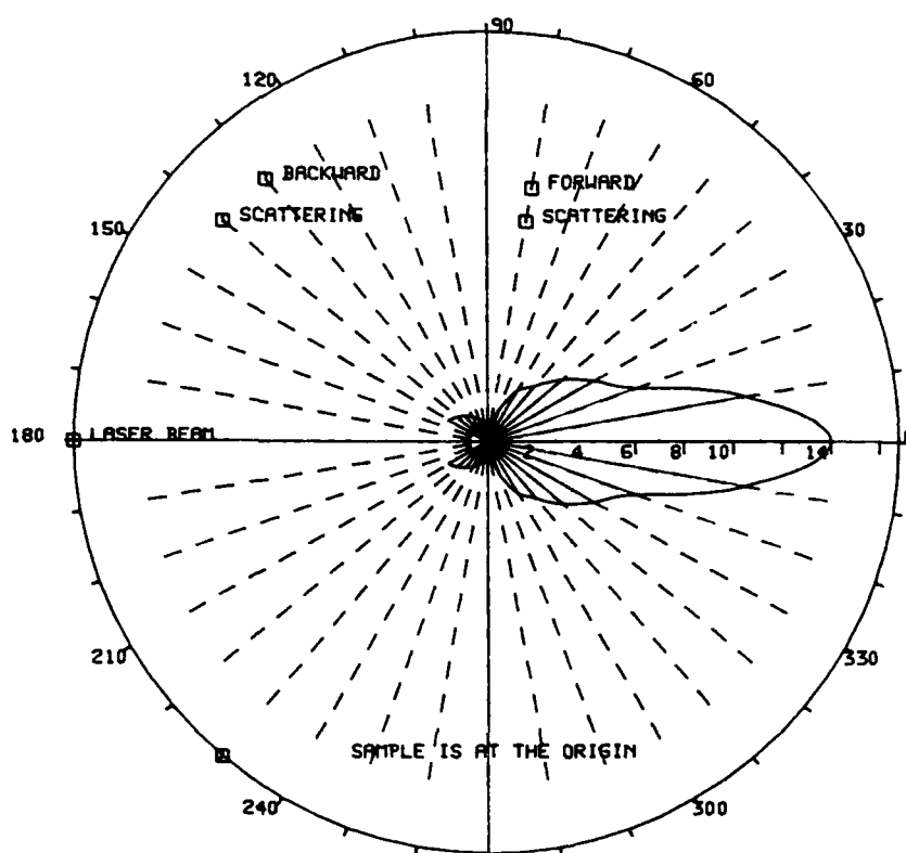
Figure 2a. Angular dependence of SHG response (relative to KDP) of an m NA/PMMA (50 v.t %) composite; this sample contains spherulitic crystals.
