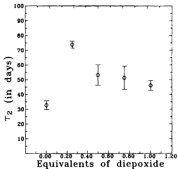
Figure 4. Long-term decay parameters ( \tau_2 , equation 1) for d_{33} of (PS)O-NPP films simultaneously corona poled and cross-linked with the indicated equivalents of 1,4-butanediol diglycidyl ether/equivalents available phenol OH groups.
