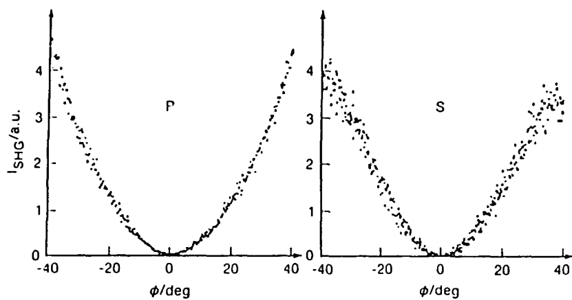
Figure 6. Plots of Maker-fringe data for a poled PPNA film of 1.2\mu m thickness at room temperature (P=p polarization, S=s polarization). (Reproduced with permission from Ref. 12. Copyright 1989 American Institute of Physics.)
