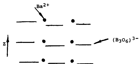
Fig. 4. Schematic drawing of BBO's Lattice net.
