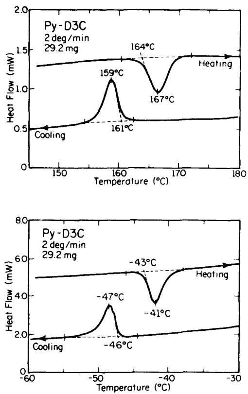
Figure 4. Differential scanning calorimetry curves for Py-D3C.
