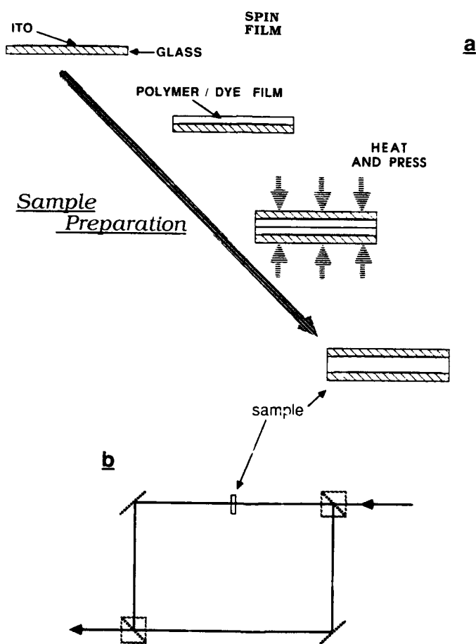
Figure 5. (a) QEO sample preparation. (b) QEO interferometric measurement.
