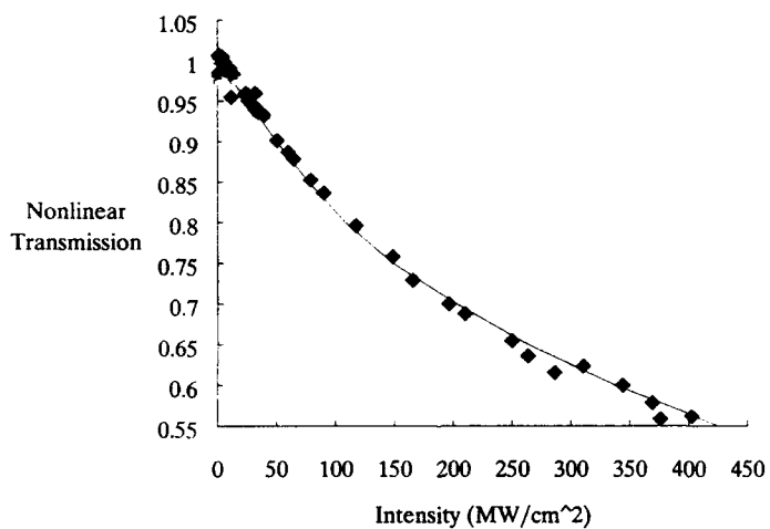
Figure 2. Nonlinear Transmission through bis [1,2-diphenyl-1,2-ethenedithiolato(2-)-S,S'] Nickel.
