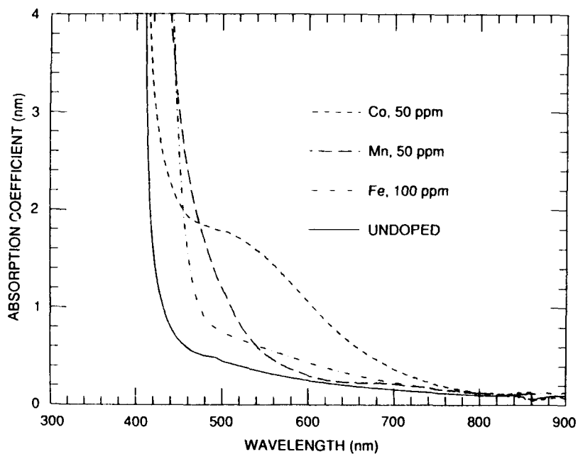
Figure 3. Wavelength dependence of the absorption coefficient (measured with light polarized perpendicular to the c-axis) of undoped and doped \text{BaTiO}_3 crystals. Concentrations refer to dopant atoms per \text{BaTiO}_3 formula unit in the melt.
