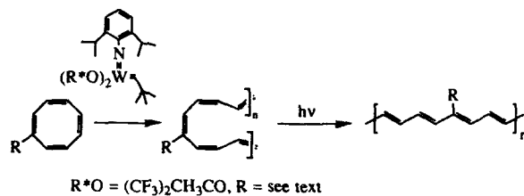
Figure 1. Polymerization of cyclooctatetraenes.
