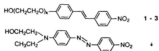
Figure 1. Structures of donor-acceptor substituted, conjugated side groups.
