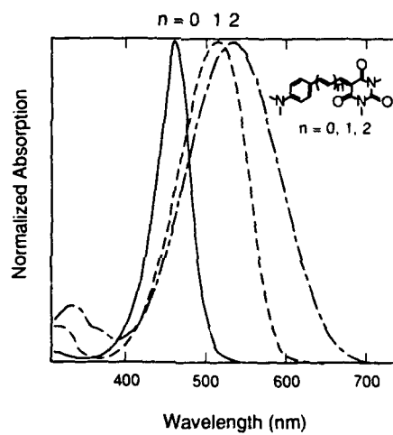
Figure 8. Normalized spectra of extended barbituric acid chromophores.
