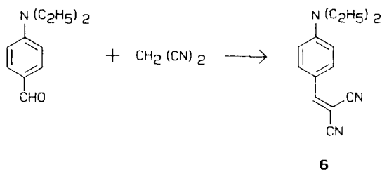
Figure 4. Synthesis of dicyanovinyl derivative 6 .
