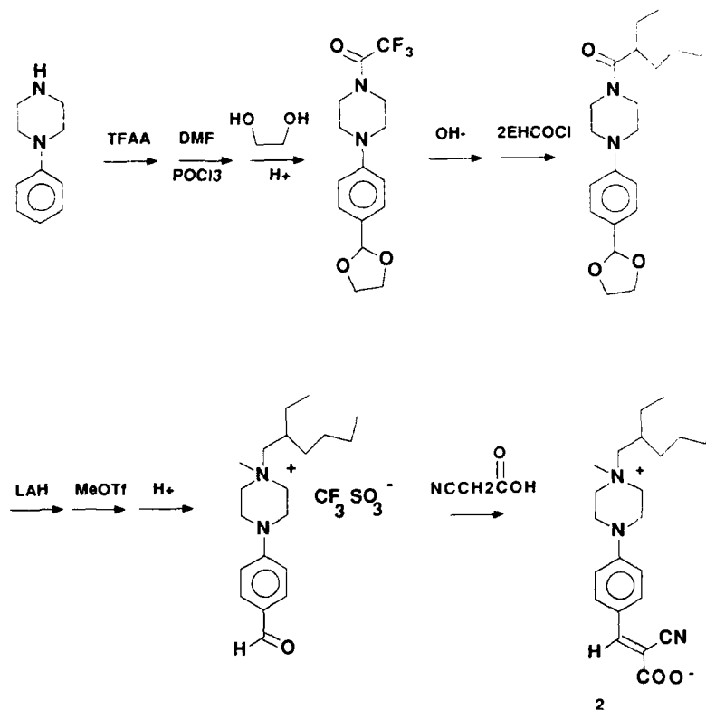
Scheme 1. Abbreviations: TFAA, trifluoroacetic anhydride; DMF, N,N-dimethylformamide; 2EHCOCI, 2-ethylhexanoyl chloride; LAH, lithium aluminum hydride; MeOTf, methyl trifluoromethanesulfonate.
