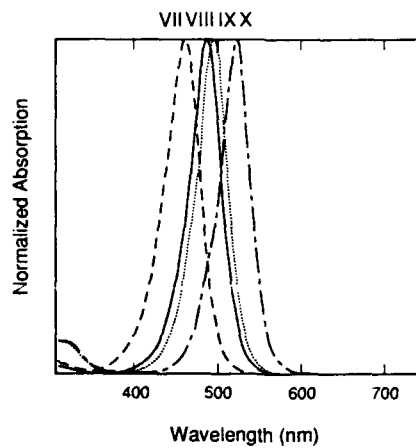
Figure 7. Normalized spectra of barbituric acid dyes.
