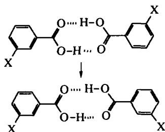
Acid Dimers Have Non-constrained Orientations
