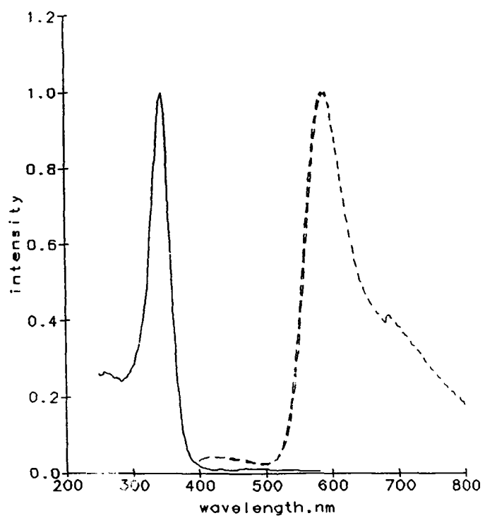
Figure 6. Excitation (solid line) and emission (dotted line) spectra of Zn_{0.93}Mn_{0.07}S prepared in porous sol-gel glass by method 1 in text.
