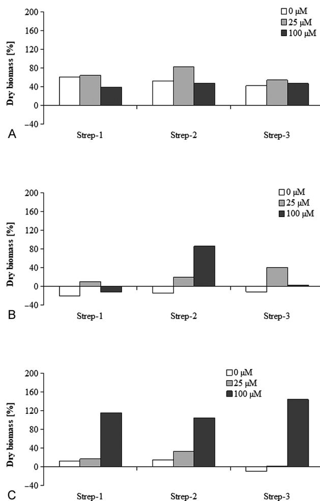
Fig. 1. Dry biomass of leaves (A), shoots (B) and roots (C) of S. viminalis clones inoculated with Streptomyces sp. strains growing at 0 μM, 25 μM and 100 μM Cd 2+ in the culture medium. The results are presented as percentage stimulation or inhibition with respect to their control (100%) representing uninoculated plants (mean ± standard deviation)
