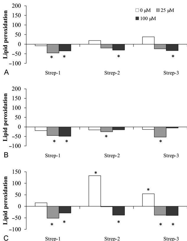
Fig. 2. The level of lipids peroxidation of leaves (A), shoots (B) and roots (C) of S. viminialis clones after Streptomyces sp. strains inoculation growing at 0 \mu\text{M} , 25 \mu\text{M} and 100 \mu\text{M} \text{Cd}^{2+} in the culture medium. The level of lipids peroxidation is represented as the percentage stimulation or inhibition compared to the control (100%) representing uninoculated plants (mean \pm standard deviation) * – significantly different compared to control ( p \leq 0.05 ).
