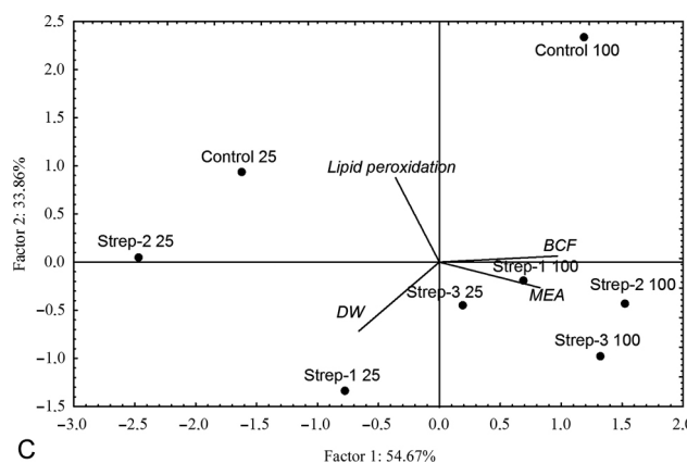
Fig. 4. The Principle Component Analysis (PCA) for the biomass production (DW), phytoextraction efficiency (MEA, BCF, Ti, MER) as well as lipid peroxidation level in the leaves (A), shoots (B) and roots (C) of inoculated and non-inoculated control of S. viminalis clones
