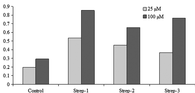
Fig. 3. The accumulation factor (AF) in the S. viminialis above-ground parts (shoots and leaves) of the non-inoculated control and inoculated with (Strep-1–Strep-3) growing in medium supplemented with 25 \mu\text{M} and 100 \mu\text{M} \text{Cd}^{2+} . Different letters indicate significant differences ( p \leq 0.05 ) at 25 \mu\text{M} (lower cases) or 100 \mu\text{M} (upper cases) \text{Cd}^{2+} concentration
