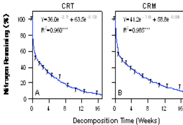
Figure 2. Percent nitrogen remaining from decomposing grass clippings when clippings were returned (A, CRT) or removed (B, CRM). ***Significance of model fit at P < 0.001 .
